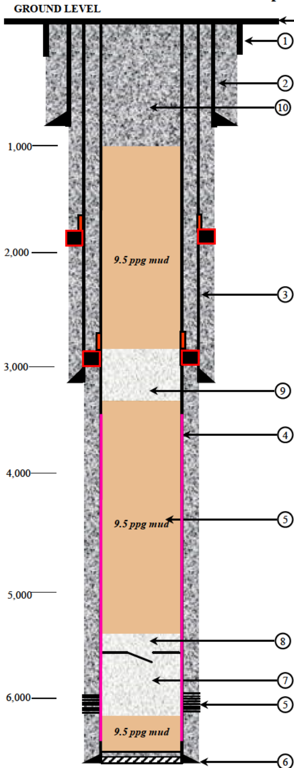
Figure 1: Injection Well 1 (INJ-1) P&A Schematic
