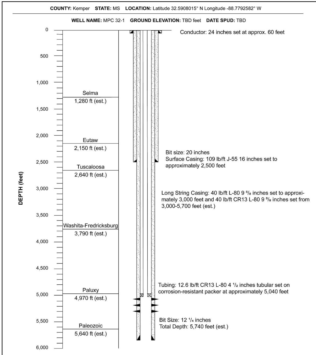
Figure 2. Proposed MPC 32-1 Injection Well Schematic
