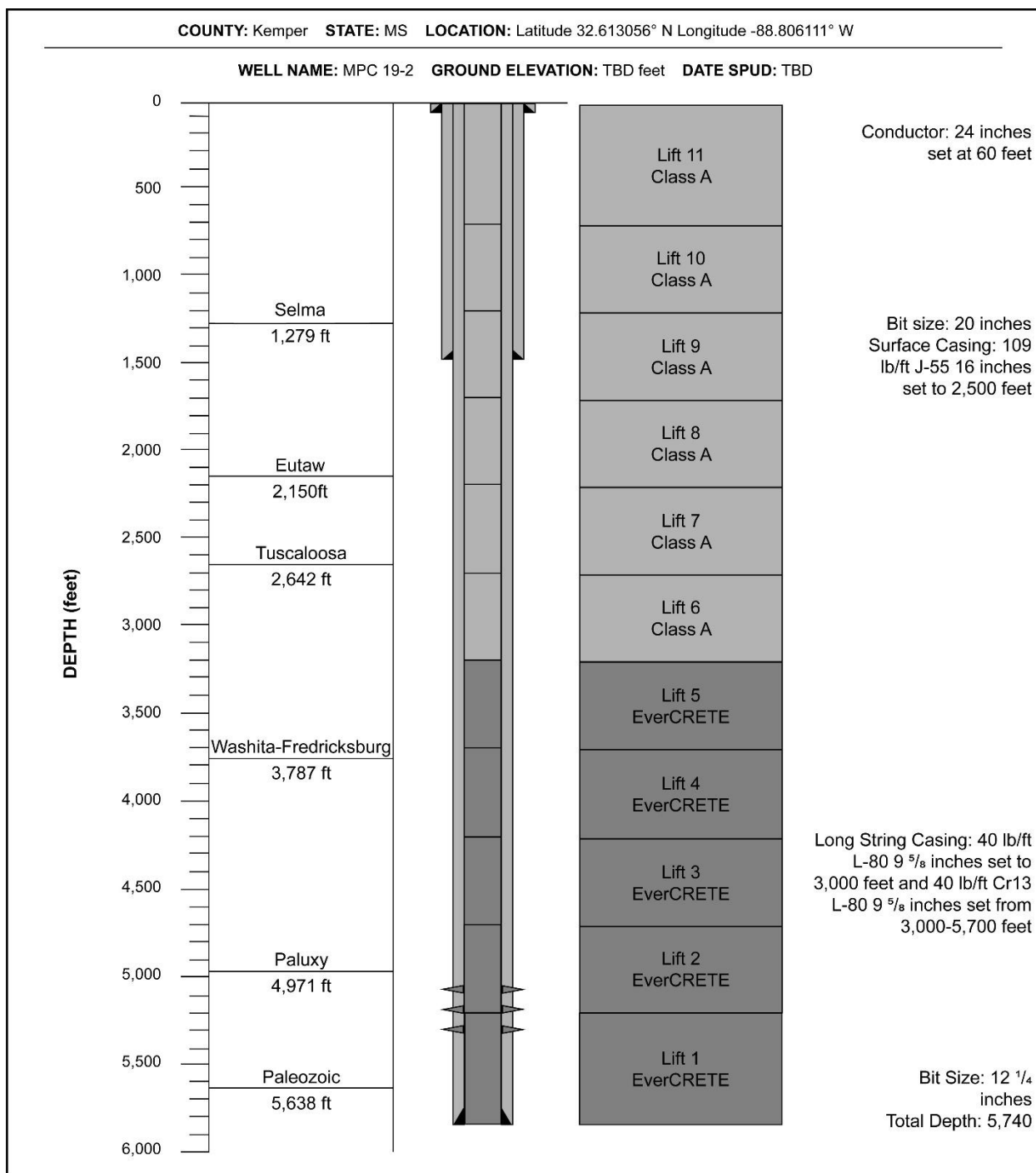
Figure 3. Diagram of MPC 19-2 After Plugging and Abandonment
