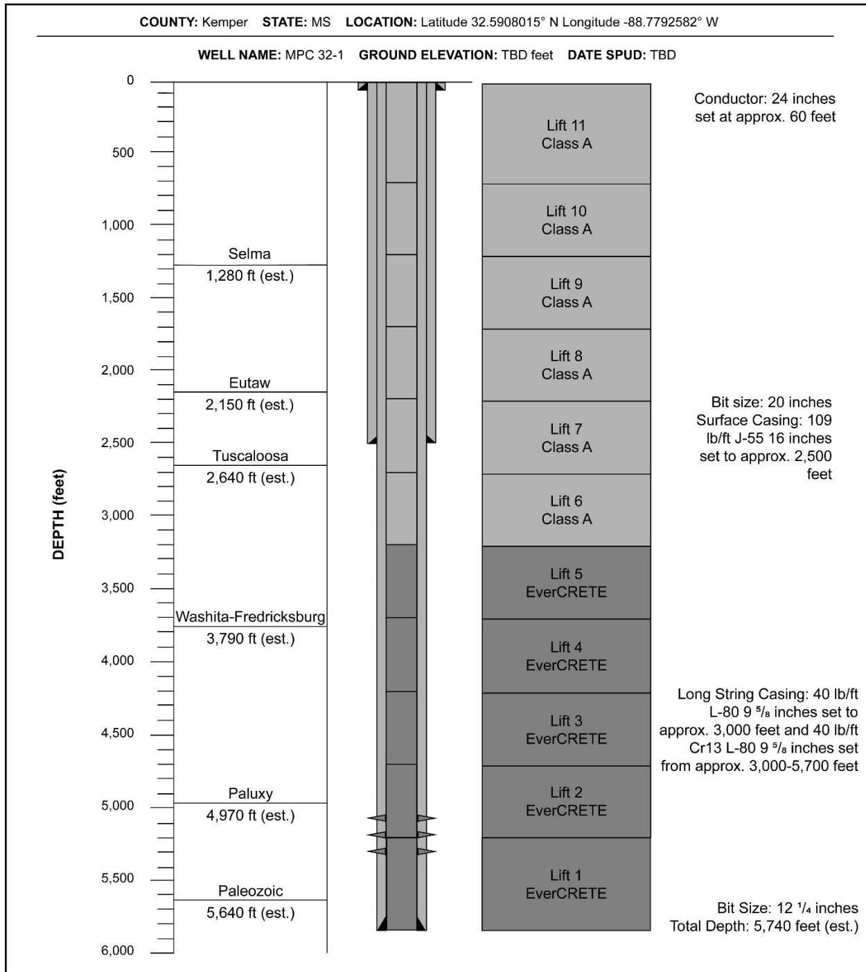
Figure 4. Diagram of MPC 32-1 After Plugging and Abandonment
