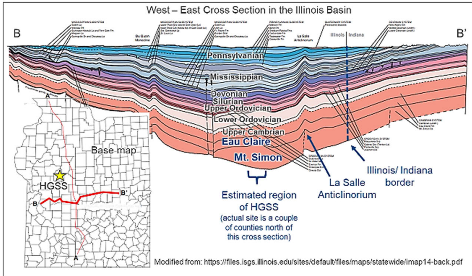
Figure 1-4. Generalized west-east cross section of the Illinois Basin (Modified from ISGS poster titled: Wireline logs and stratigraphic columns West – East Cross Section in the Illinois Basin ).
