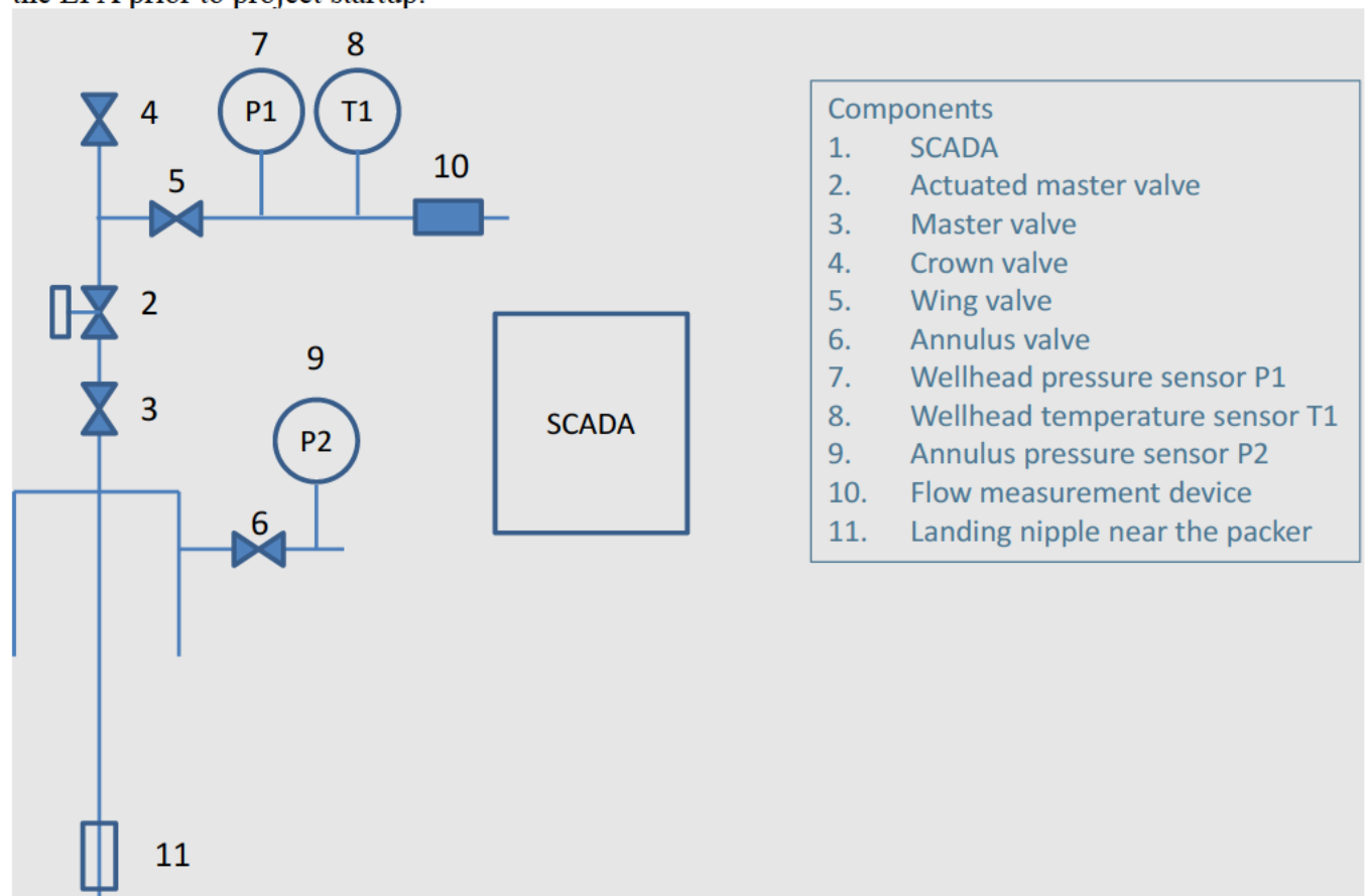
Figure 2: Safety System
