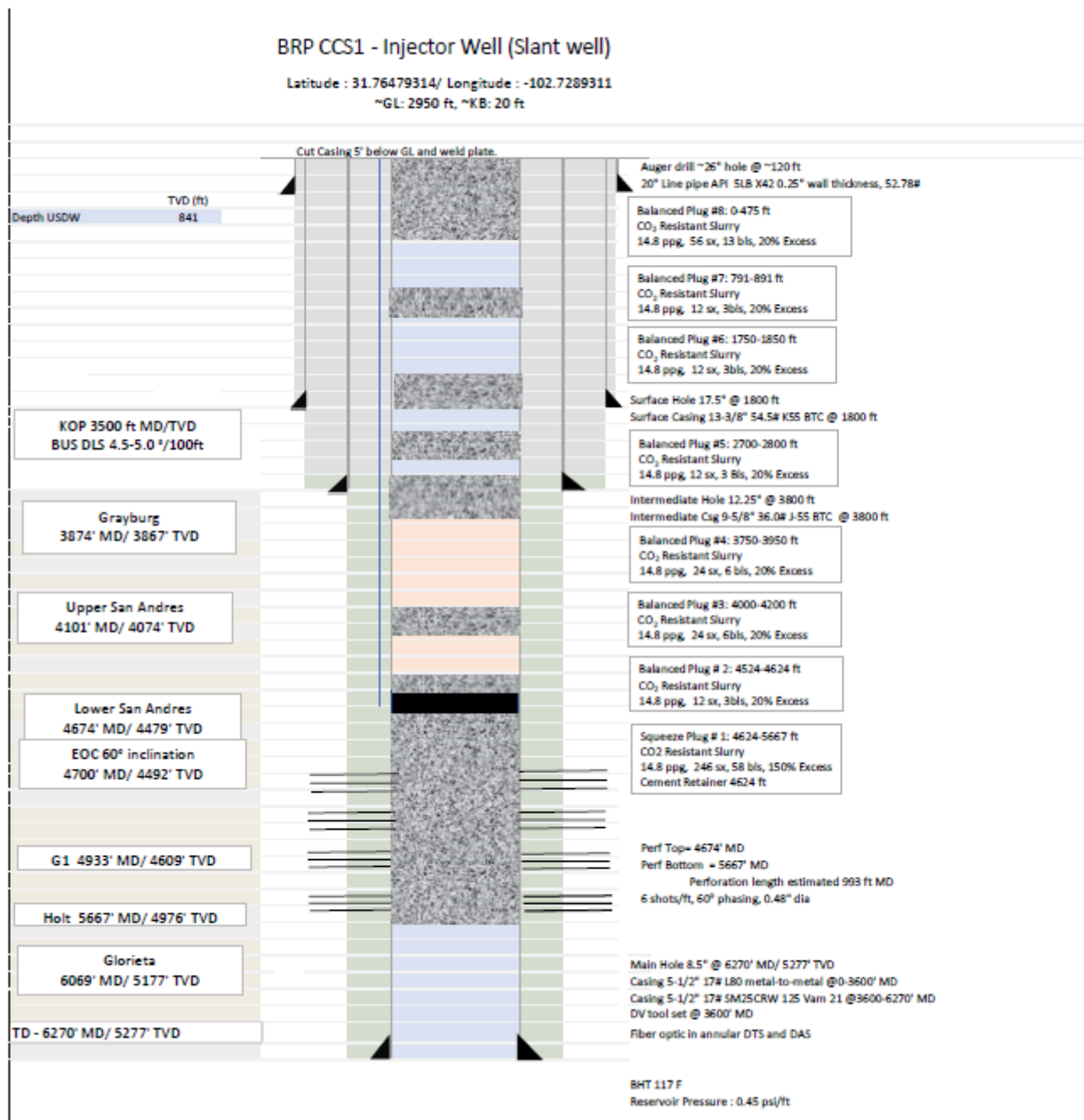
Figure 1—BRP CCS1 well plugging schematic
