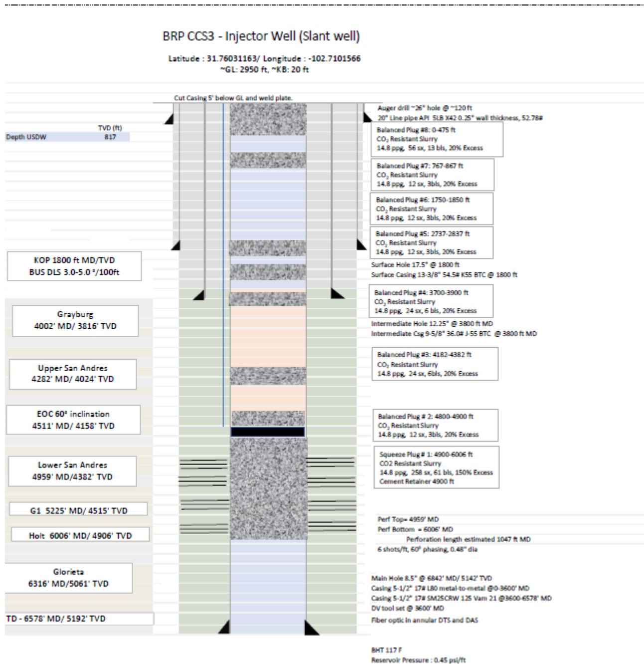
Figure 3—BRP CCS3 well plugging schematic
