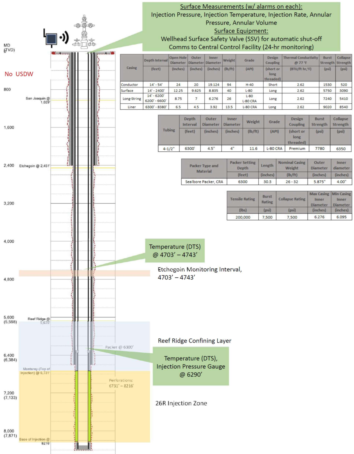
Figure 3: Injection Well 363C-27R, CO 2 Injection Schematic
