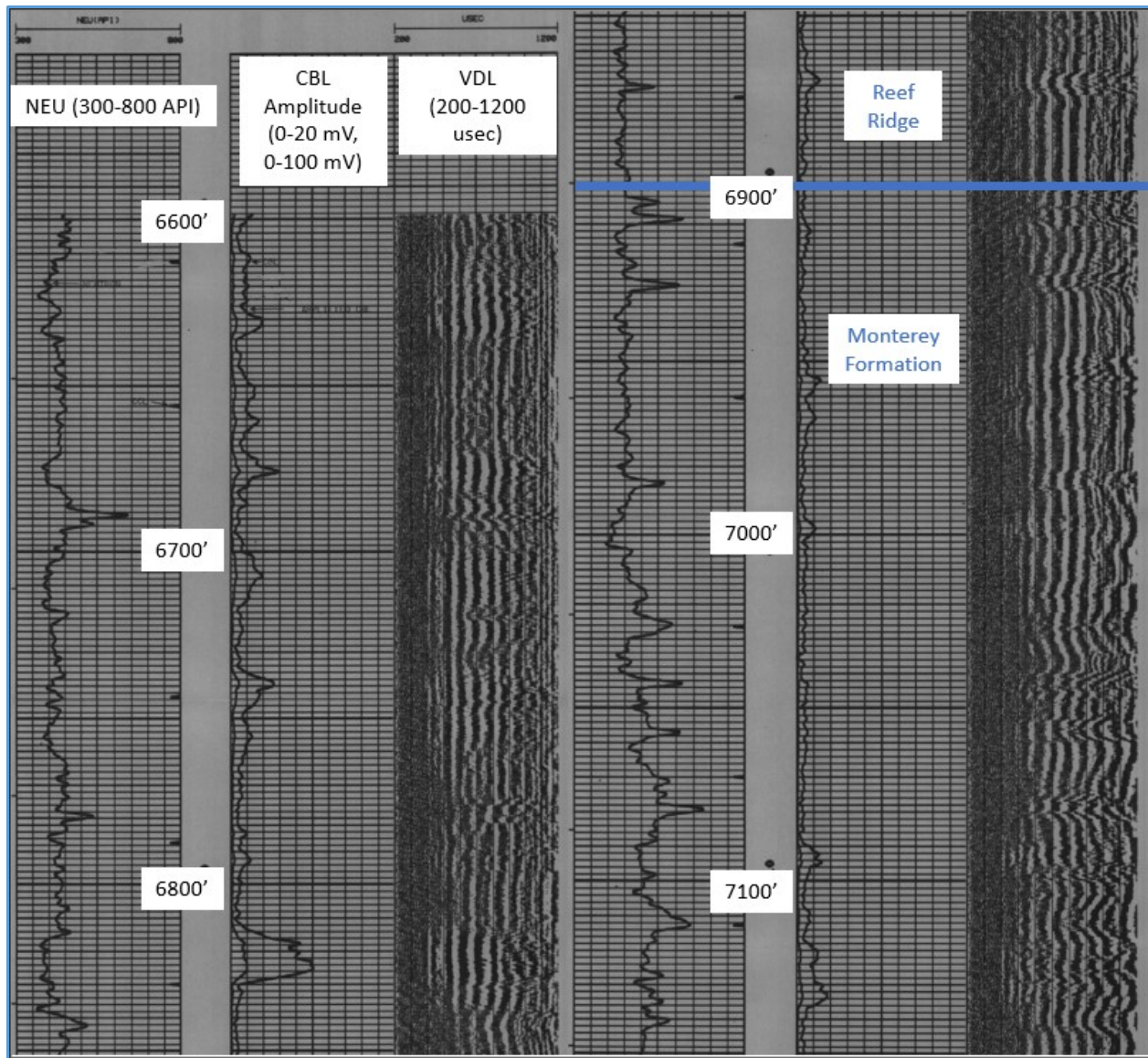
Figure 4: Cement bond log example for 373-35R, after installation of long string casing. The Monterey Formation 26R top is at 6,900 feet.
