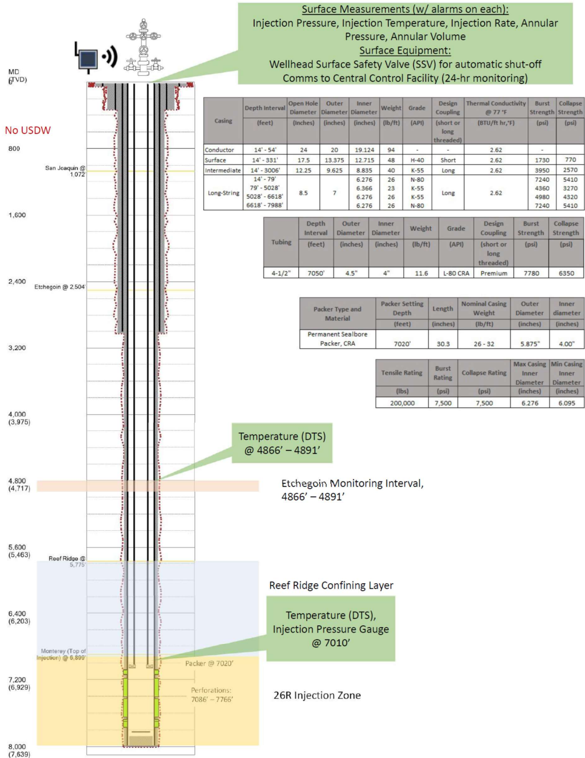
Figure 7: Injection Well 373-35R, CO 2 Injection Schematic
