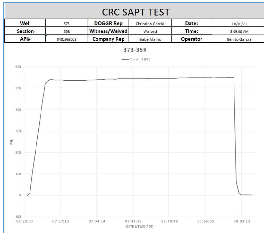
Figure 5: SAPT for 373-35R showing mechanical integrity of the tubing, casing, and packer.
