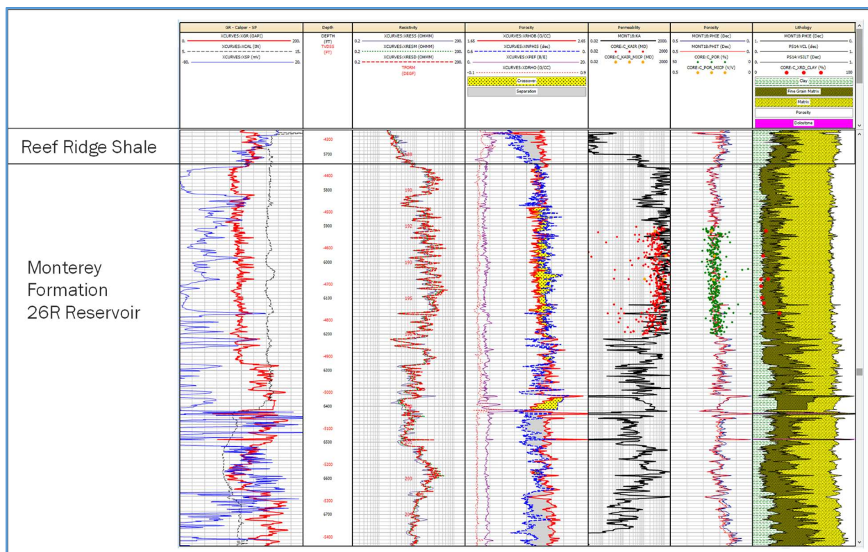
Figure 3: Open-hole well logs for 373-35R before installation of long string.
