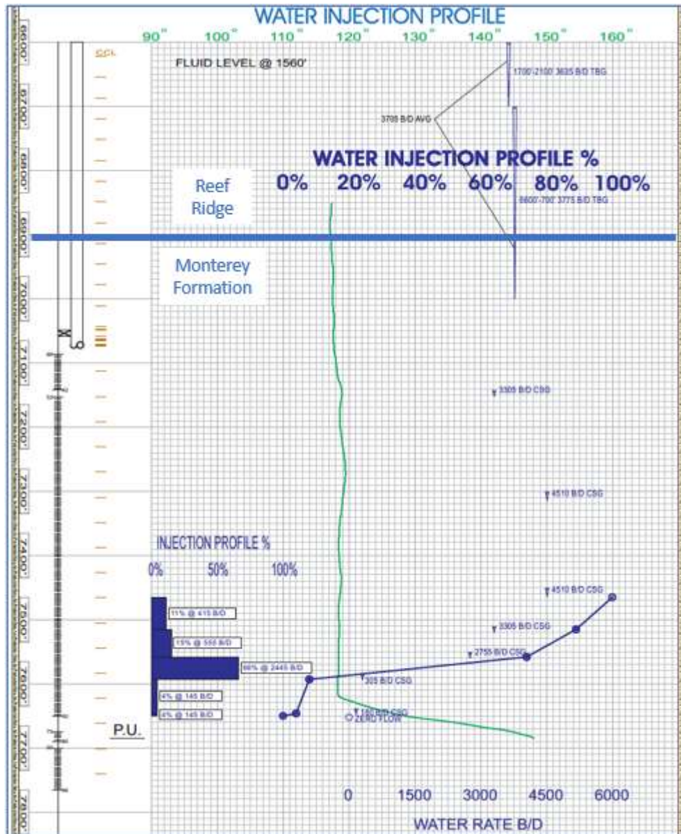
Figure 6: Radioactive tracer and temperature survey for well 373-35R showing mechanical integrity of the tubing and isolation of the perforation by the packer.
