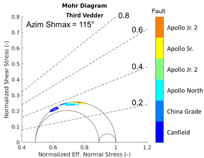
Figure 79. Fault stability results for faults near well KC20050X_ST1 for Vd3. A single stress azimuth of 115° was considered for this analysis. Stresses are normalized with respect to effective vertical stress.
