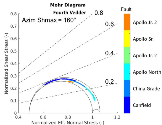
Figure 80. Fault stability results for faults near well KC20050X_ST1 for Vd4. A single stress azimuth of 160° was considered for this analysis. Stresses are normalized with respect to effective vertical stress.
