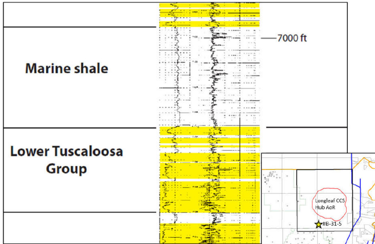
Figure 30. Type log for the Tuscaloosa Marine Shale in the Longleaf CCS Hub from well #B-31-5.
