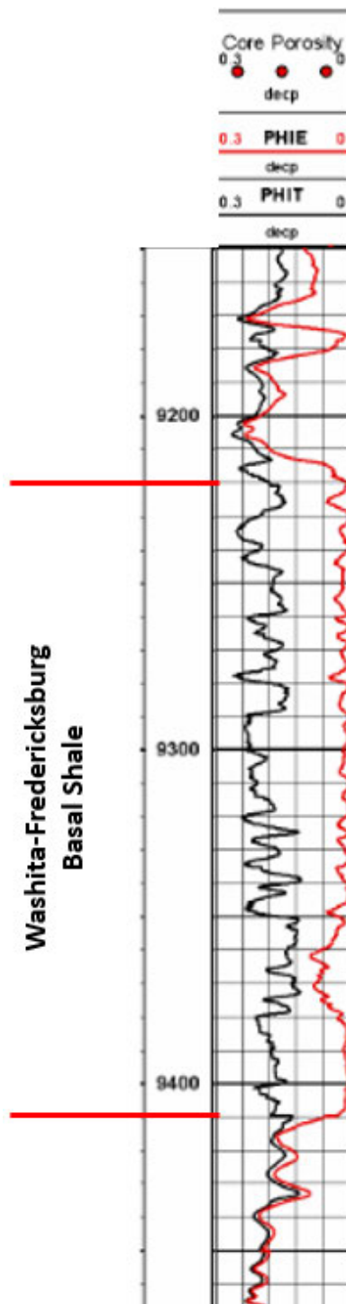
Figure 35. Porosity log from the D-9-7 #2 well over the Washita-Fredericksburg basal shale showing the total porosity (PHIT) in black and effective porosity (PHIE) in red.
