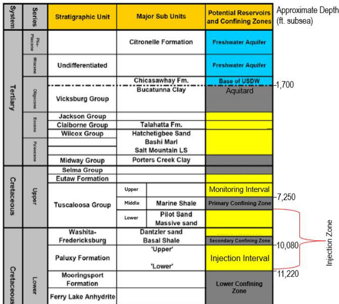
Figure 2: Geologic Stratigraphic Column at the Lingleaf CCS Hub (modified from Pashin et al., 2008). 1
