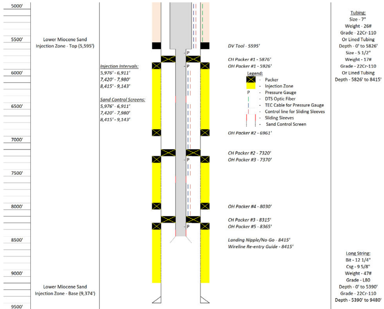
Figure 10: Proposed well schematic for LO-05 M (5,000 to 9,480 ft).
