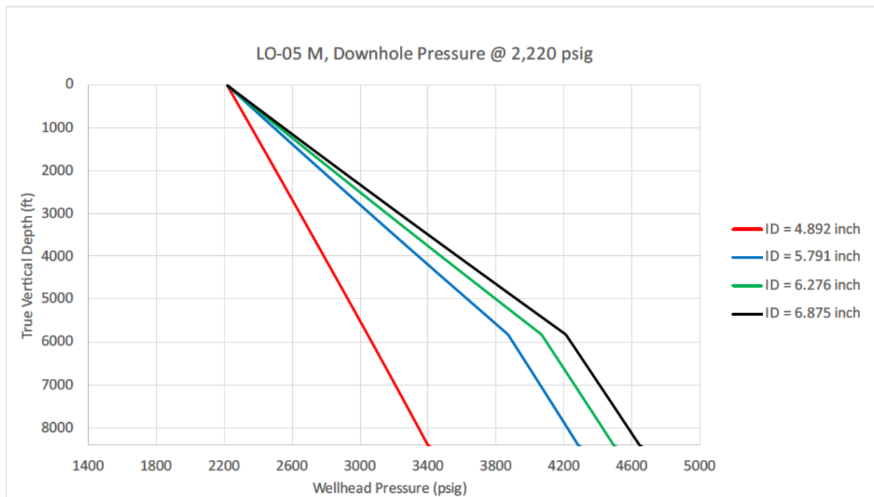
Figure 1: LO-05 M downhole pressure at maximum injection rate (3.5 MMt/y) and maximum injection pressure (2,220 psig) using different tubing sizes for CO 2 injection into the LMIC.
