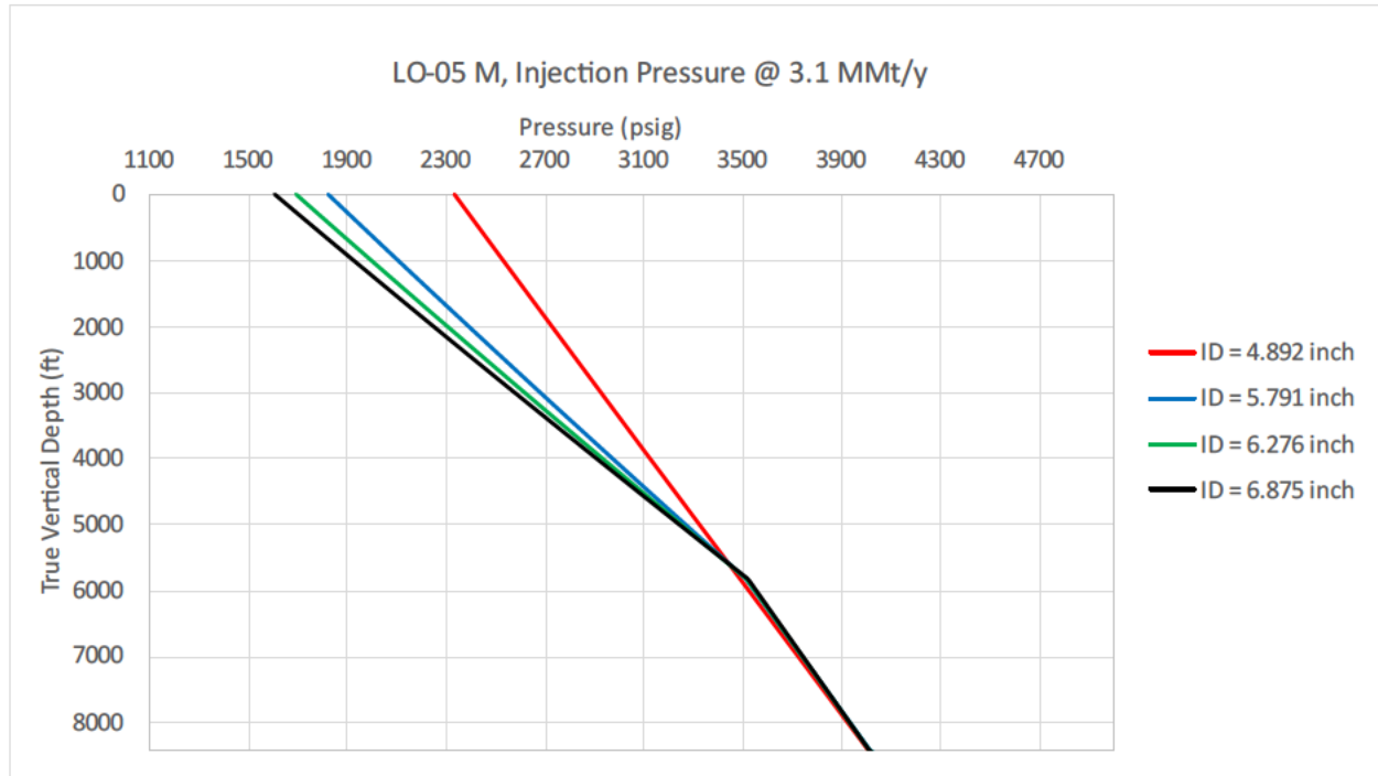
Figure 2: LO-05 M injection pressure at average injection rate of 3.1 MMt/y using different tubing sizes for CO 2 injection into the LMIC.
