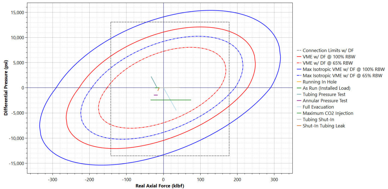
Figure 10: 3.5-inch tubing (22Cr-110) axial force design envelope with 100% and 65% remaining body wall.
