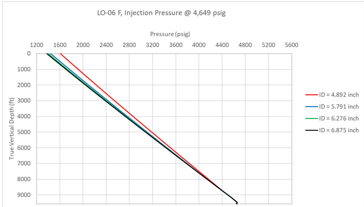
Figure 2: LO-06 F injection pressure at maximum injection rate (1.5 MMt/y) and average reservoir pressure (4,649 psig) using different tubing sizes for CO 2 injection into the OFIC.
