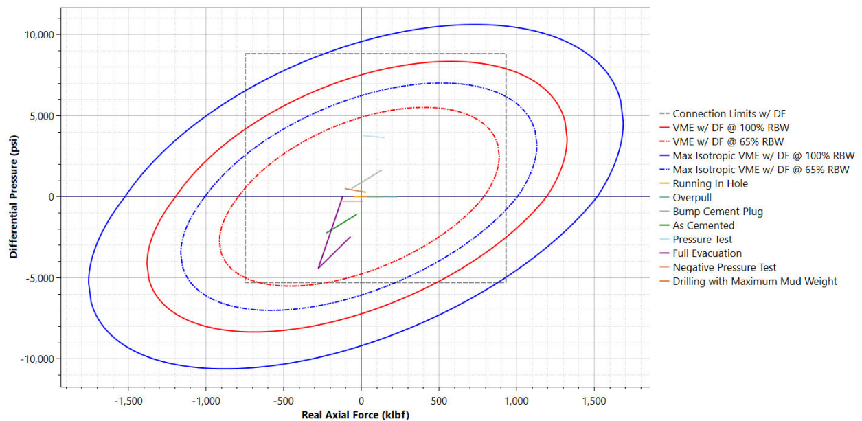
Figure 6: 9.625-inch long-string casing (22Cr-110) axial force design envelope with 100% and 65% remaining body wall.
