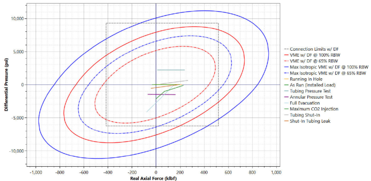
Figure 8: 7-inch tubing (22Cr-110) axial force design envelope with 100% and 65% remaining body wall.
