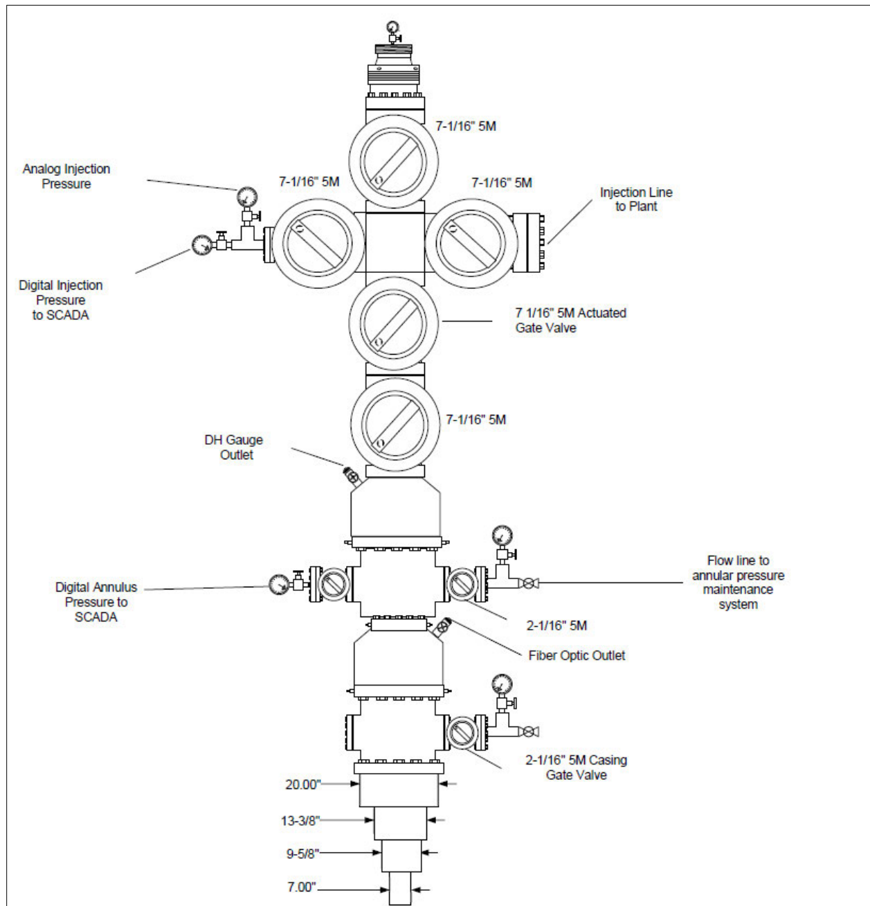
Figure 11: Proposed wellhead and christmas tree schematic for LO-06 F.
