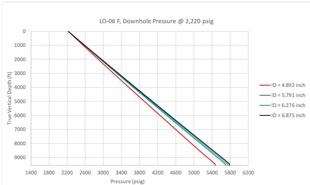
Figure 1: LO-06 F downhole pressure at maximum injection rate (1.5 MMt/y) and maximum injection pressure (2,220 psig) using different tubing sizes for CO 2 injection into the OFIC.
