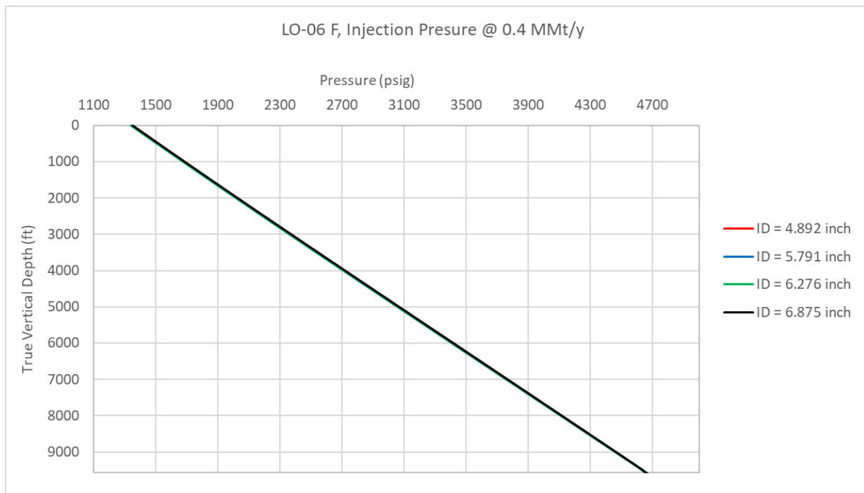
Figure 3: LO-06 F injection pressure at average injection rate of 0.4 MMt/y using different tubing sizes for CO 2 injection into the OFIC. The pressure profiles are almost identical for the tubing designs.
