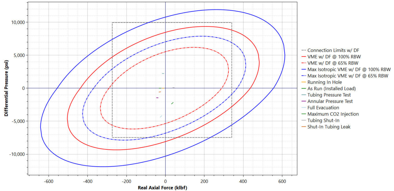
Figure 9: 5.5-inch tubing (22Cr-110) axial force design envelope with 100% and 65% remaining body wall.
