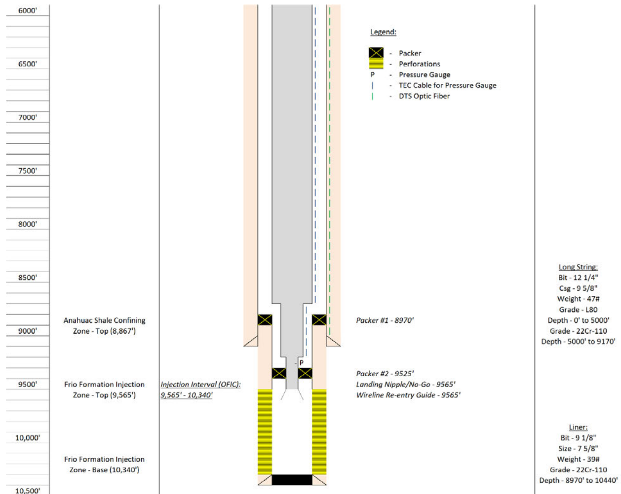
Figure 13: Proposed well schematic for LO-06 F (6,000 ft – 10,440 ft TVD).
