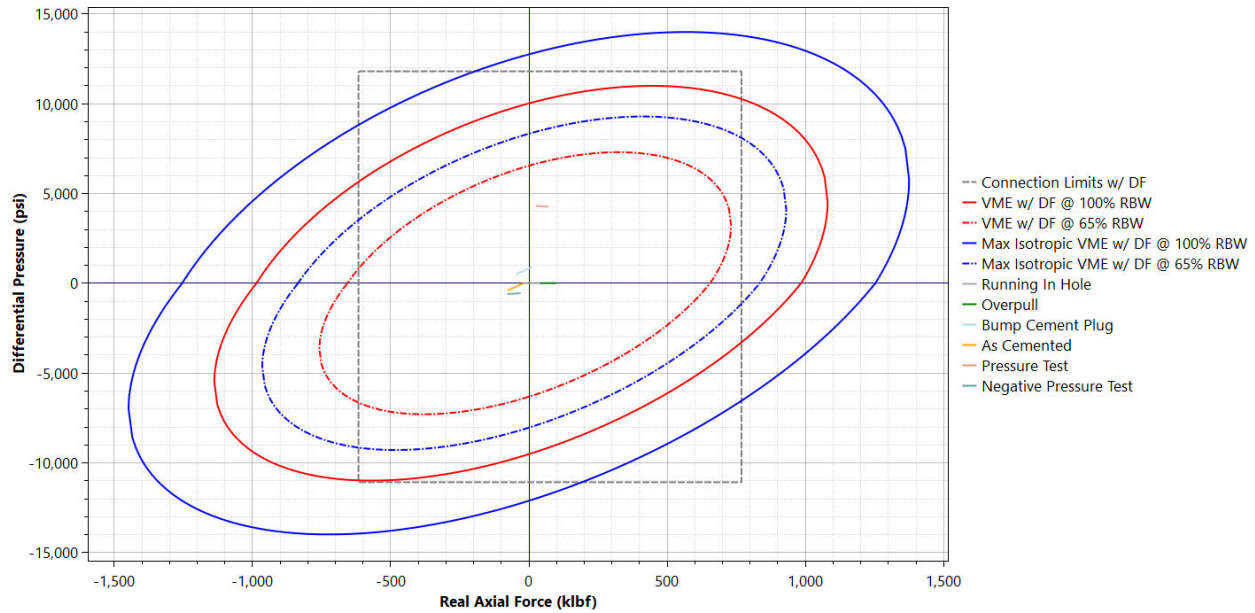
Figure 7: 7.625-inch liner (22Cr-110) axial force design envelope with 100% and 65% remaining body wall.
