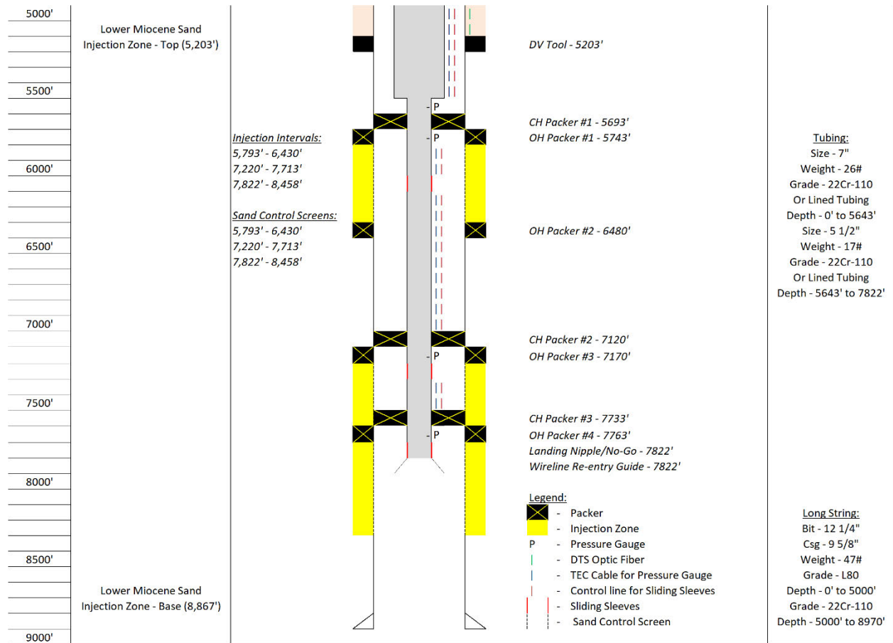
Figure 10: Proposed well schematic for LO-06 M (Zoomed 5,500 to 8,970 ft).
