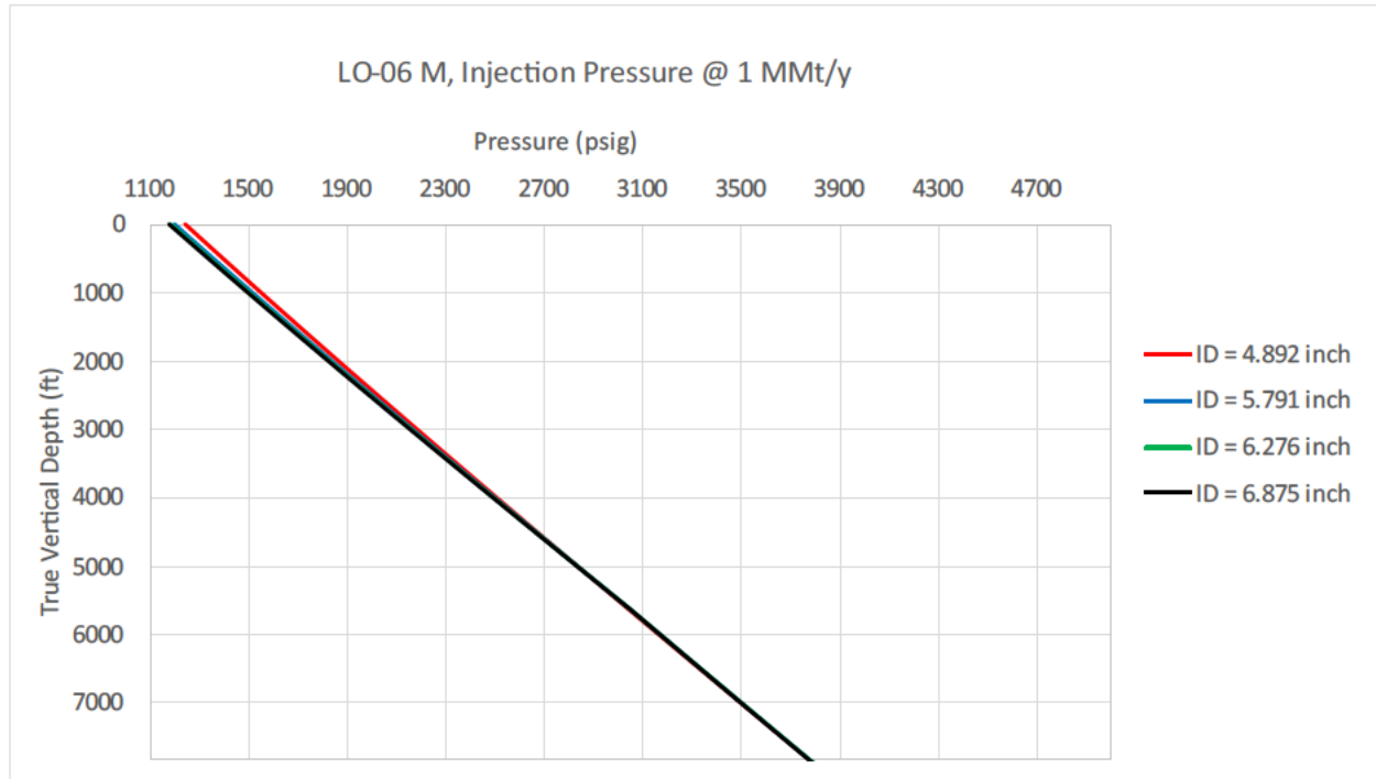
Figure 2: LO-06 M injection pressure at average injection rate of 1.0 MMt/y using different tubing sizes for CO 2 injection into the LMIC.
