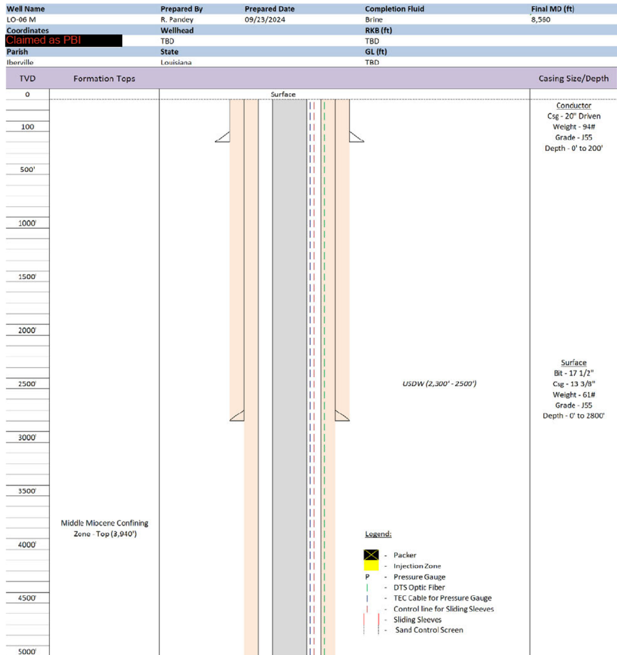
Figure 9: Proposed well schematic for LO-06 M (0 ft to 5,000 ft).
