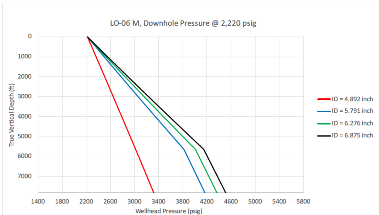
Figure 1: LO-06 M downhole pressure at maximum injection rate (3.5 MMt/y) and maximum injection pressure (2,220 psig) using different tubing sizes for CO 2 injection into the LMIC.
