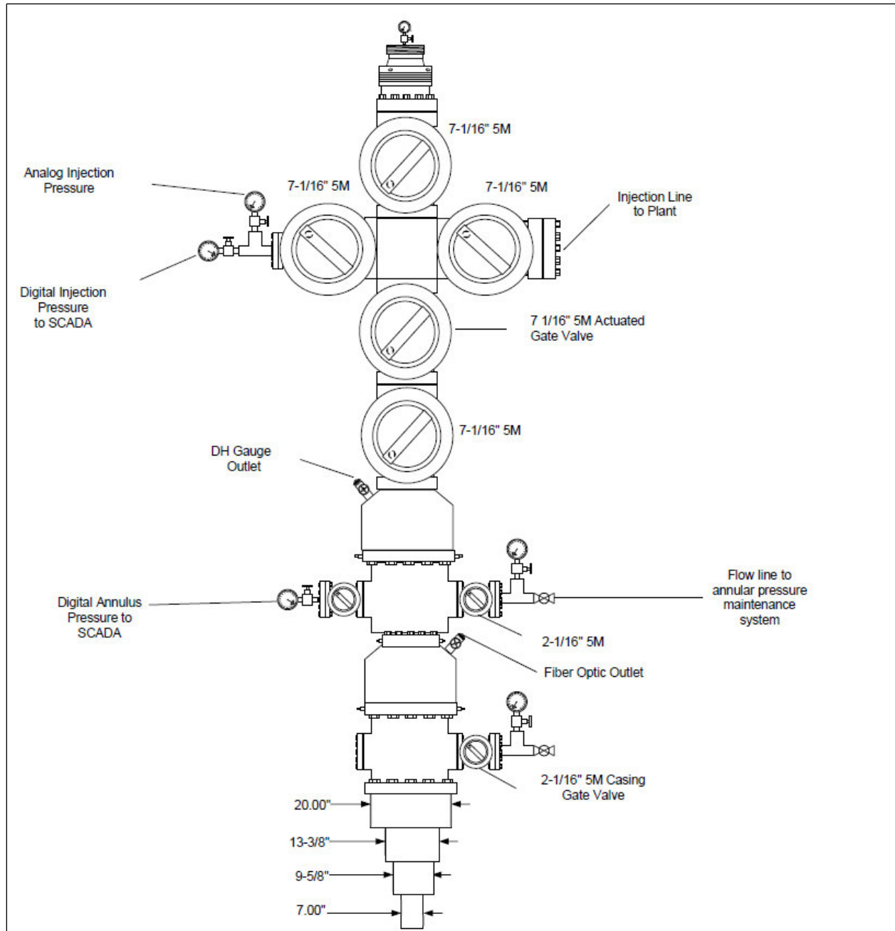
Figure 8: Proposed wellhead and christmas tree schematic for LO-06 M.
