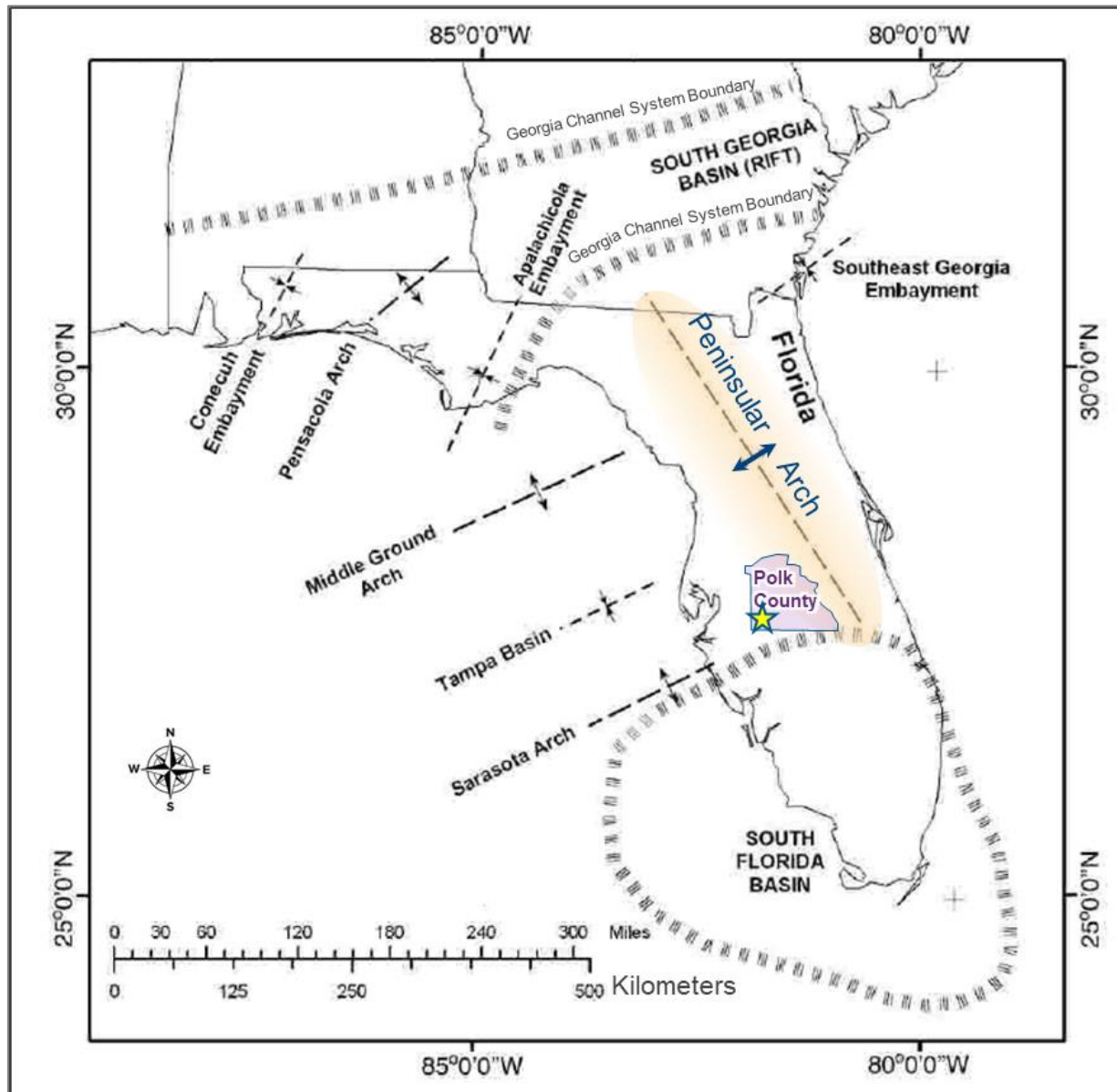
Figure 1-2. Map showing the locations of major geologic structures and basins across the state of Florida. Yellow star is the location of TEC's Polk Power Station. Map modified from Lloyd (1991). 4
