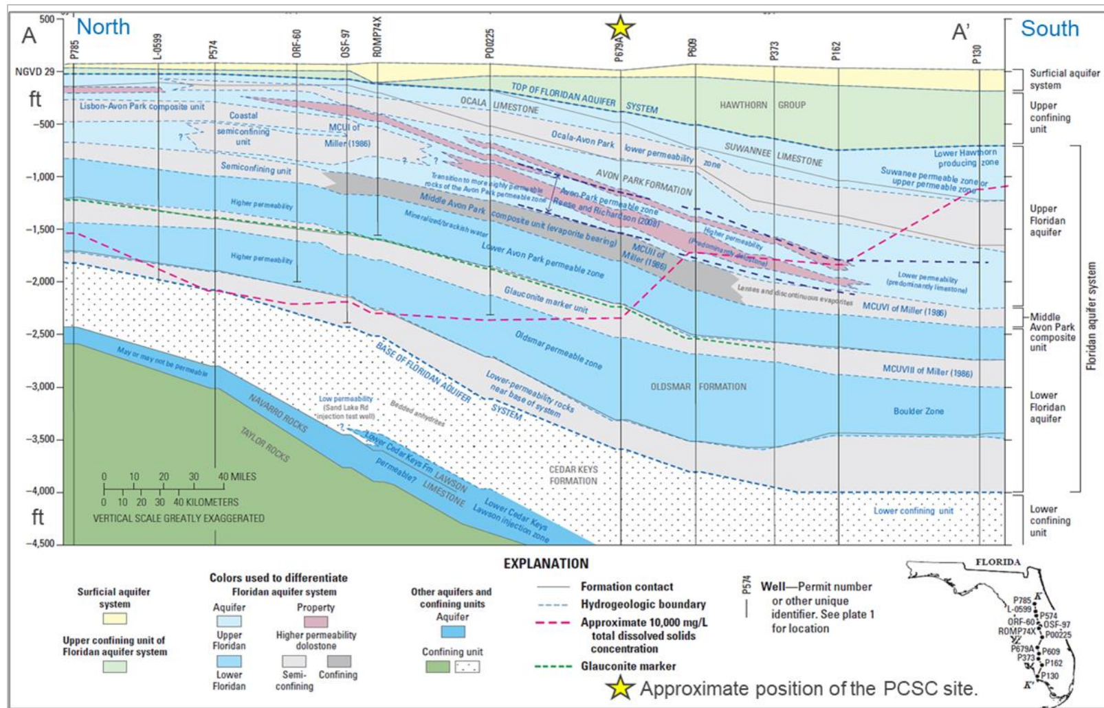
Figure 1-21. Cross section depicting the hydrological units in Florida (image taken from Williams et al., 2015). 30
