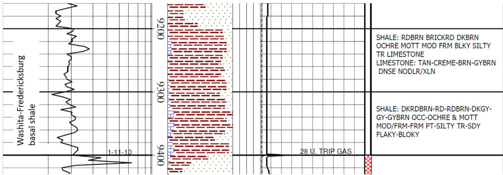
Figure 34. Mud log with lithology descriptions from the basal shale of the Washita Fredericksburg interval.
