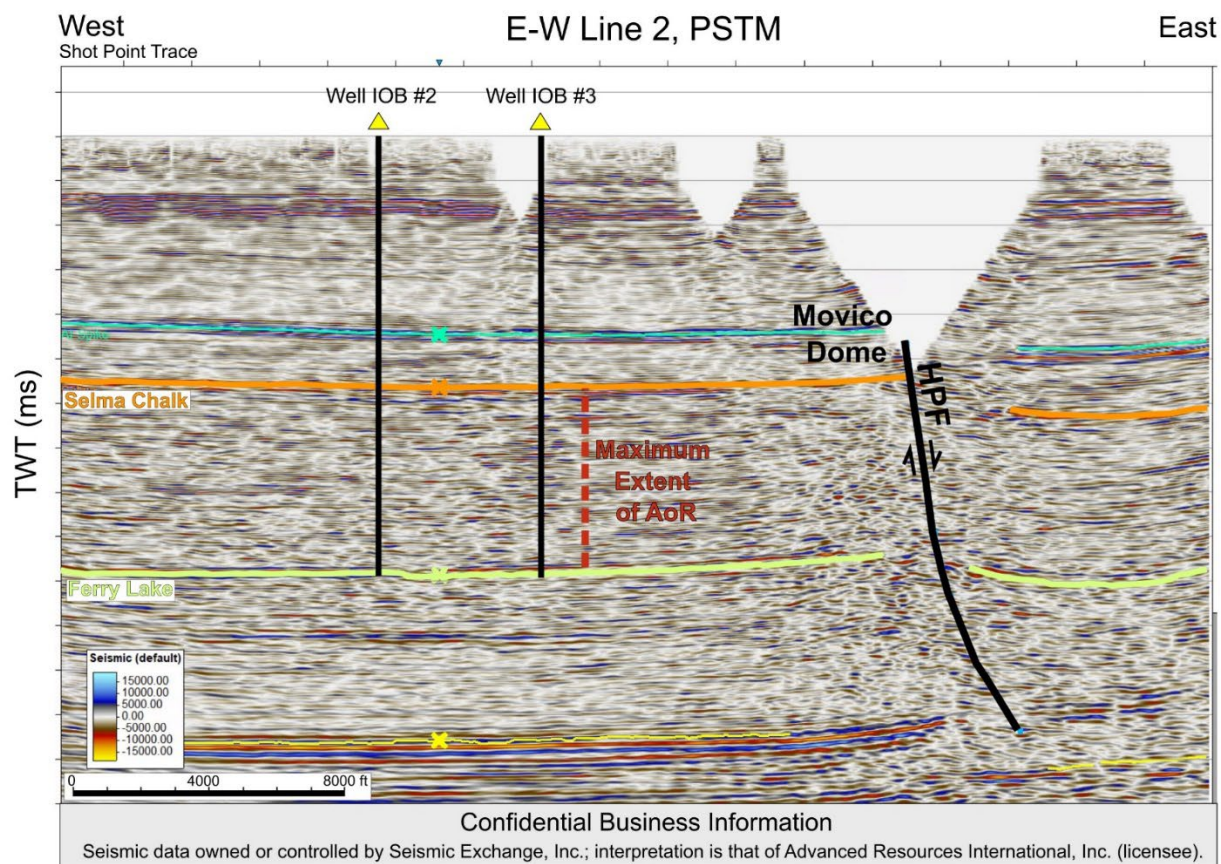
Figure 11. Interpreted Post Stack Time Migrated (PTSM) west-east 2D seismic line that intersects the AoR and HPF along the western edge of the Mobile Graben. The structural high point of Movico Dome is also indicated adjacent to the HPF along the footwall of the fault. The locations of in-zone monitoring wells IOB#2 and IOB#3 were projected onto the 2D seismic line. The Selma Chalk and Ferry Lake Anhydrite are also interpreted on the seismic image.
