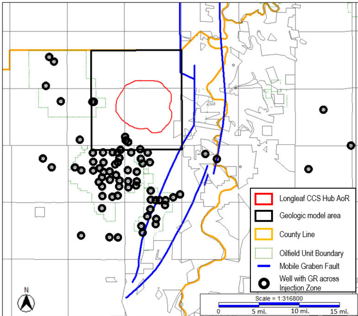
Figure 7. Wells with gamma ray logs across the Paluxy Formation and Tuscaloosa Marine Shale used in regional geologic study, including the 3 DOE/NETL SECARB Phase III Anthropogenic CO 2 injection test wells and 80 existing deep exploration wells.
