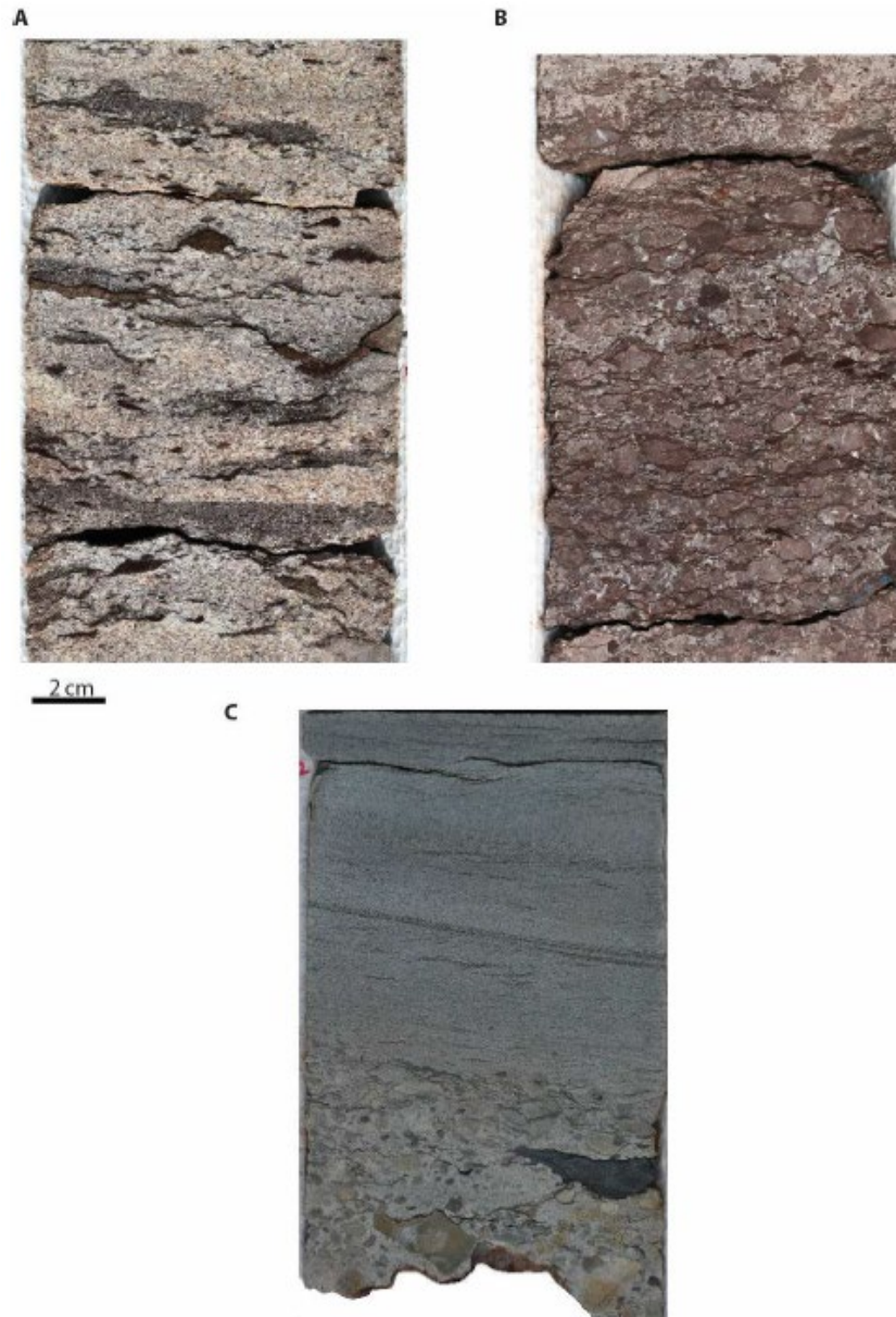
Figure 17. Core photos of the Paluxy conglomerate facies.
