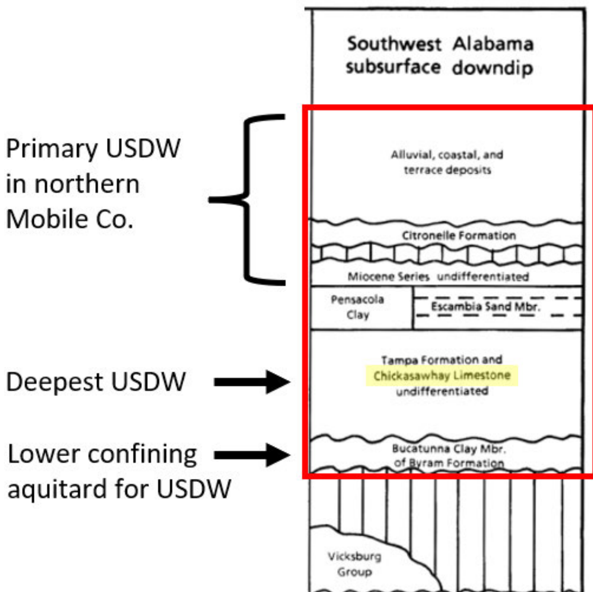
Figure 43. Stratigraphic column of USDW and the confining aquitard protecting USDW in southwest Alabama (modified from Raymond et al., 1988).
