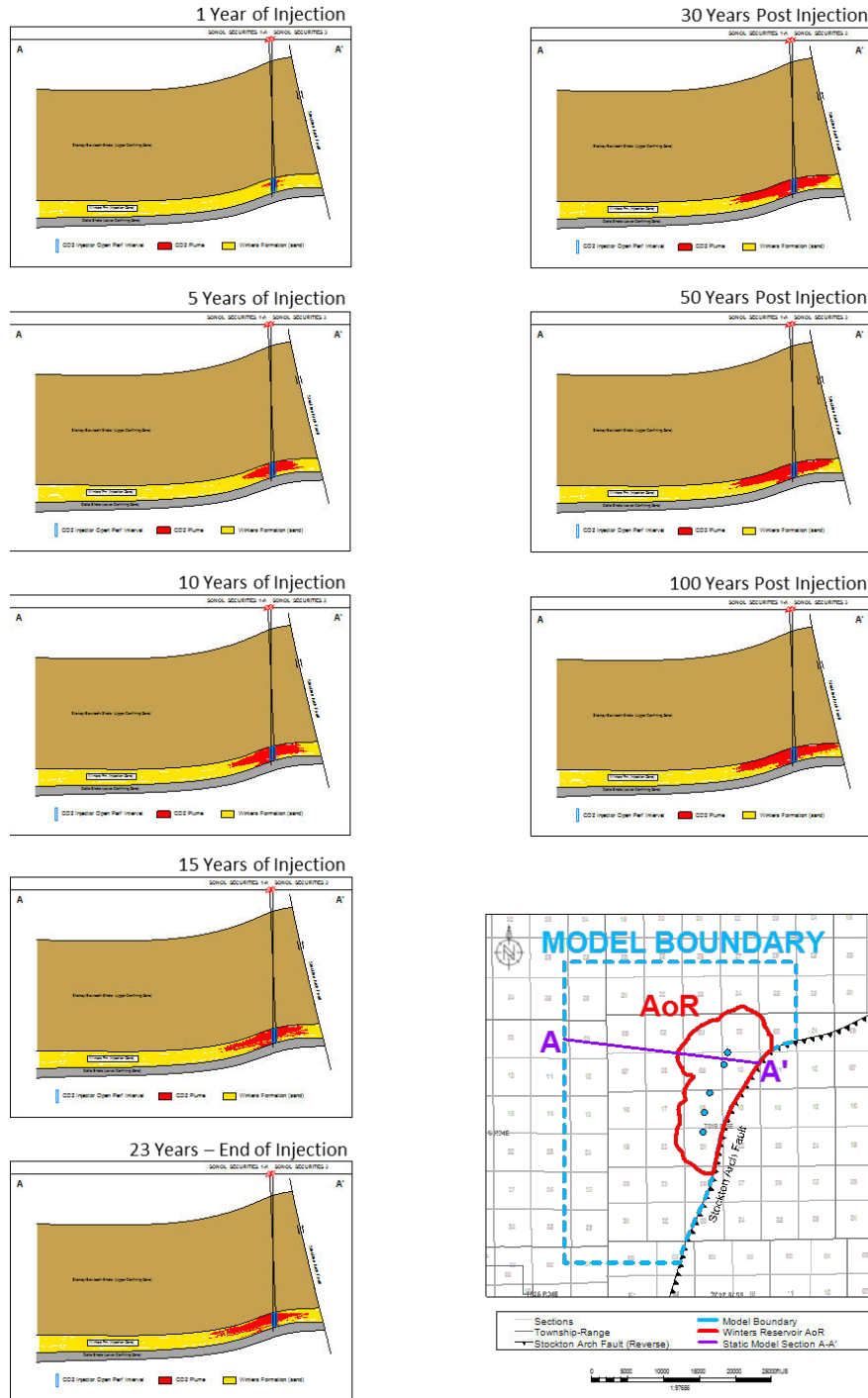
Figure A-58b. Section showing proximity of CO 2 (Injectate 2) to the Stockton Arch Fault and lateral dispersion of CO 2 throughout time and confinement under the overlying Starkey-Sawtooth through time for the five injector modeled Base scenario. As the sections show, plume growth over time is driven by the reservoir anticlinal structure, and is thus representative of the plume growth at all injector locations.
