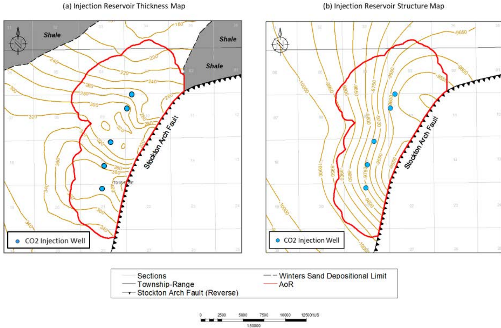
Figure A-14. (a) Injection reservoir thickness map (b) Injection reservoir structure map. AoR in red.
