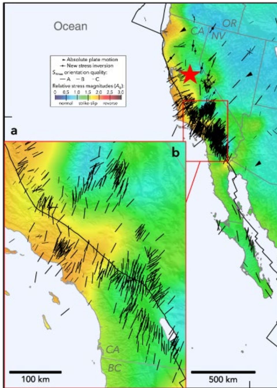
Figure A-42. Image modified from Lund Snee and Zoback (2020) showing relative stress magnitudes across California. Red star indicates CTV II project site area.
