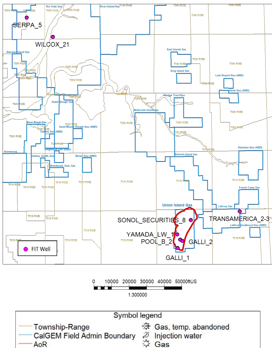
Figure A-37. Locations of wells with FIT data.
