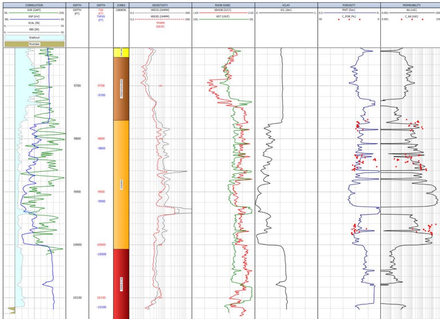
Figure A-30. Log plot for well Sonol_Securities_6, showing the log curves used as inputs into calculations of clay volume, porosity and permeability, and their outputs. Core data for porosity and permeability is shown for comparison to the log model. Track 1: Correlation and caliper logs. Track 2: Measured depth. Track 3: Vertical depth and vertical subsea depth. Track 4: Zones. Track 5: Resistivity. Track 6: Compressional sonic and density logs. Track 7: Volume of clay. Track 8: Porosity calculated from log curves and core porosity. Track 9: Permeability calculated using transform and core permeability.
