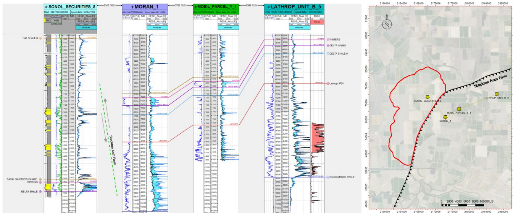
Figure A-24. Well Section across the Stockton Arch Fault.
