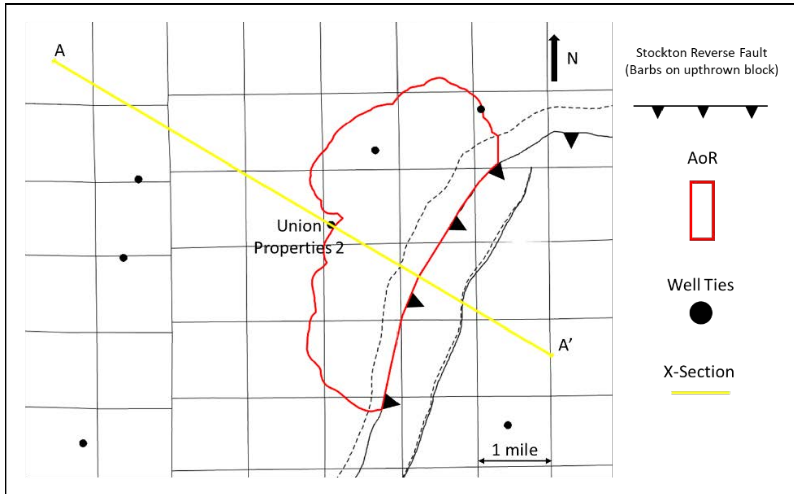
Figure A-19. The two faults within the model are shown at the Winters level. The fault to the east is believed to be antithetic to the main Stockton Arch fault and is dashed into it in cross-section. Yellow line highlights the cross section shown in Figure A-20.
