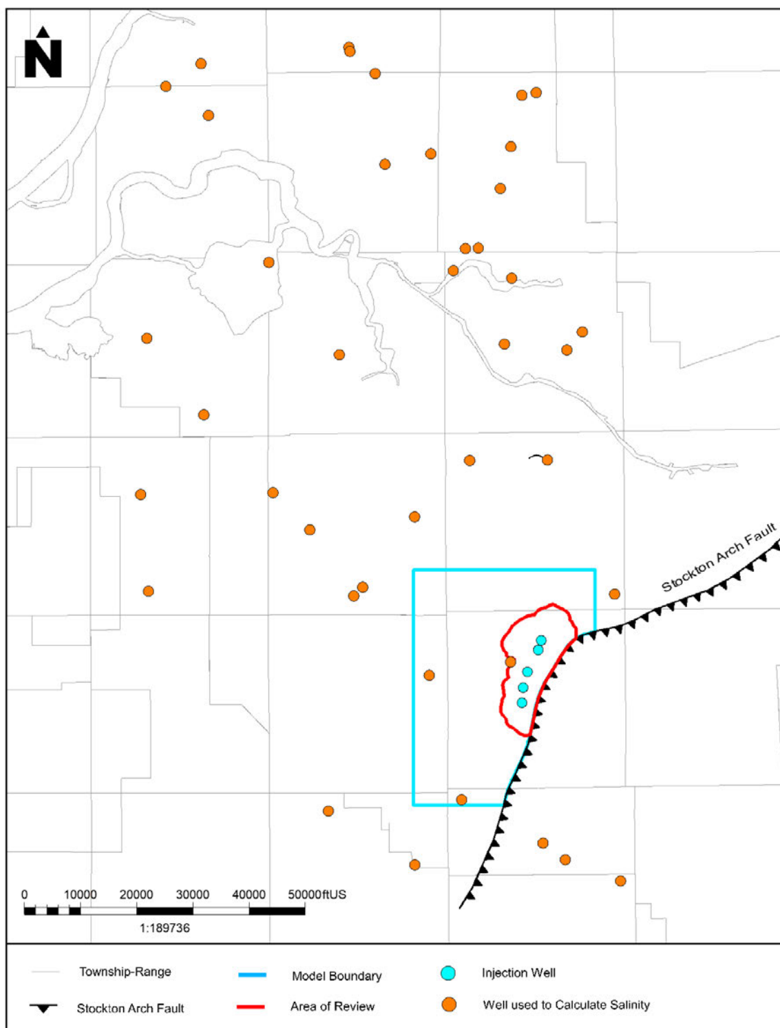
Figure A-45. Wells used in salinity calculations.
