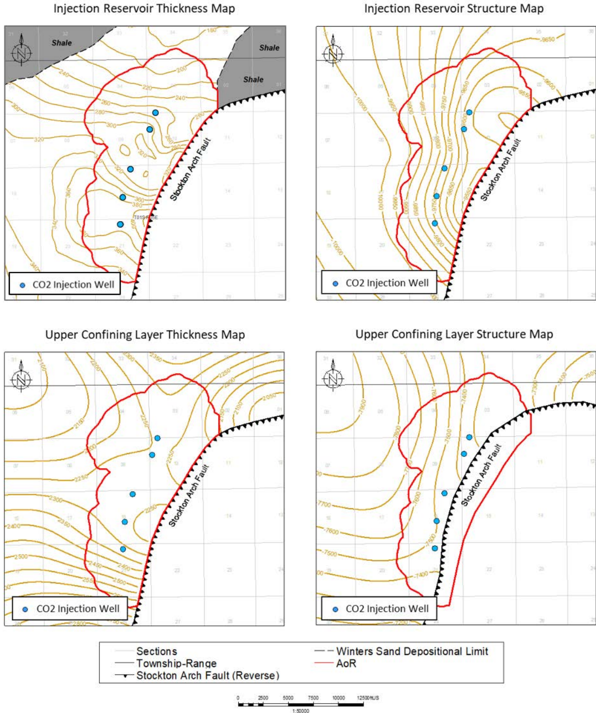
Figure A-33. Gross thickness and depth maps within the AoR for the injection reservoir and upper confining layer. The Stockton Arch Fault dips to the southeast, therefore the surface of the upper confining layer intersects the fault within the AoR boundary.
