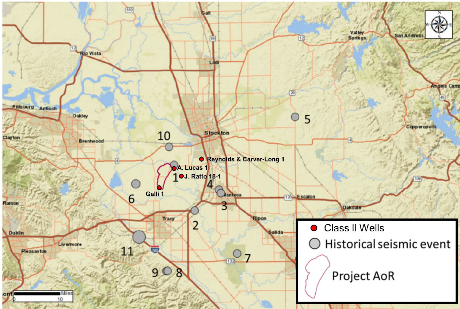
Figure A-41. Historical seismic events and Class II wells near the Area of Review. This image has been modified from USGS search results. Data from these events are compiled in Table A-11 in chronological order associated with events 1 through 11 on the map. Data associated with the Class II wells is compiled in Table A.12.
