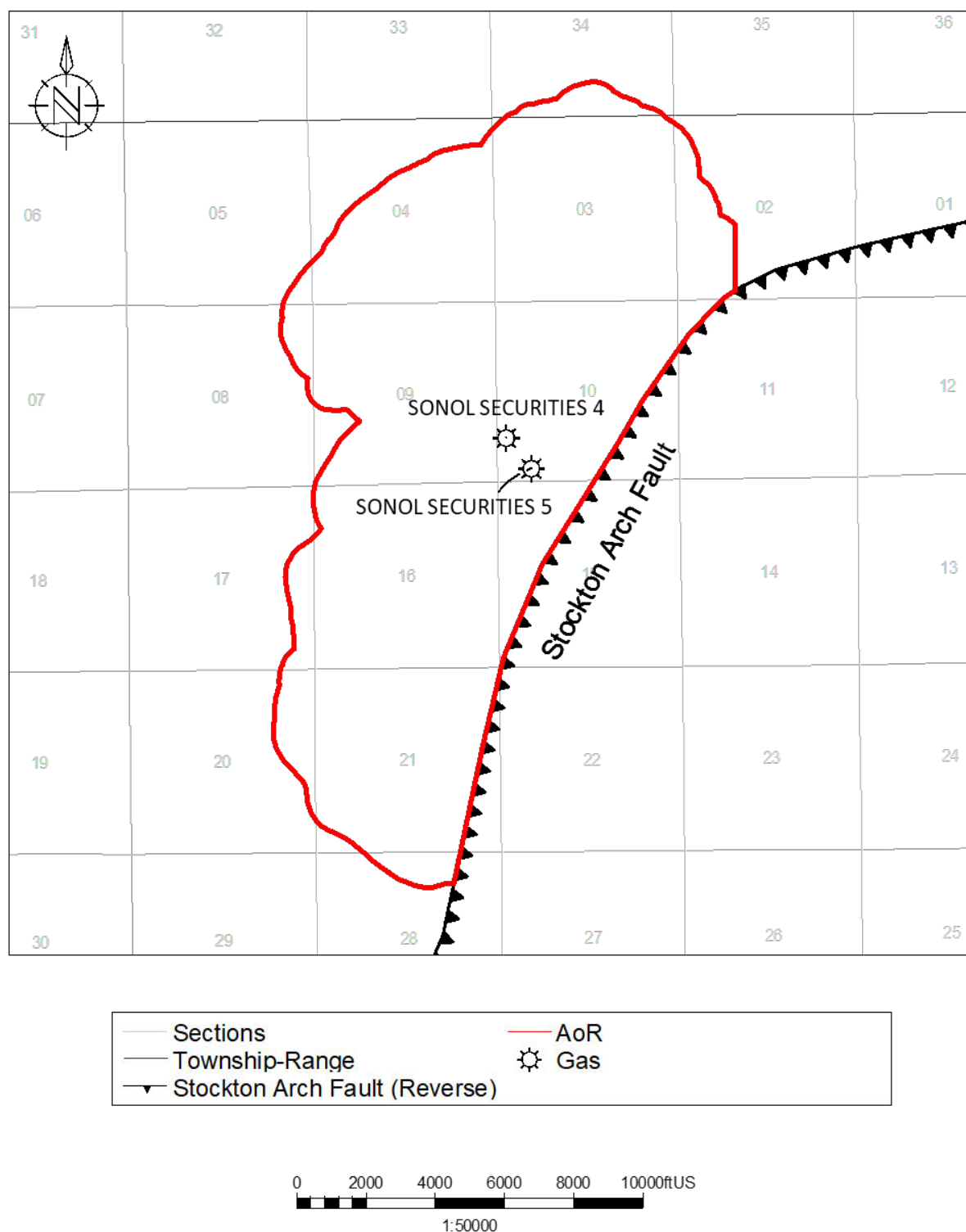
Figure A-57. Locations of wells with geochemistry data.
