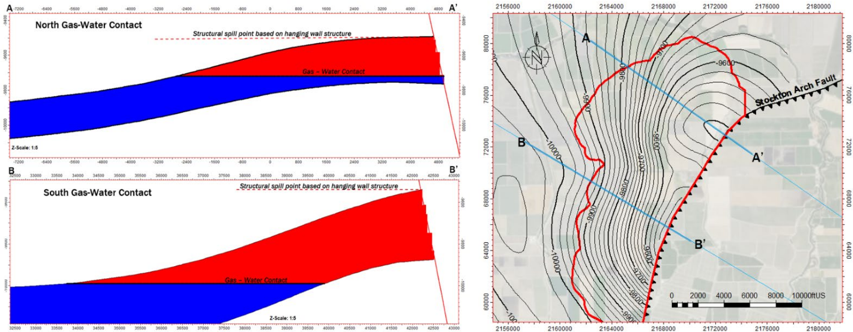
Figure A-23. Gas-water contacts and structural spill points.
