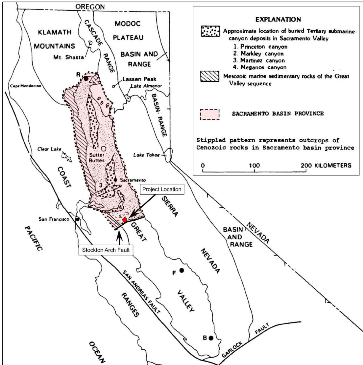
Figure A-2. Location map of California modified from (Beyer, 1988) & (Sullivan, 2012). The Sacramento Basin regional study area is outlined by a dashed black line. B – Bakersfield; F – Fresno; R – Redding.
