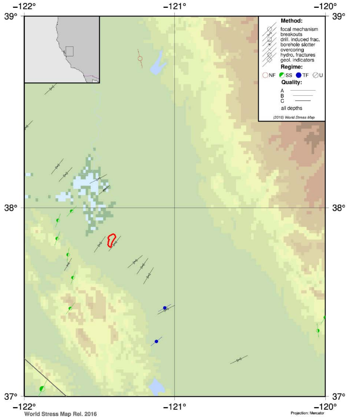
Figure A-36. World stress map output showing SHmax azimuth indicators and earthquake faulting styles in the Sacramento Basin (Heidbach et al., 2016). The red polygon is the project AoR. The background coloring represents topography.
