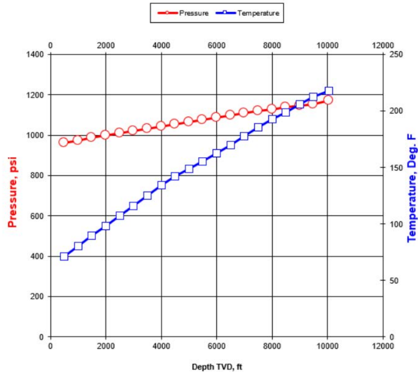
Figure A-21. POOL B-2 Pressure and Temperature Gradient
