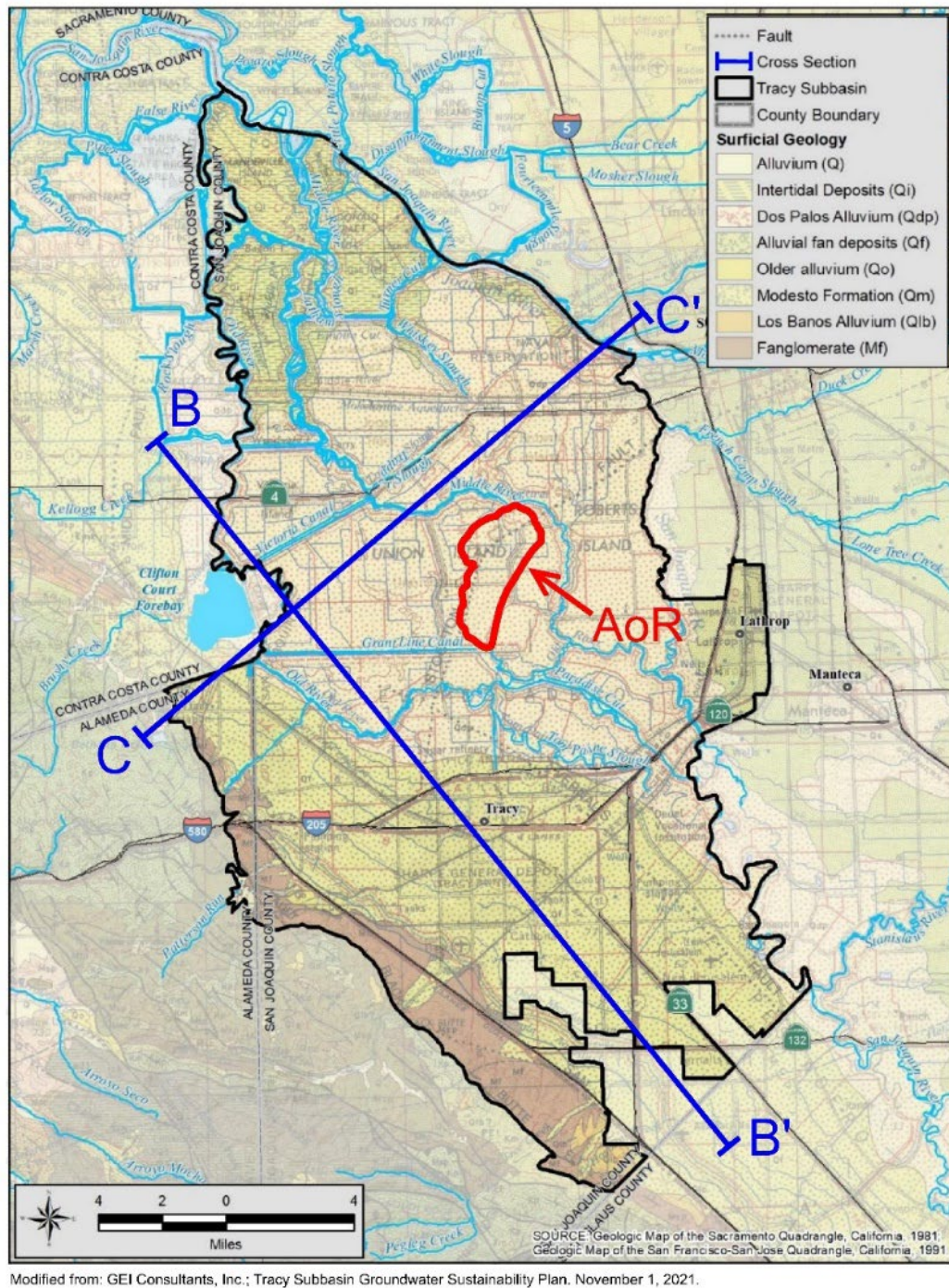
Figure A-43. Tracy Subbasin, surface geology, and cross section index map.
