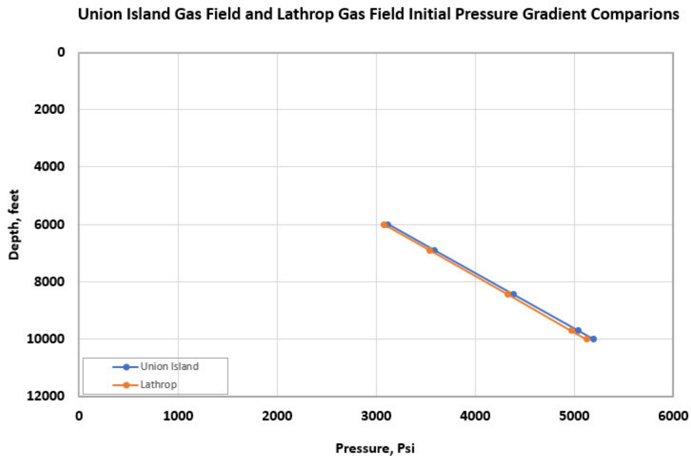
Figure A-25. Discovery pressure gradients at Union Island and Lathrop gas field
