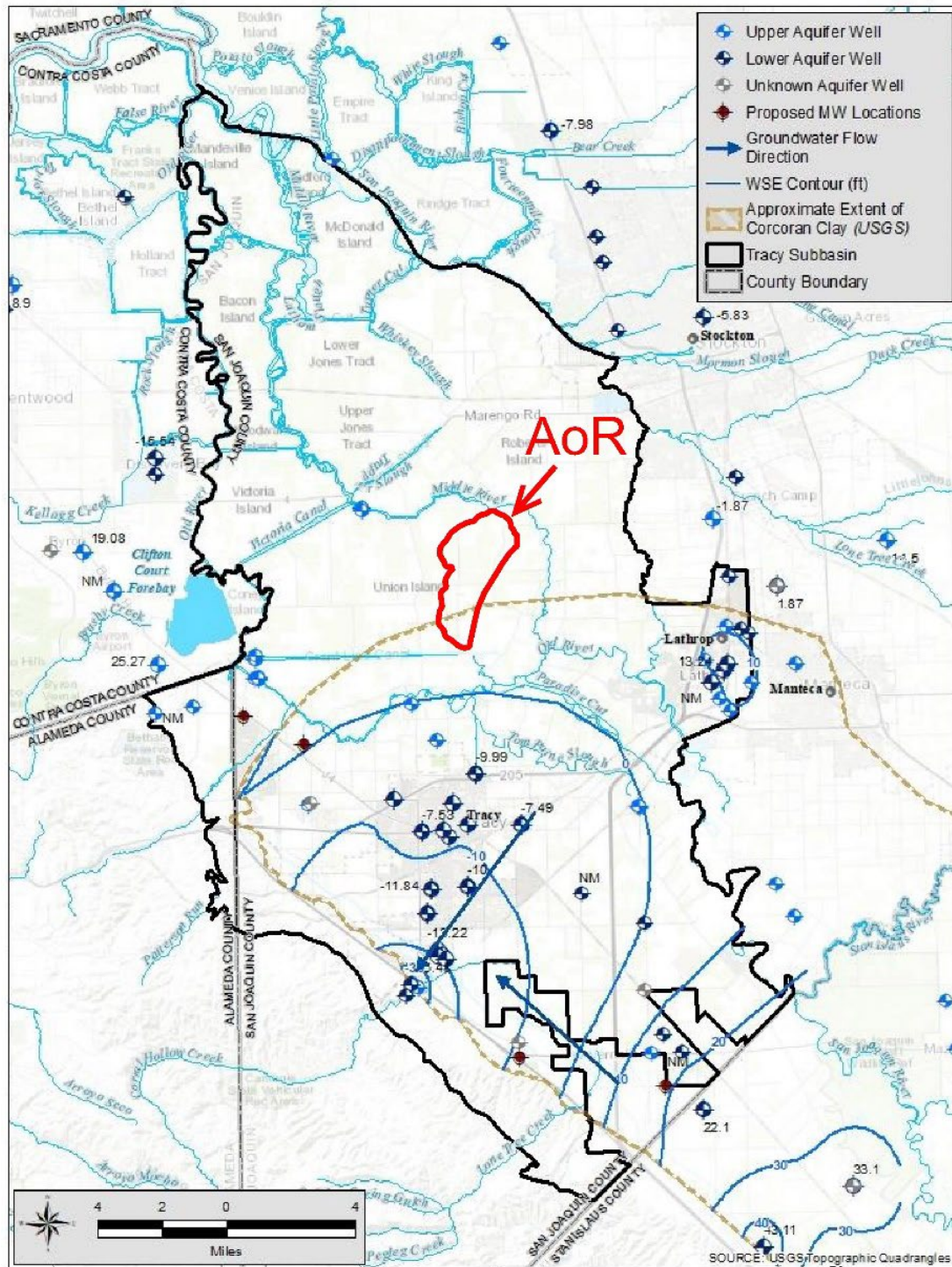
Figure A-53. Lower Aquifer groundwater elevations, spring 2019.
