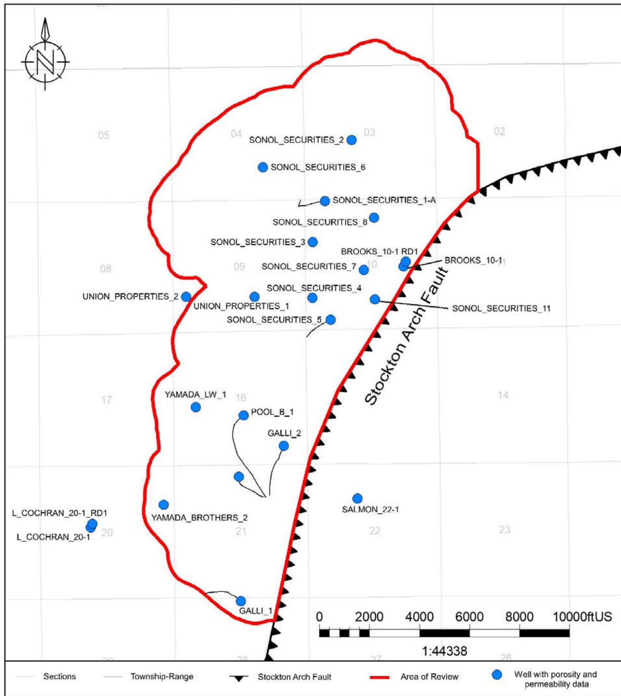
Figure A-31. Map of wells with porosity and permeability data.
