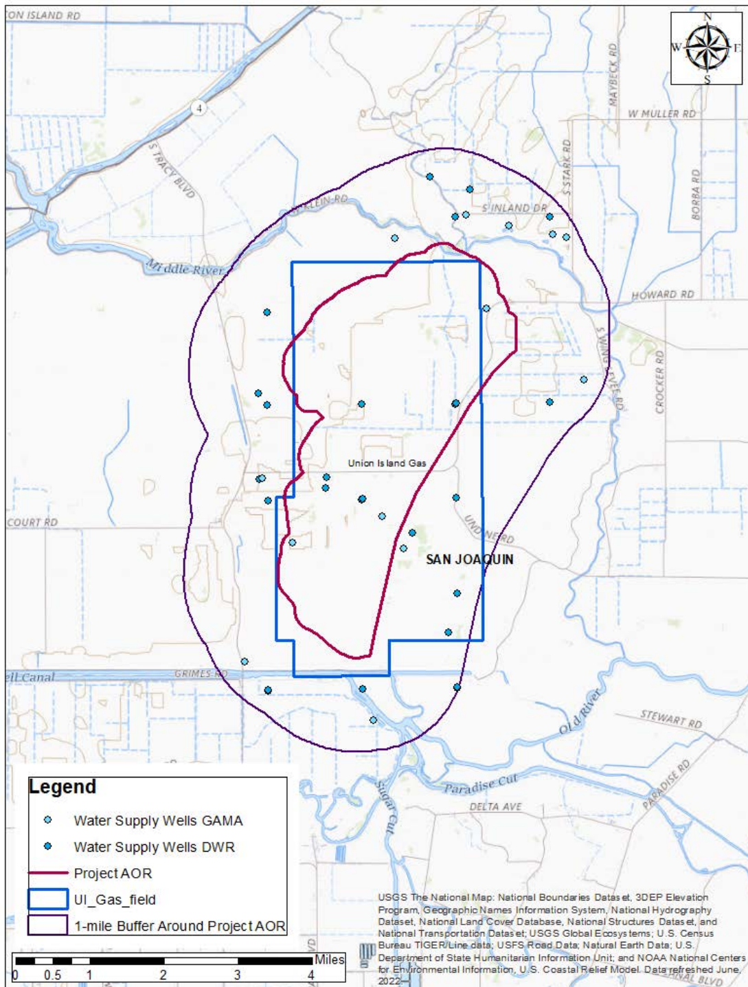
Figure A-54. Water well location map.
