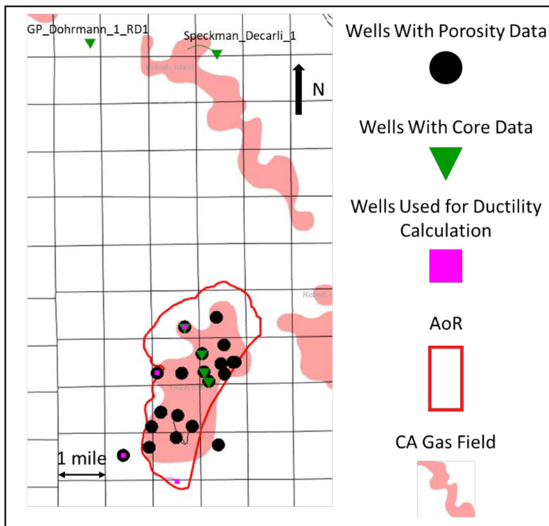
Figure A-26. Map showing location of wells with mineralogy data relative to the AoR.
