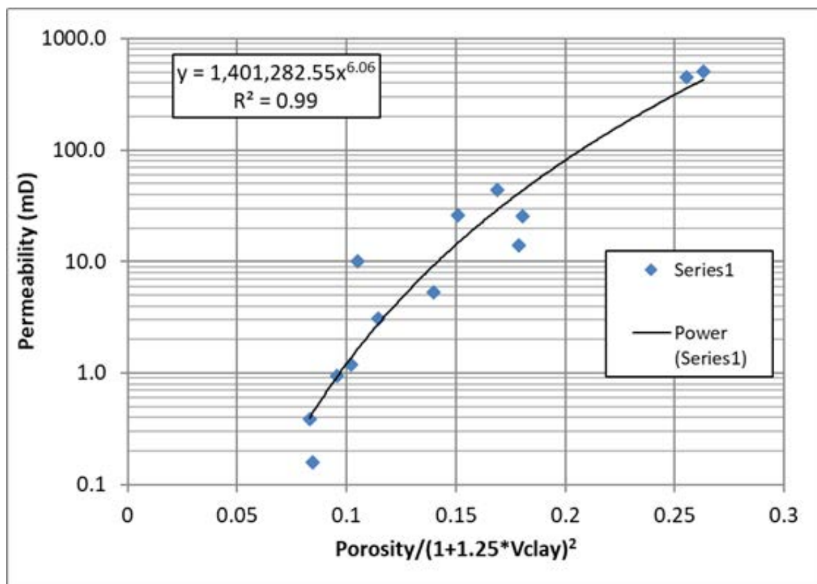
Figure A-27. Permeability transform for Sacramento basin zones.
