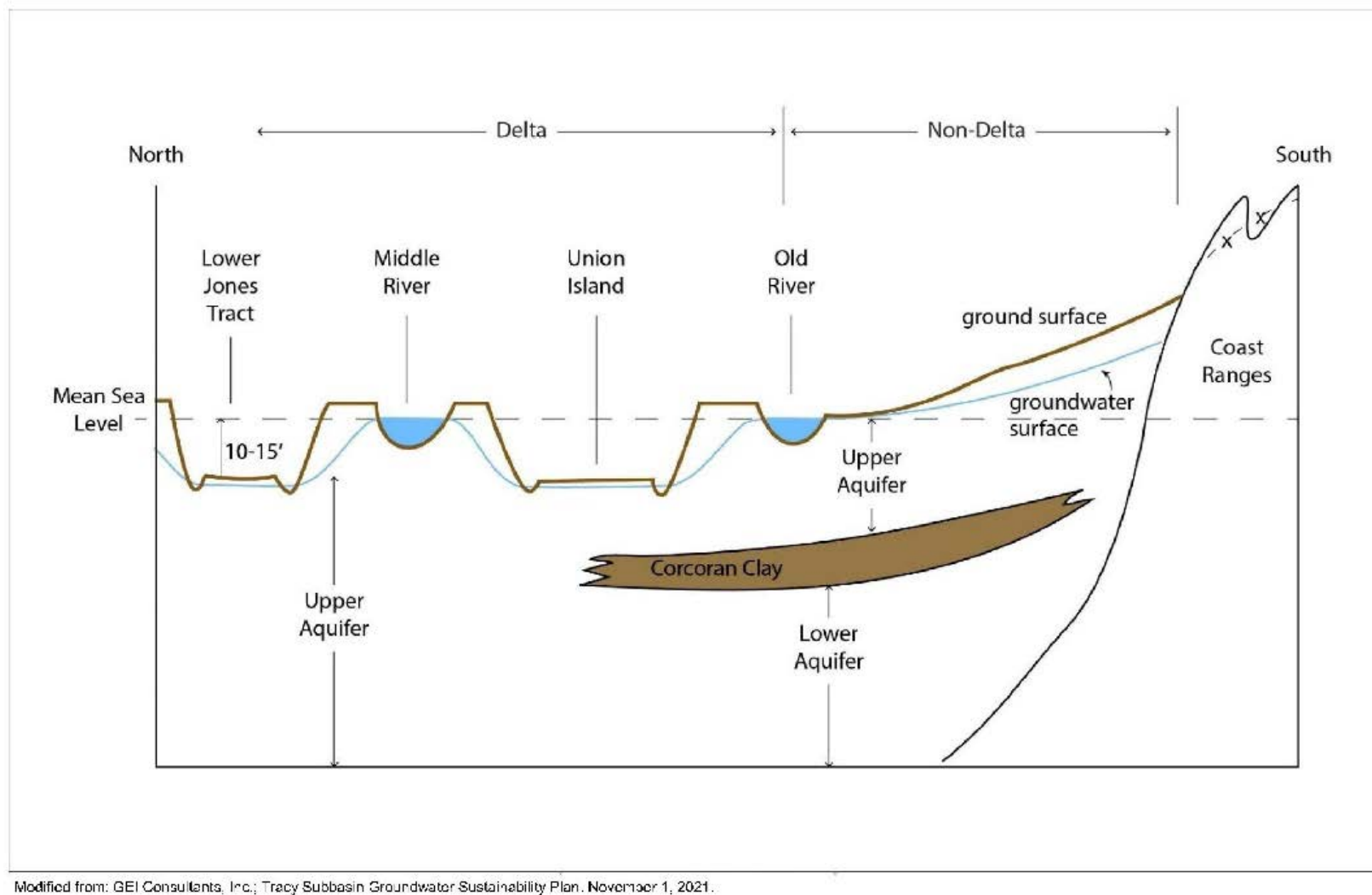
Figure A-51. Principal aquifer schematic profile.
