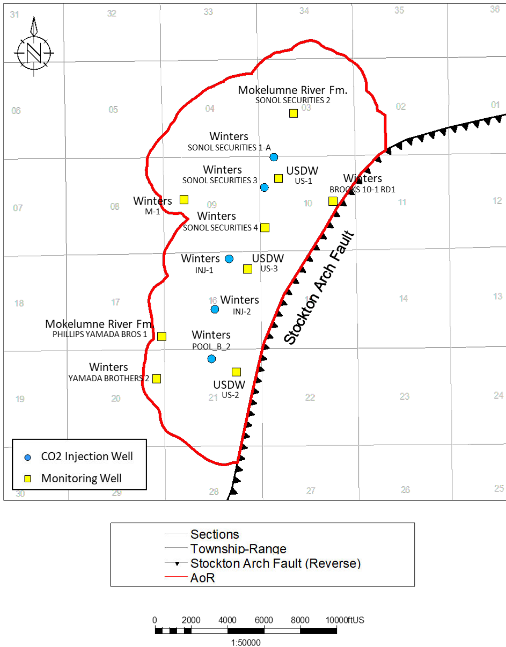
Figure A-59. Map showing the locations of injection wells and monitoring wells.
