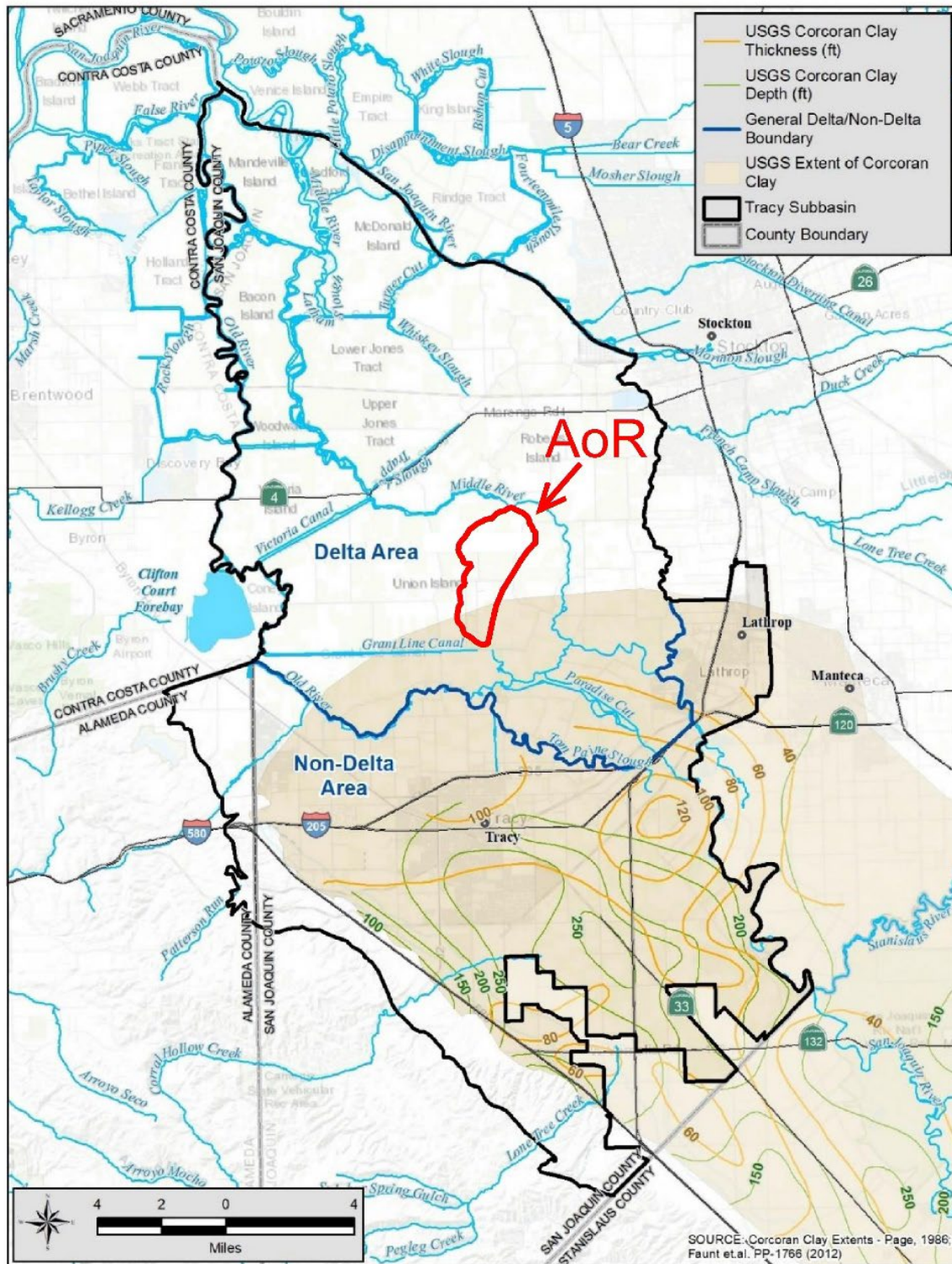
Figure A-47. Estimated Corcoran Clay thickness and extent.
