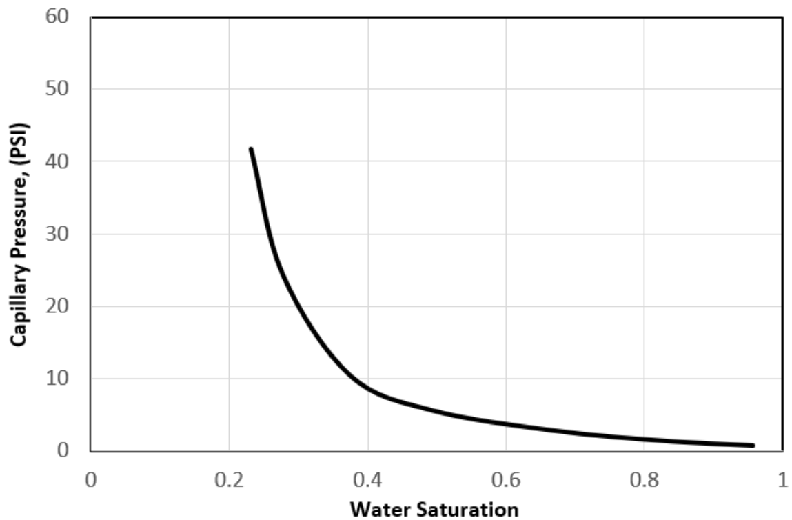
Figure A-32. Injection Zone capillary pressure curve used in computational modeling. Obtained from core sample from Sonol Securities 5 in the Union Island Gas Field.
