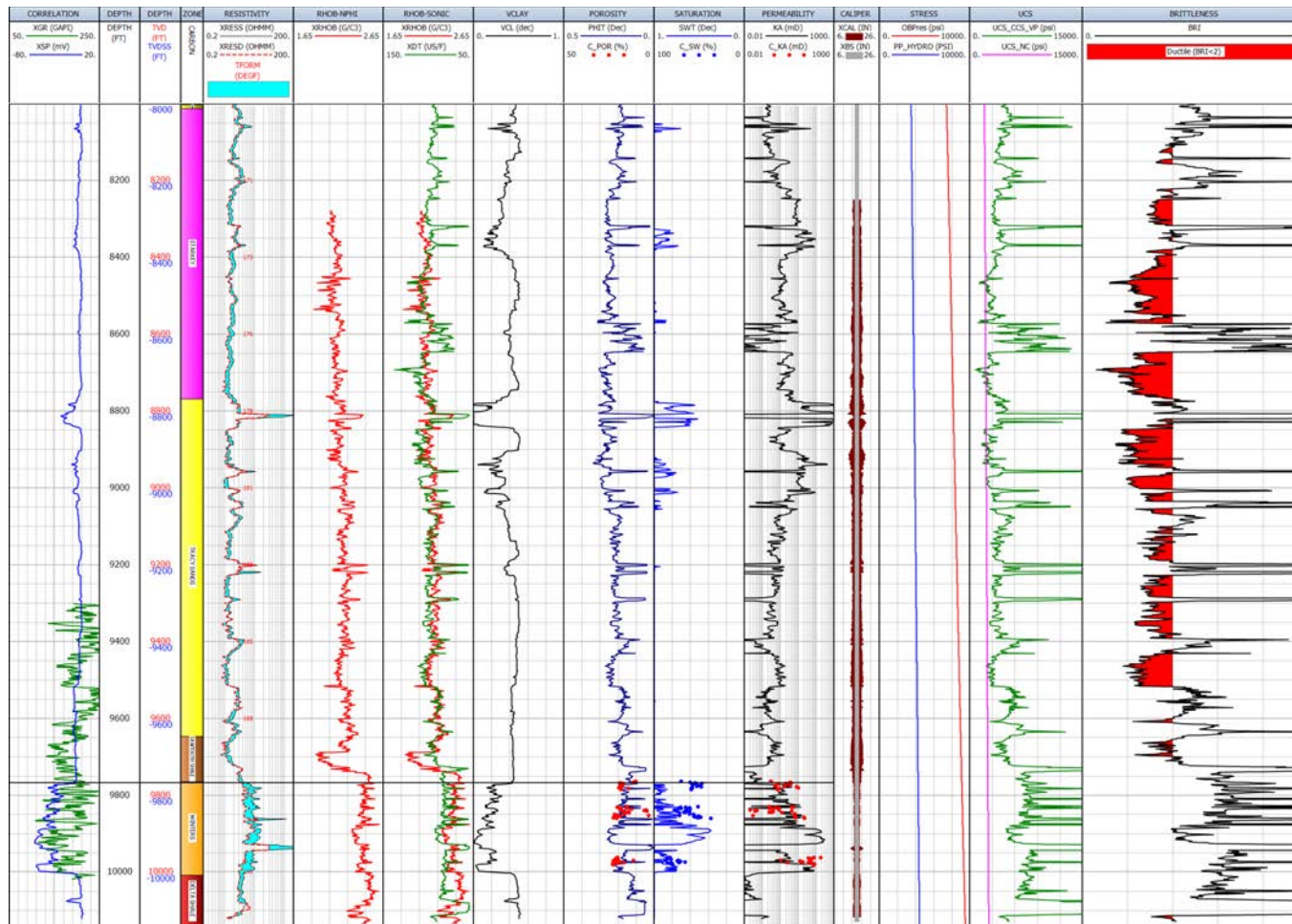
Figure A-34. Unconfined compressive strength and ductility calculations for Sonol_Securities_6. The upper confining zone ductility is less than two. Track 1: Correlation logs. Track 2: Measured depth. Track 3: Vertical depth and vertical subsea depth. Track 4: Zones. Track 5: Resistivity. Track 6: Density log. Track 7: Density and compressional sonic logs. Track 8: Volume of clay. Track 9: Porosity calculated from sonic and density. Track 10: Water saturation. Track 11: Permeability. Track 12: Caliper. Track 13: Overburden pressure and hydrostatic pore pressure. Track 14: UCS and UCS_NC. Track 15: Brittleness.
