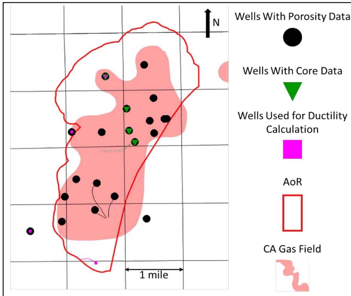
Figure A-10. Wells drilled in the Union Island Gas Field with porosity data are shown in black, wells with core are shown in green, and wells used for ductility calculation are shown in pink.
