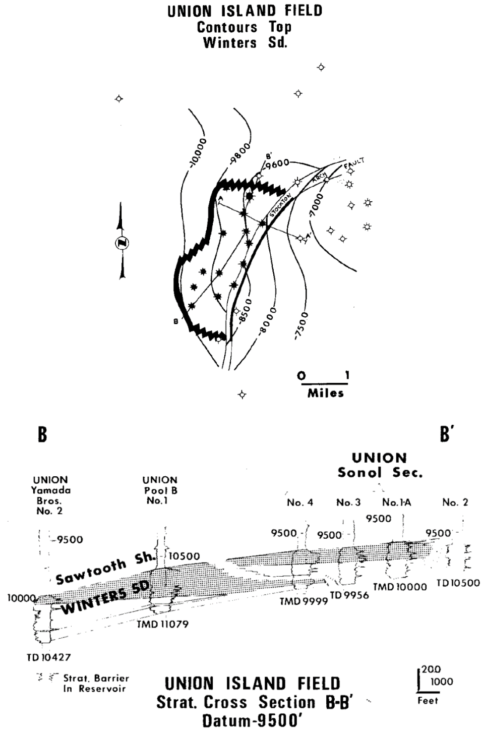
Figure A-16. Cross section B-B' across Union Island Gas Field displaying the flow barrier which separates the Northern and Southern field. Figures taken from Hill (1979), Figure 2 and 8.
