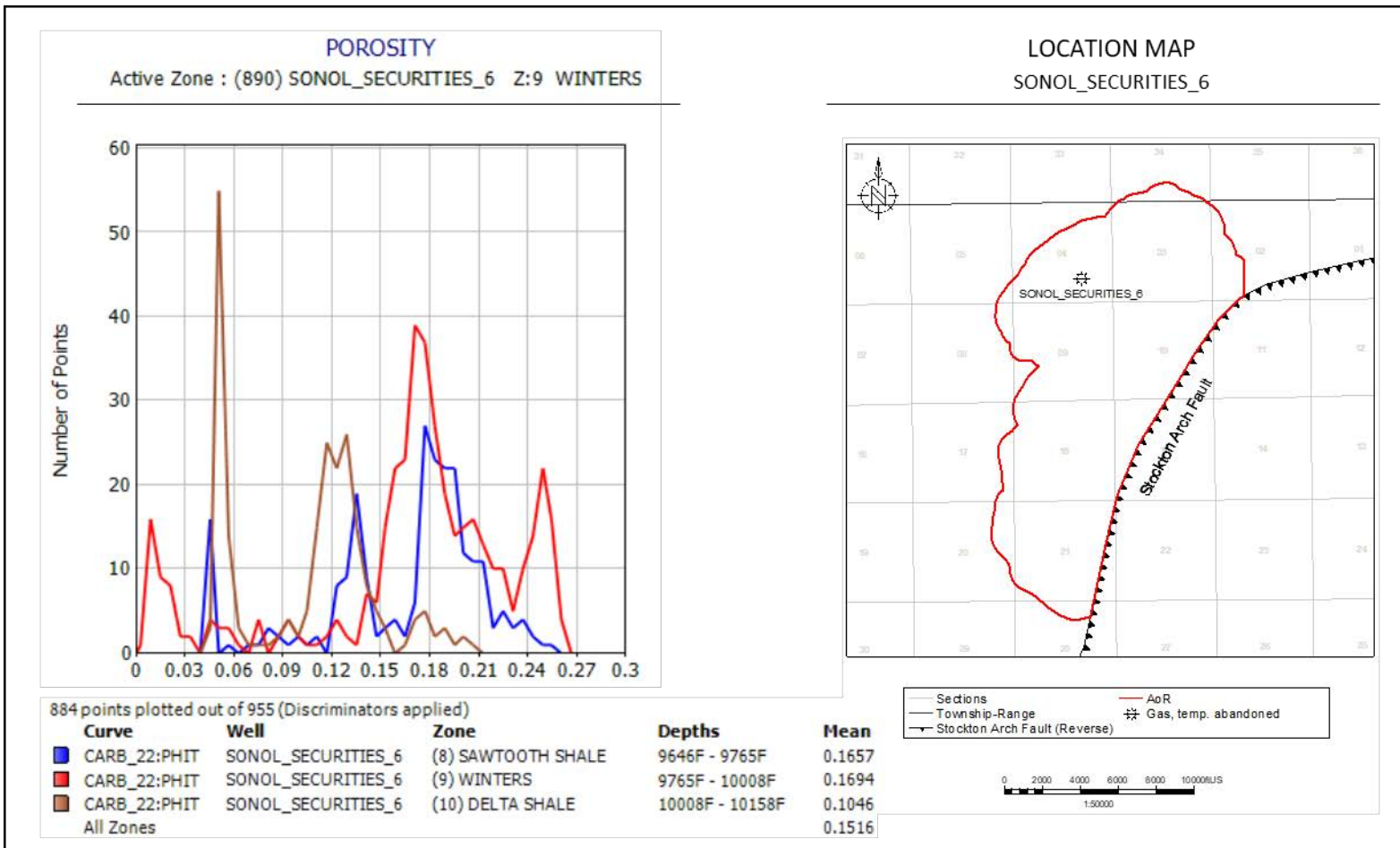
Figure A-28. Porosity histogram for well Sonol_Securities_6. In the histogram, blue represents the Sawtooth Shale, red the Winters Formation, and brown the Delta Shale. For the two shale intervals, only data with VCL>0.25 is shown, and for the Winters only data with VCL<=0.25 is shown.
