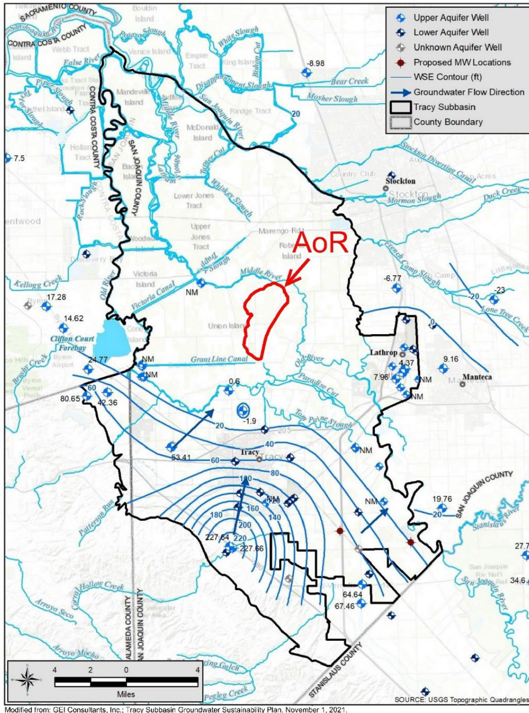
Figure A-52. Upper Aquifer groundwater elevations, Fall 2019.
