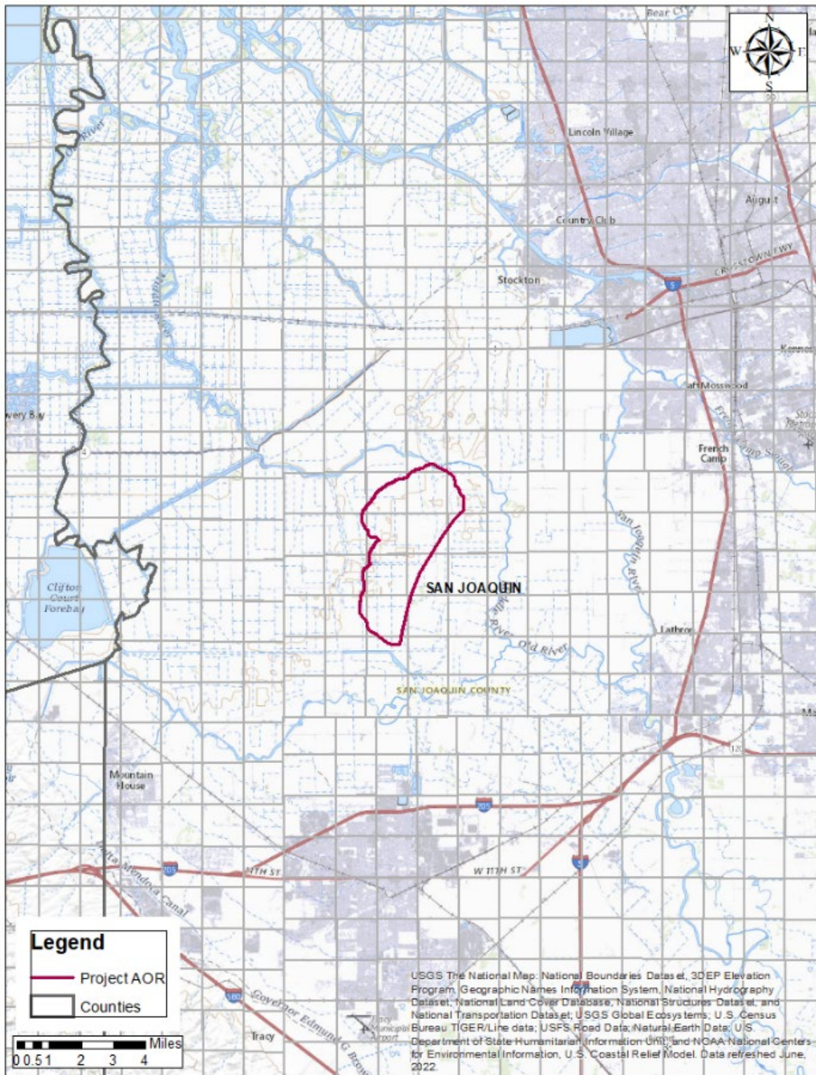
Figure A-17. Surface Features and the AOR
