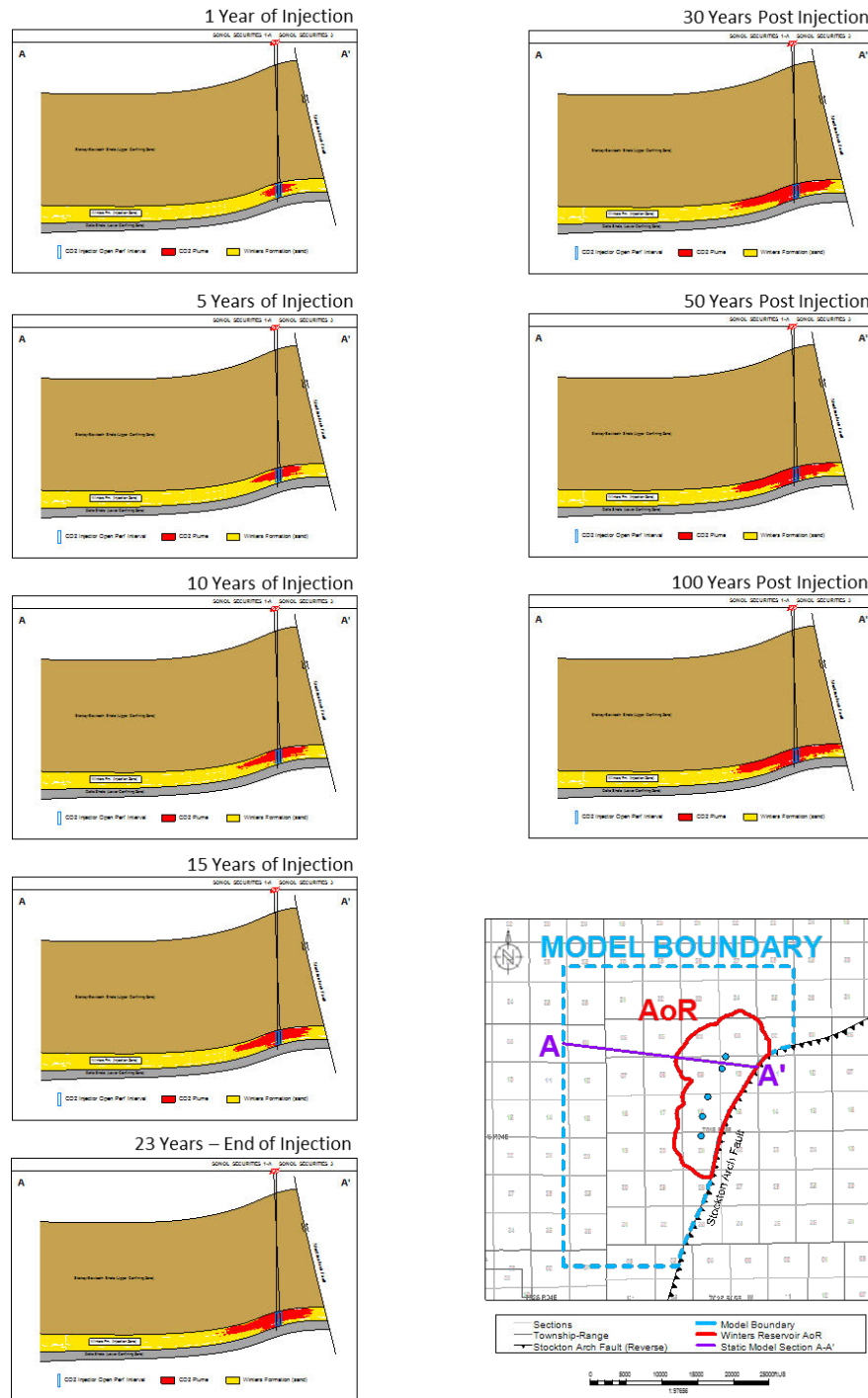
Figure A-58a. Section showing proximity of CO 2 (Injectate 1) to the Stockton Arch Fault and lateral dispersion of CO 2 throughout time and confinement under the overlying Starkey-Sawtooth through time for the five injector modeled Base scenario. As the sections show, plume growth over time is driven by the reservoir anticlinal structure, and is thus representative of the plume growth at all injector locations.
