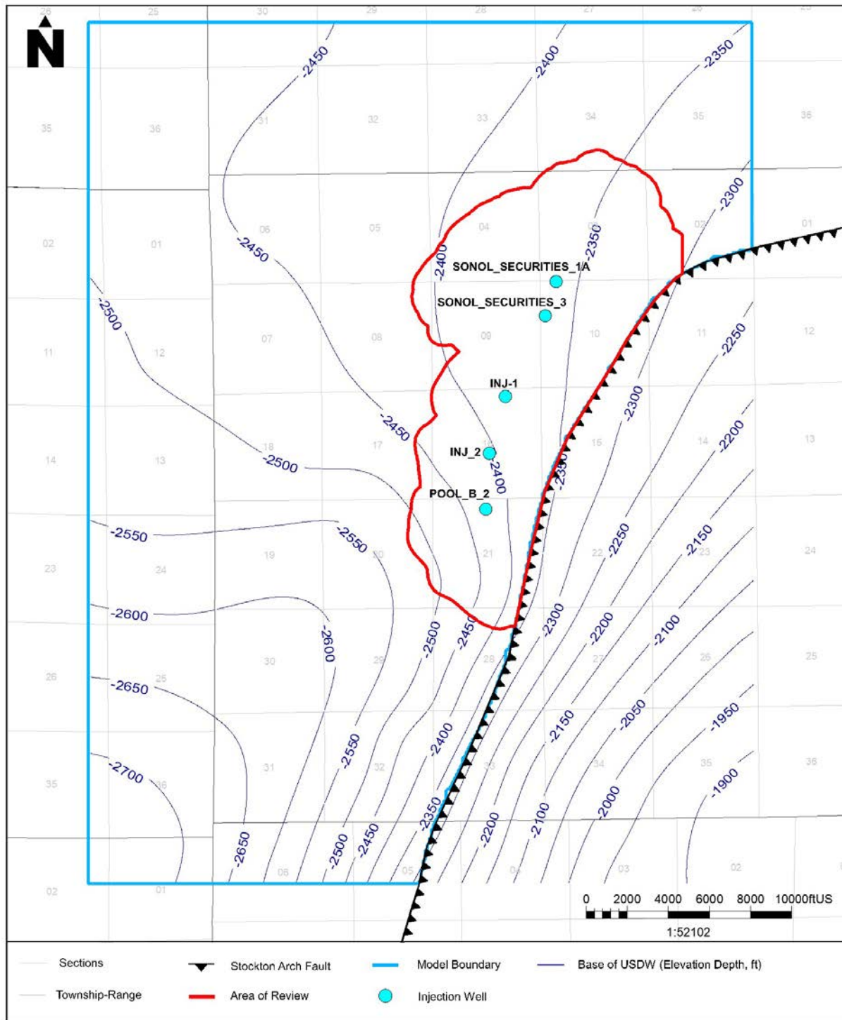
Figure A-46. Depth to the base of the lowermost USDW based on the calculation of salinity from logs (TVDSS).
