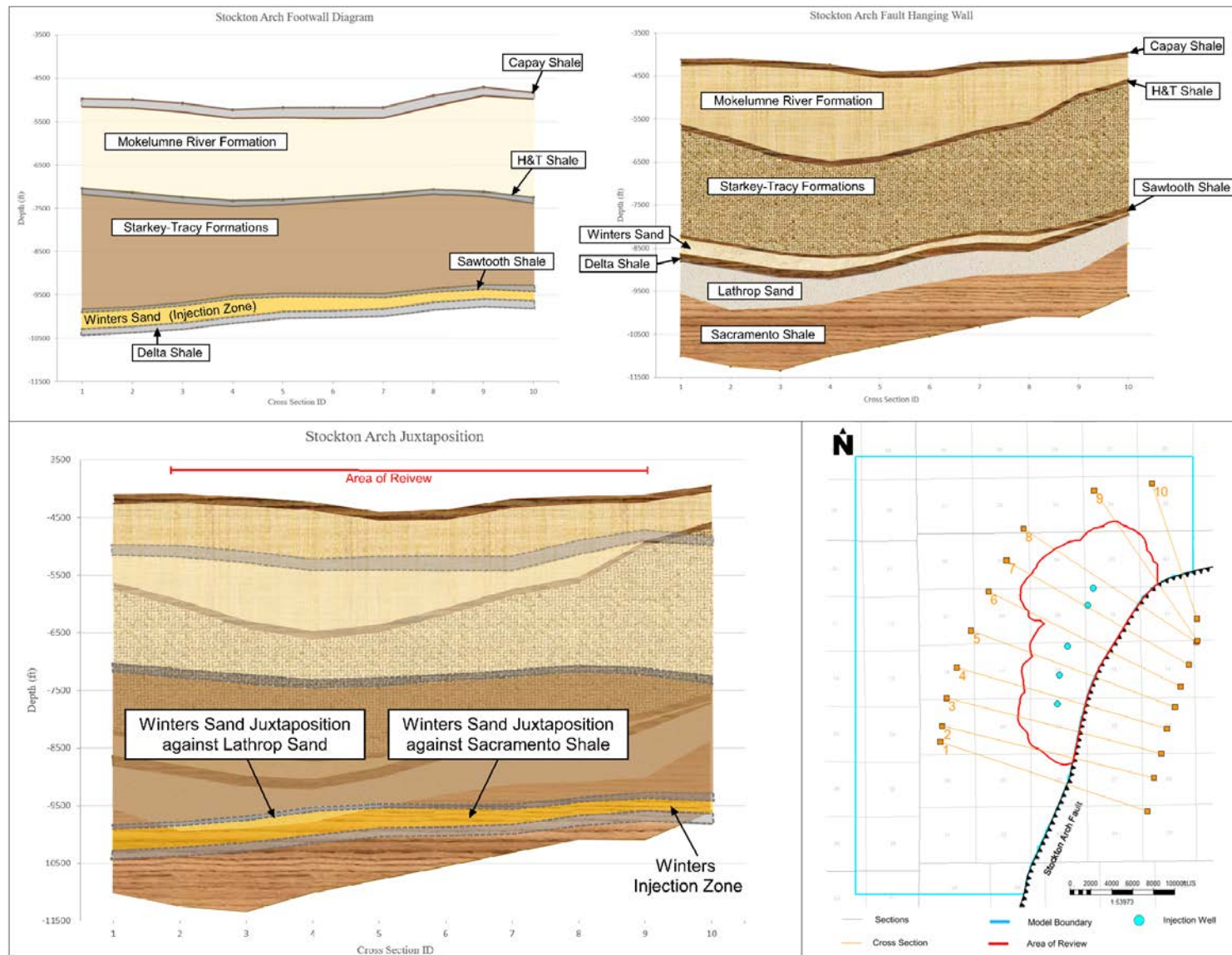
Figure A-22. Stockton Arch Fault Juxtaposition
