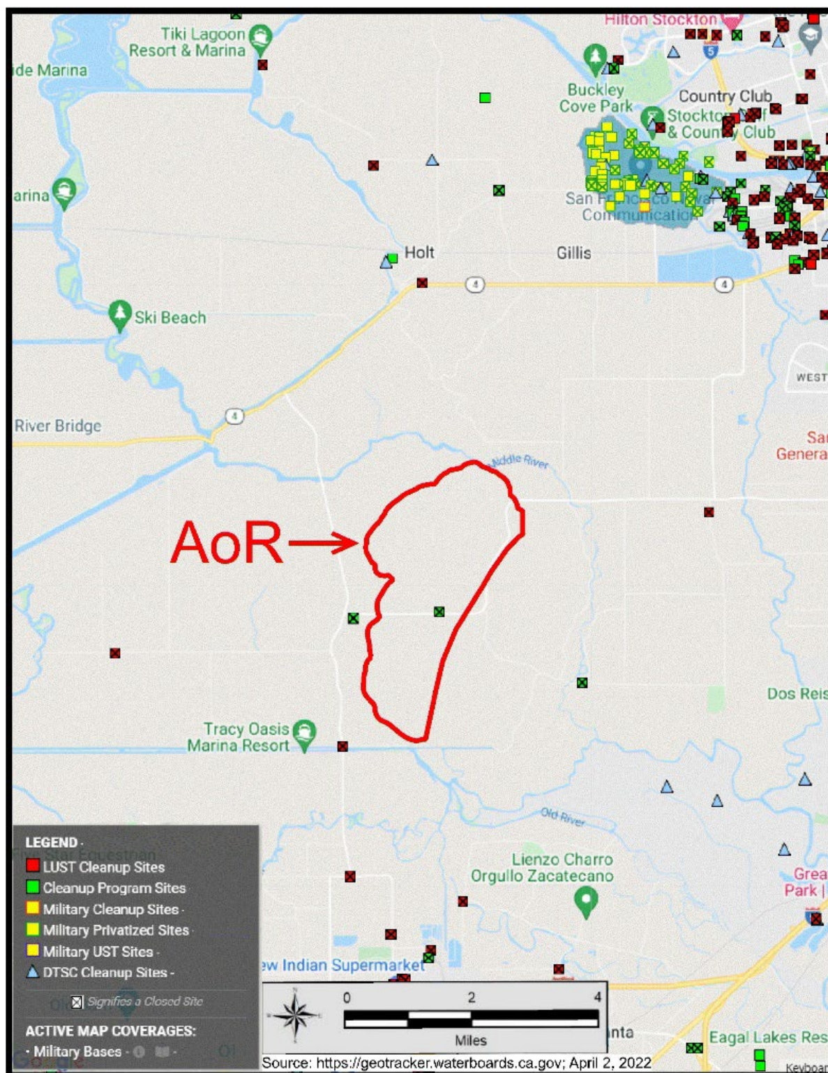
Figure A-18. State or EPA Subsurface Cleanup Sites.
