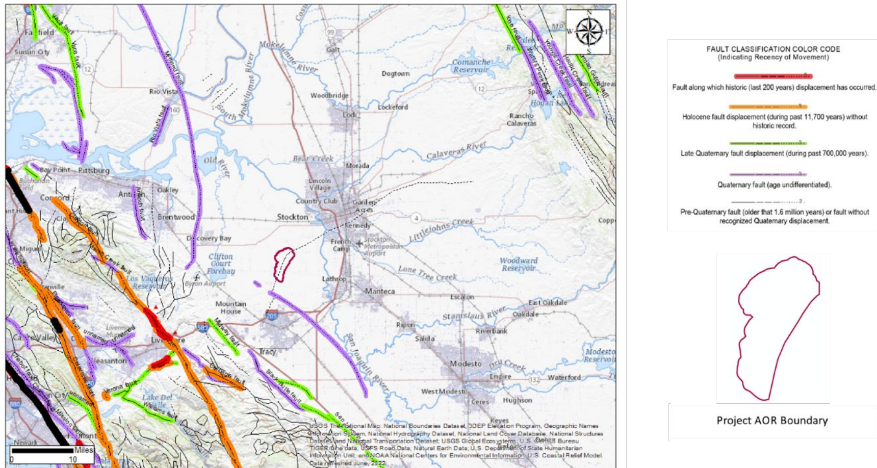
Figure A-40. Fault Activity Map from the California Geologic Survey and United States Geological Survey. The fault trace of the Stockton Fault shown here agrees with the 3D seismic interpretation. The fault trace is not colored indicating it is interpreted as Pre-Quaternary (older than 1.6 million years) by the California Geologic Survey. This is also in agreement with the seismic and well-based interpretation. ( https://maps.conservation.ca.gov/cgs/fam/ ).
