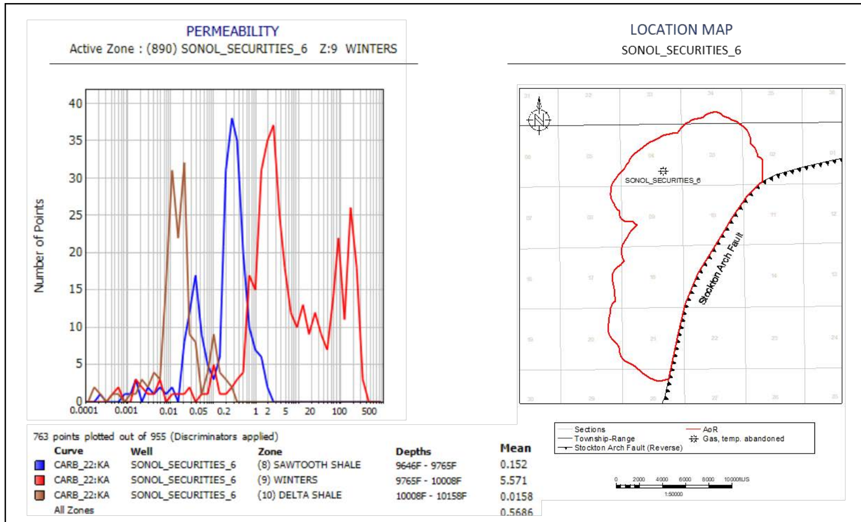
Figure A-29. Permeability histogram for well Sonol_Securities_6. In the histogram, blue represents the Sawtooth Shale, red the Winters Formation, and brown the Delta Shale. For the two shale intervals, only data with VCL > 0.25 is shown, and for the Winters only data with VCL \leq 0.25 is shown.
