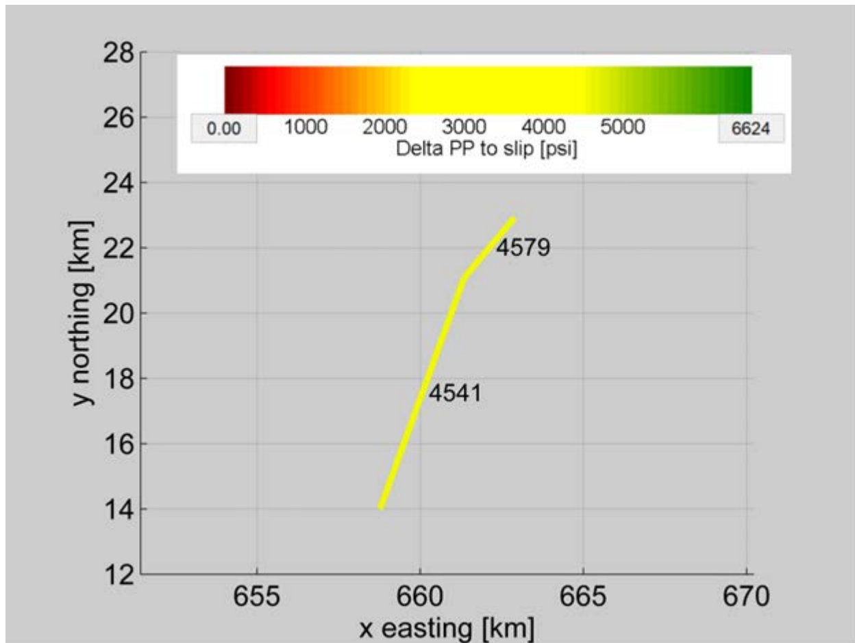
Figure A-39. Map showing the two modeled segments of the Stockton Arch Fault. The numbers on the plot represent the necessary increase in pore pressure above present-day conditions to cause failure on that fault segment.
