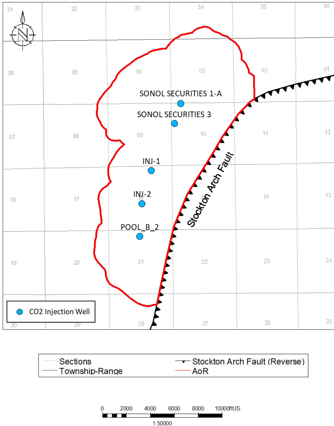
Figure A-15. AoR and injection well location map for the project area. Minimum distance between injection wells is 1,735 feet and maximum distance is 4,390 feet.
