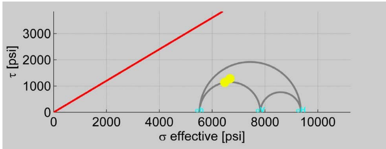
Figure A-38. Mohr circle of the Winters reservoir at present-day conditions. The normal stress (x-axis) and shear stress (y-axis) on the two Stockton Arch fault segments is represented by the two yellow dots. The red line represents the Mohr coulomb failure surface assuming a coefficient of friction of 0.6 and a fault cohesion of 0 psi.
