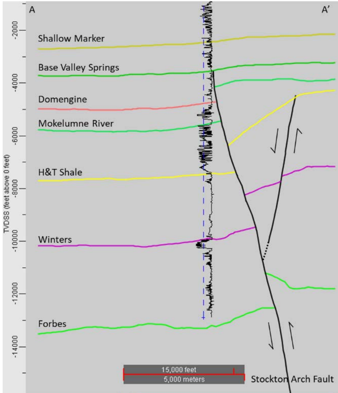
Figure A-20. Structural cross section across the geologic model. Well Union Properties 2 (04077203220000) is shown with SP log (negative values to left) for correlation and geologic packages. Geologic surfaces developed from seismic interpretation. The Stockton Arch Fault is cut-off by the Base Valley Springs. The interpreted antithetic fault to the east is dashed into the Stockton Arch Fault.
