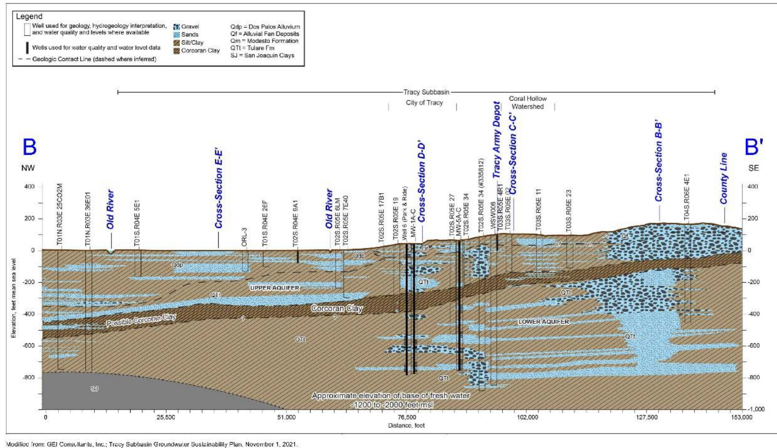
Figure A-48. Geologic cross section B-B'.
