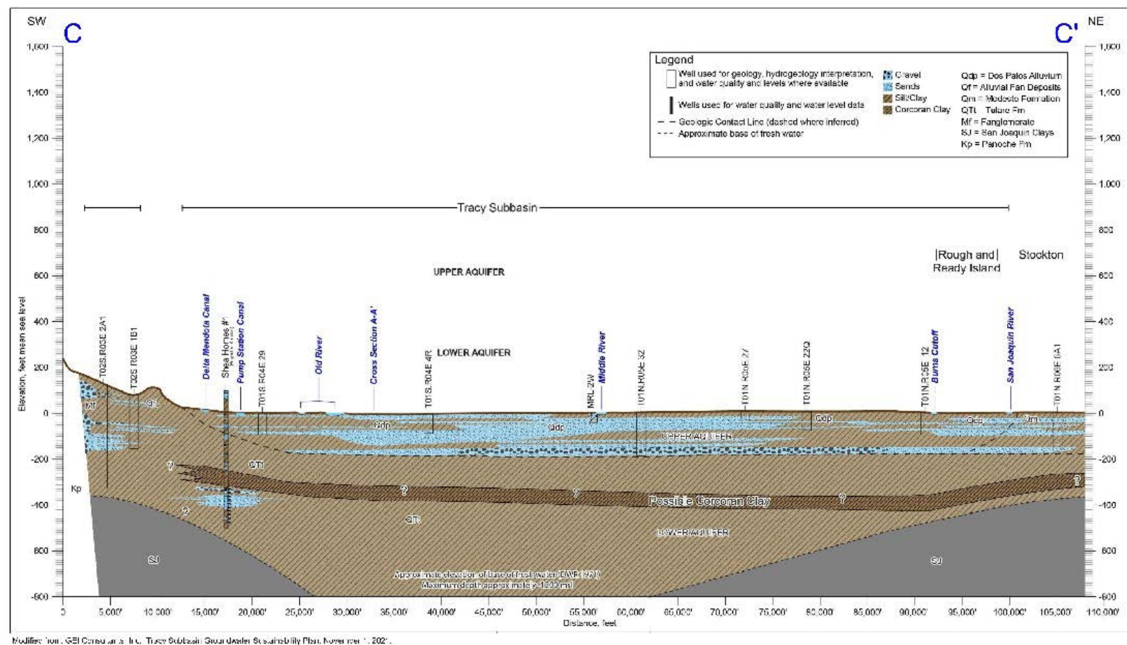
Figure A-49. Geologic cross section C-C'.
