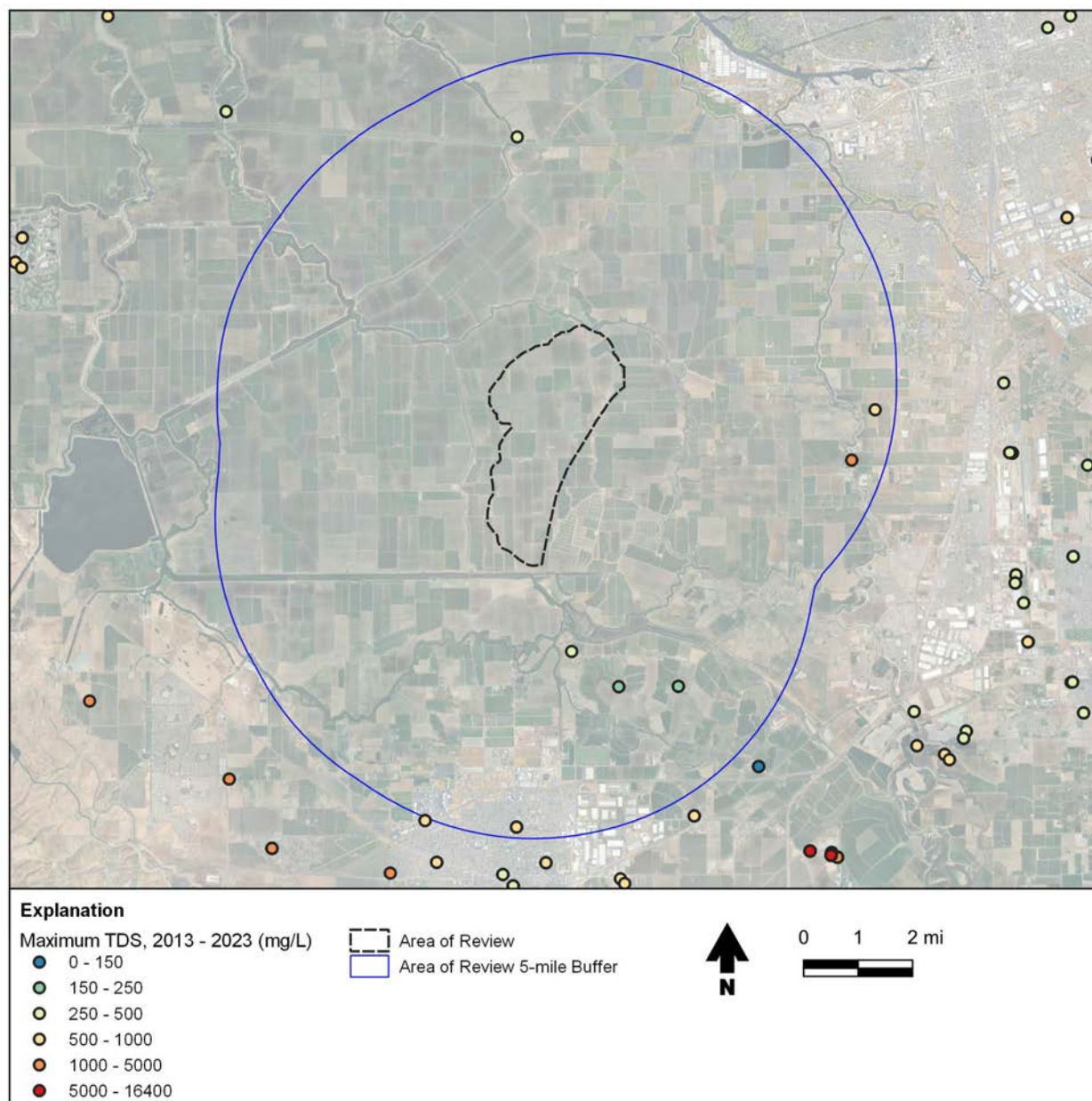
Figure A-50. Total Dissolved Solids (TDS) from water supply wells, 2013 – 2023. Data from California State Water Resources Control Board Groundwater Ambient Monitoring and Assessment (GAMA) Program. Maximum reported well depth within 5-mile AoR buffer is 732 feet.
