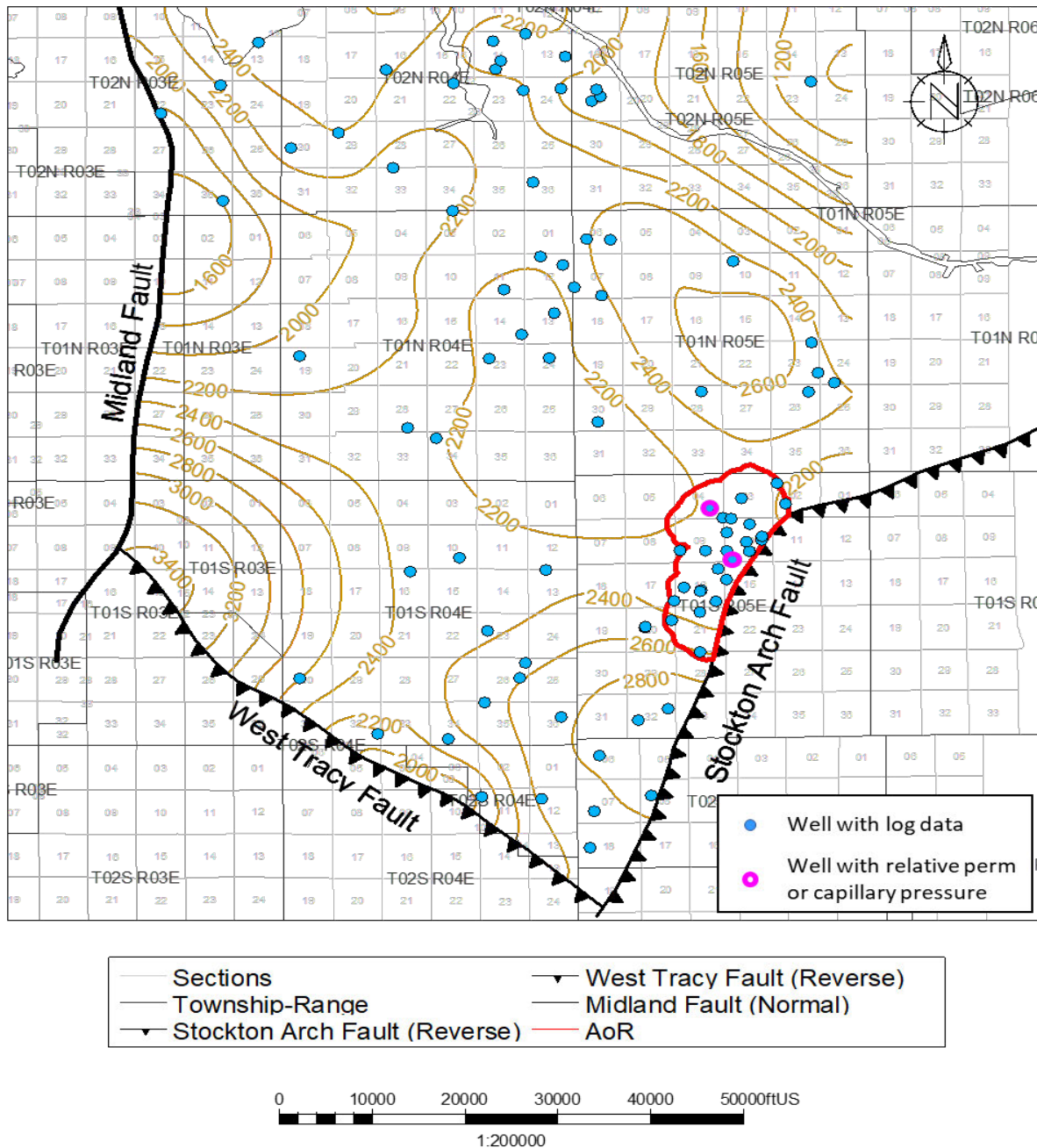
Figure A-7. Starkey-Sawtooth Shale isopach map for the greater storage project area. Wells shown as blue dots on the map penetrate the Starkey-Sawtooth Shale and have open-hole logs. Wells with relative permeability or capillary pressure data are shown as magenta circles.
