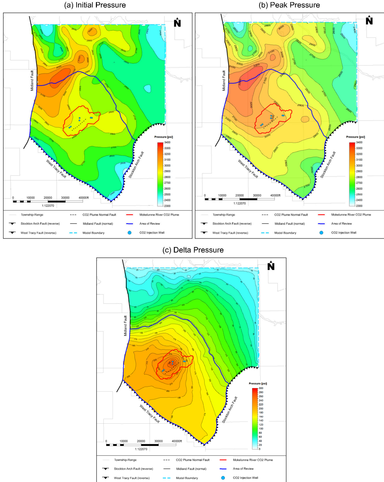
Figure E-5: (a) Initial pressure across the model boundary, (b) Peak pressure across the model boundary, (c) Delta pressure across the model boundary.
