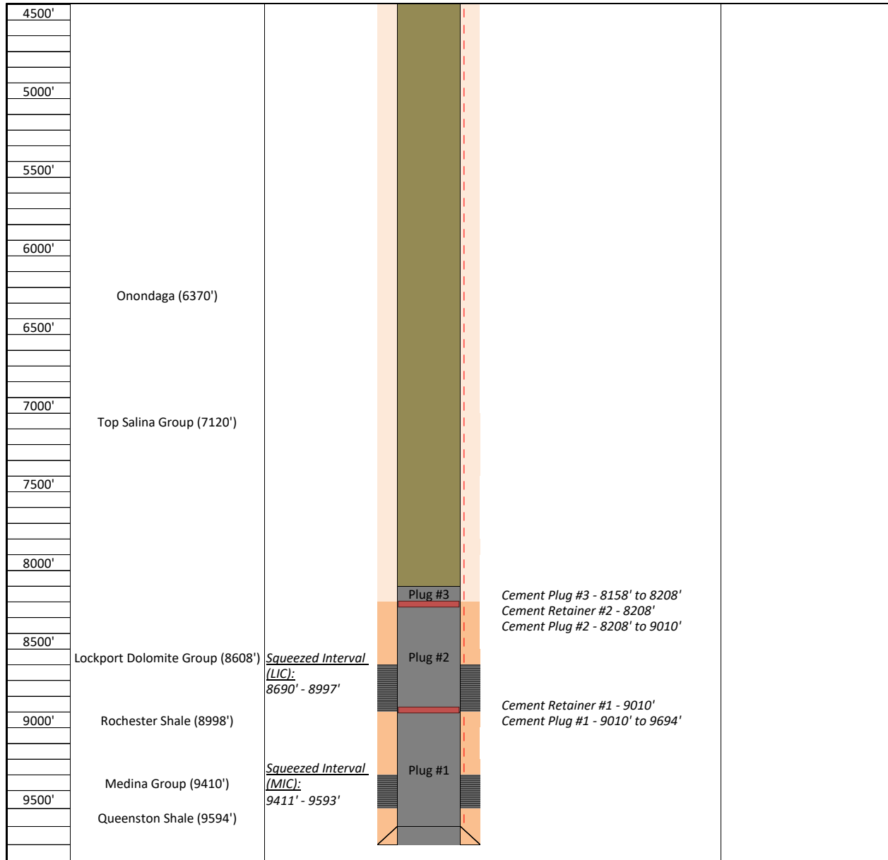
Figure 4: Proposed well schematic for TR2-4 after plugging the injection well to surface. Well schematic split in two for illustration purposes, 2/2: 4,500 ft to 9,800 ft.
