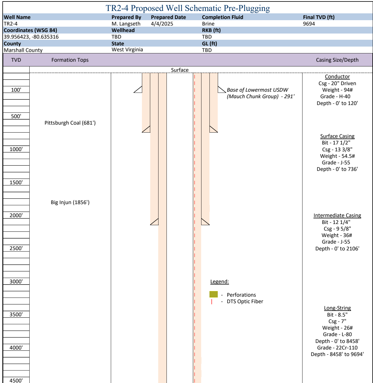
Figure 1: Proposed well schematic for TR2-4 after pulling the completion and before plugging the injection well. Well schematic split in two for illustration purposes, 1/2: Surface to 4,500 ft.
