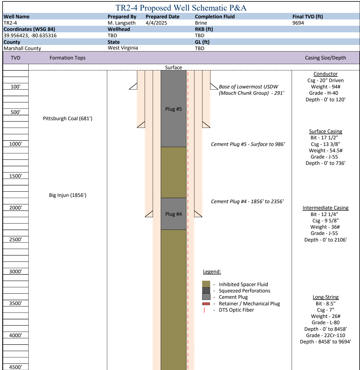
Figure 3: Proposed well schematic for TR2-4 after plugging the injection well to surface. Well schematic split in two for illustration purposes, 1/2: Surface to 4,500 ft.
