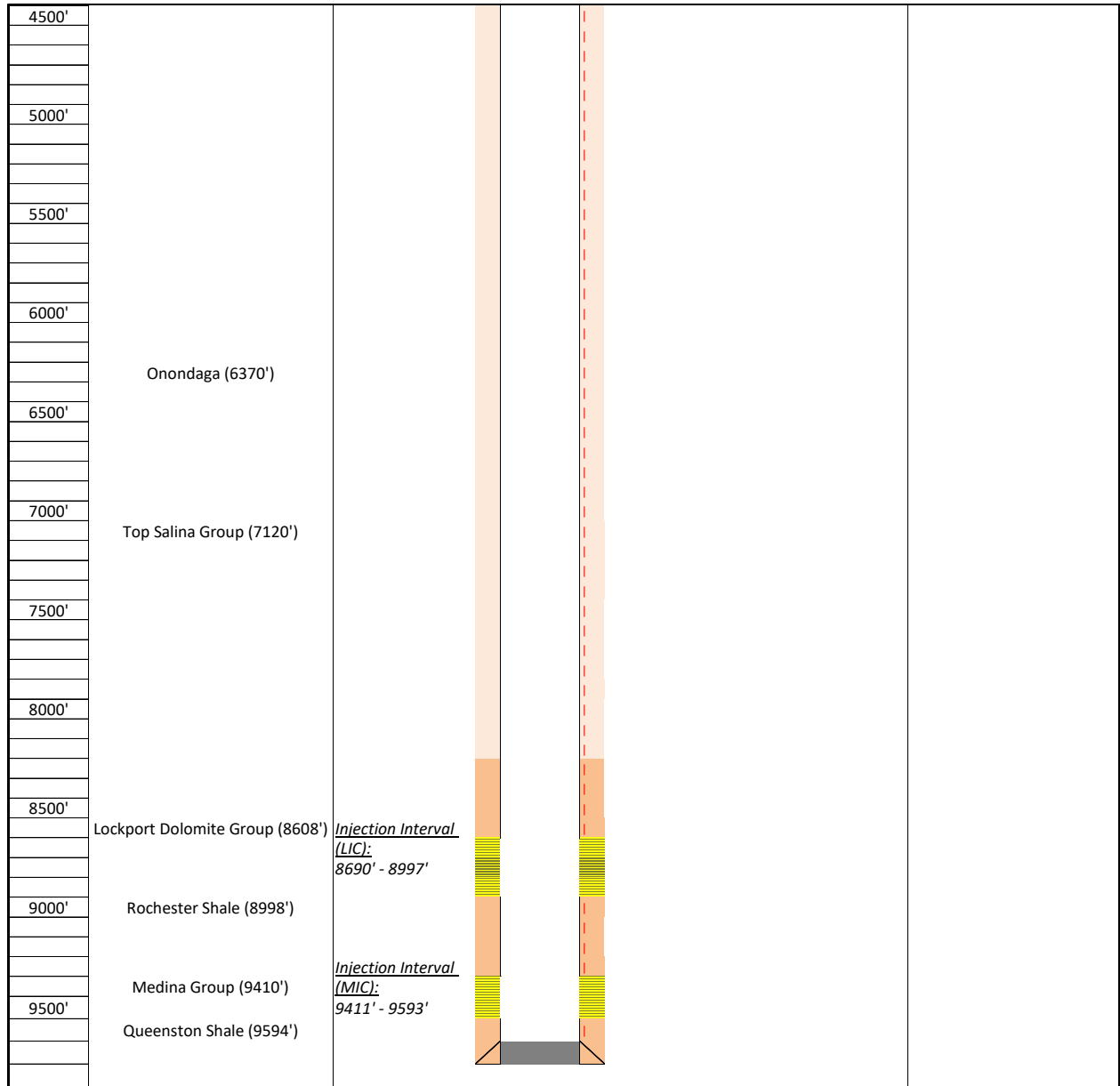
Figure 2: Proposed well schematic for TR2-4 after pulling the completion and before plugging the injection well. Well schematic split in two for illustration purposes, 2/2: 4,500 ft to 9,800 ft.
