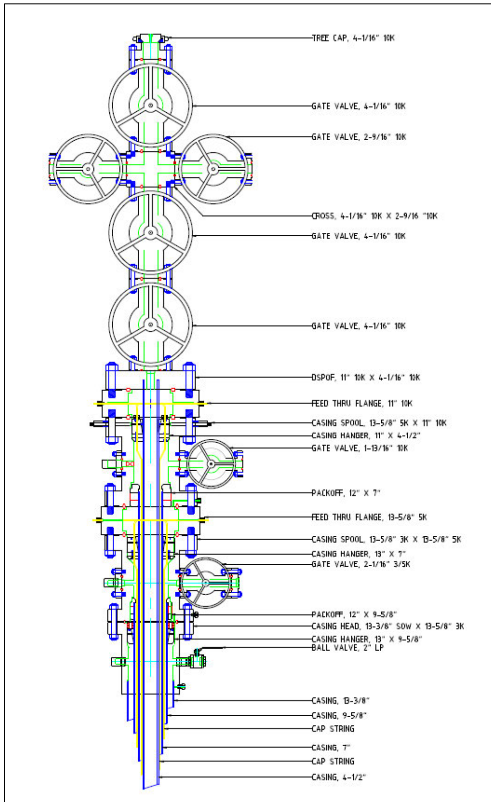
Figure 3: Proposed wellhead design for the Lambda-Brown 4-1 CO 2 injection well.
