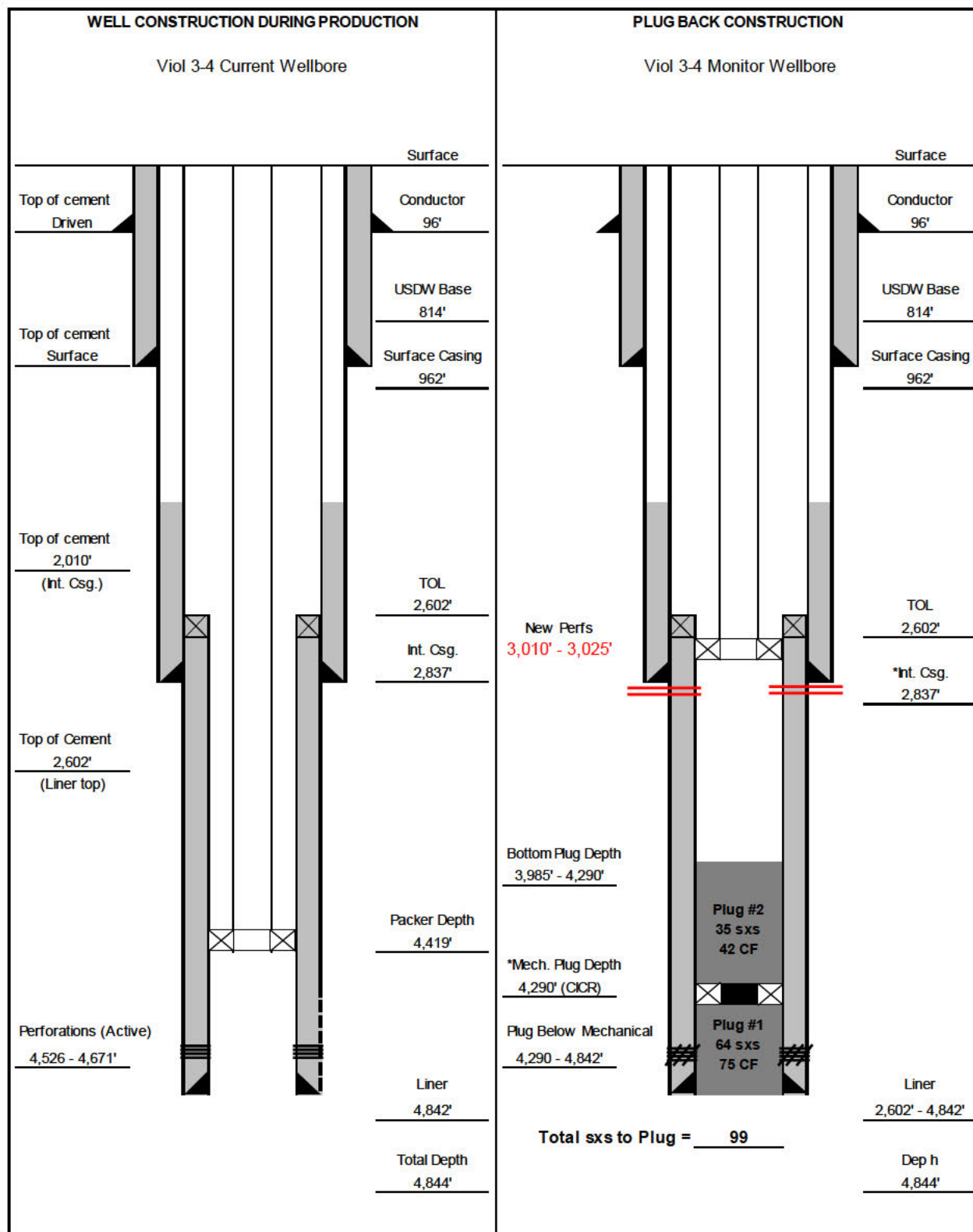
Figure 5: Current and proposed wellbore diagram for the Viol Et Al 3-4 well.
