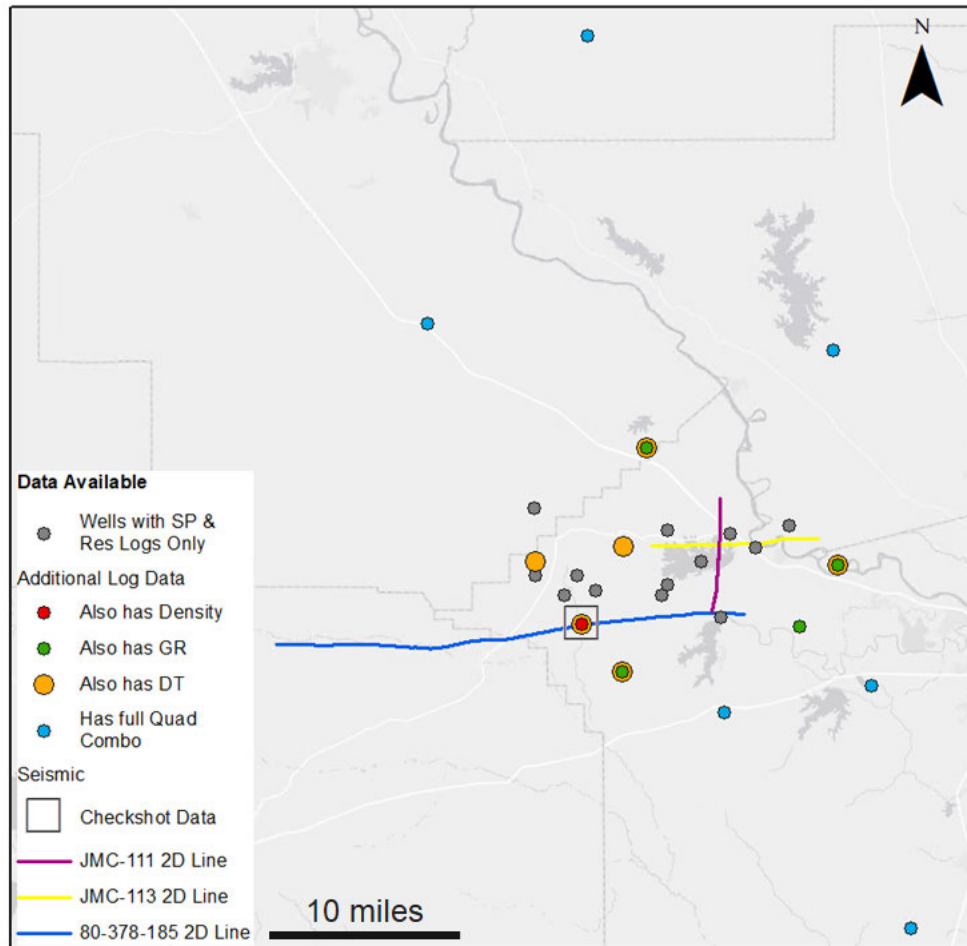
Figure 1-10: Map of the wells selected for log data analysis and location of purchased 2D seismic lines. The well highlighted in red was used to create a well-tie to tie the seismic time data to depth for integration into the model.
