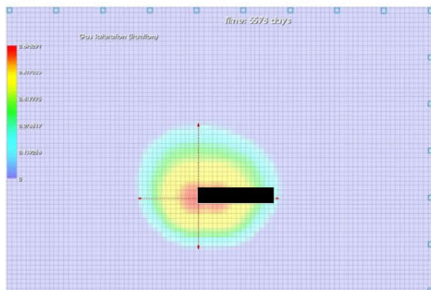
Figure 4. Plume after 15 years of injection
