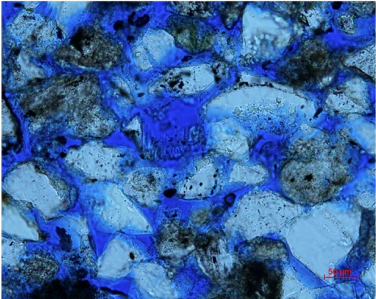
Figure 1-9 – Thin section image of fine-grained Miocene sandstone sample. Blue is pore space and white is quartz grains with little calcite cementation present (Meckel & Trevino, 2014).
