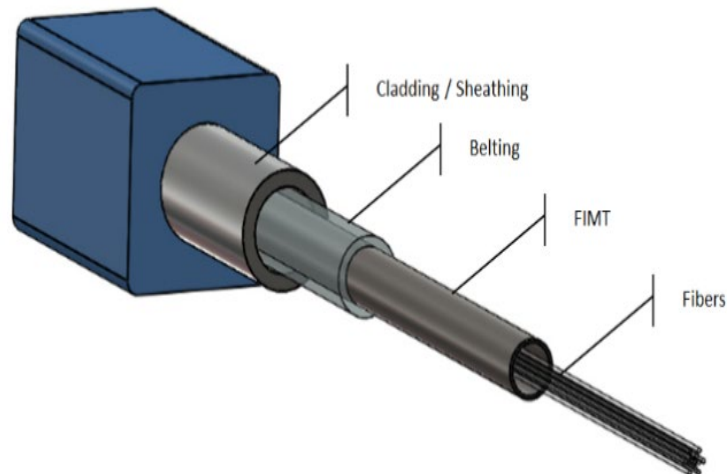
Figure 5-14 – SureVIEW with CoreBright Optical Fiber
