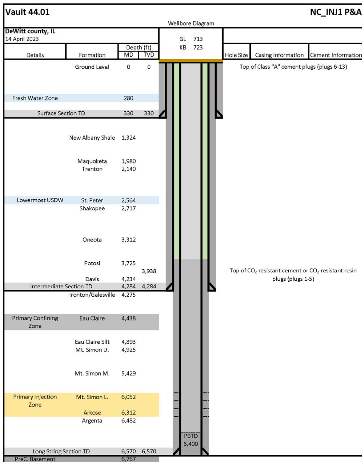
Figure 1: Injection well plugging schematic for NC_INJ1.
