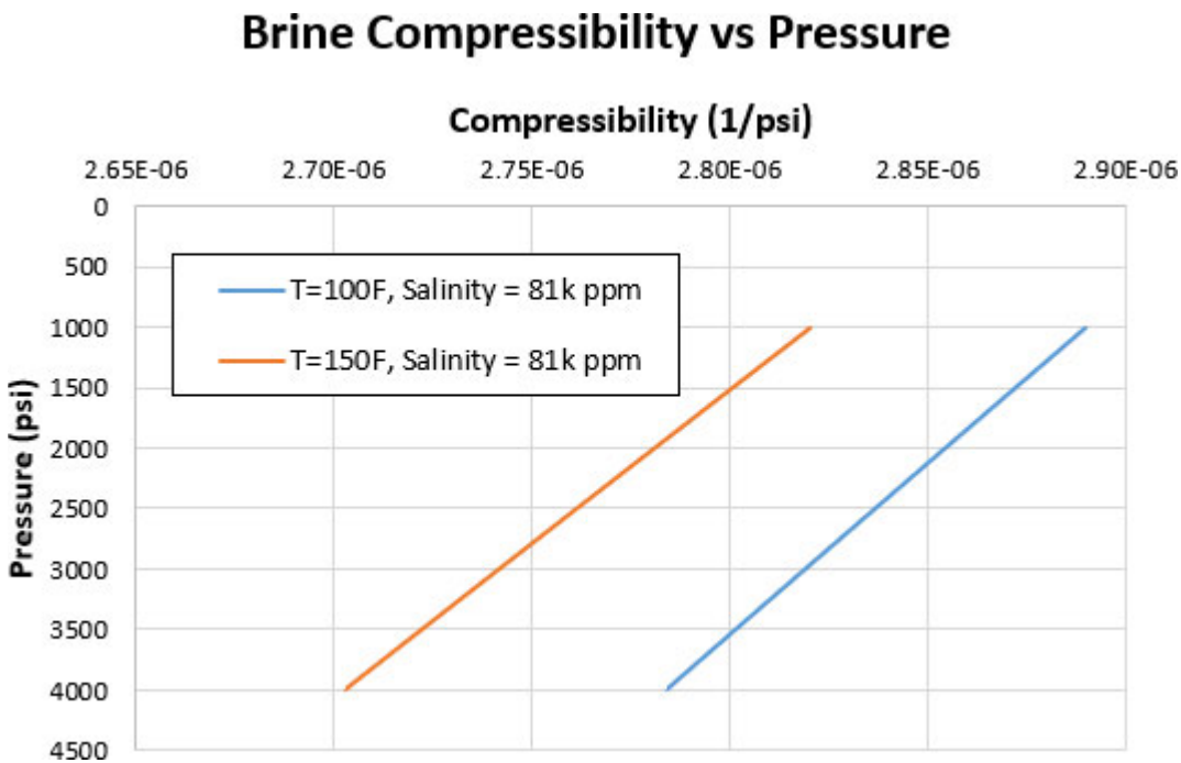
Figure 3-8: Brine compressibility at Different Pressure and Temperature
