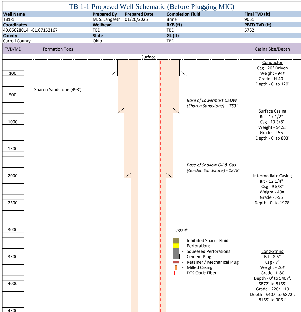
Figure 5: Proposed well schematic for TB1-1 after pulling the completion and before plugging the MIC. Well schematic split in two for illustration purposes, 1/2: Surface to 4,500 ft.
