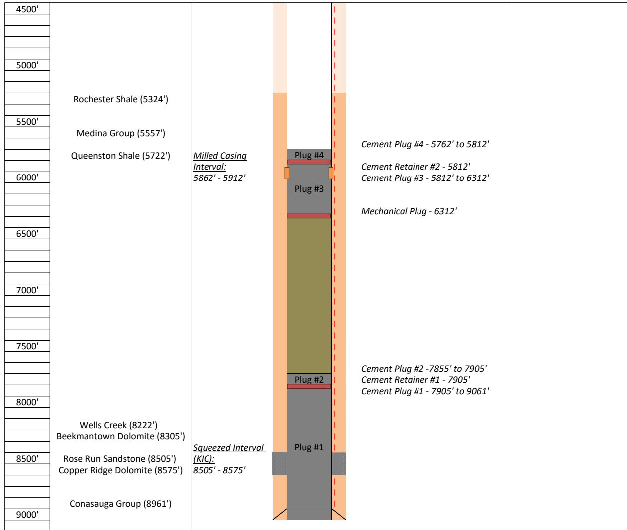
Figure 4: Proposed well schematic for TB1-1 after plugging from the KIC to the Queenston Shale (lower confining zone of MIC). Well schematic split in two for illustration purposes, 2/2: 4,500 ft to 9,100 ft.
