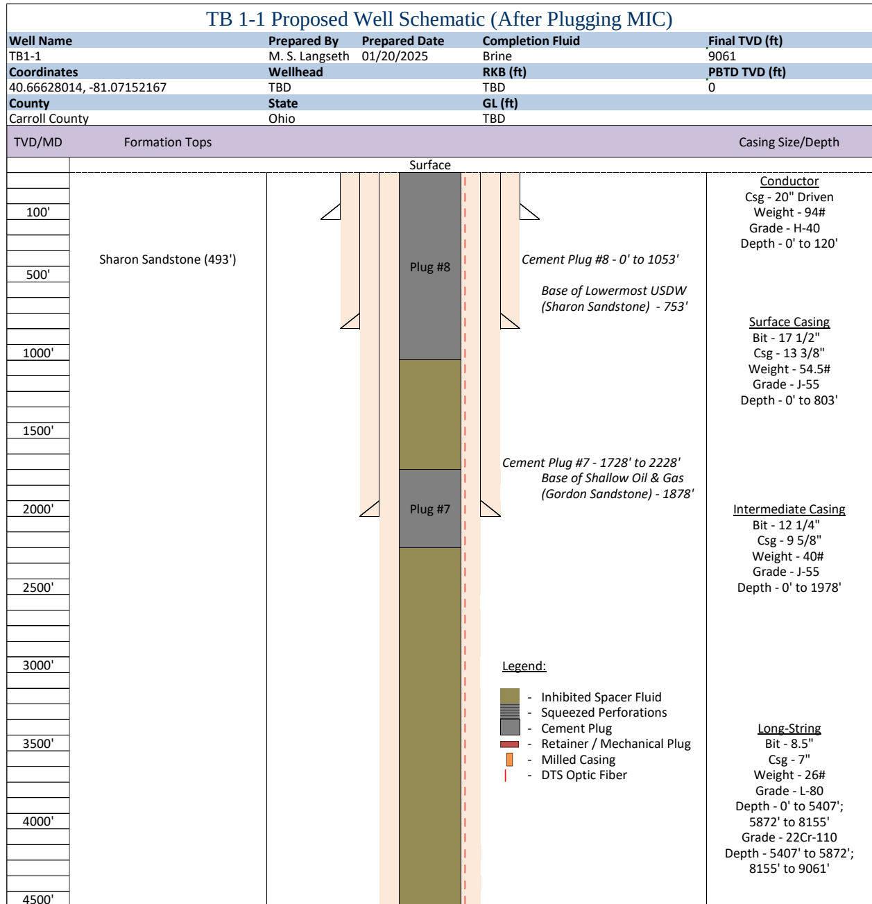
Figure 7: Proposed well schematic for TB1-1 after plugging the MIC to surface. Well schematic split in two for illustration purposes, 1/2: Surface to 4,500 ft.
