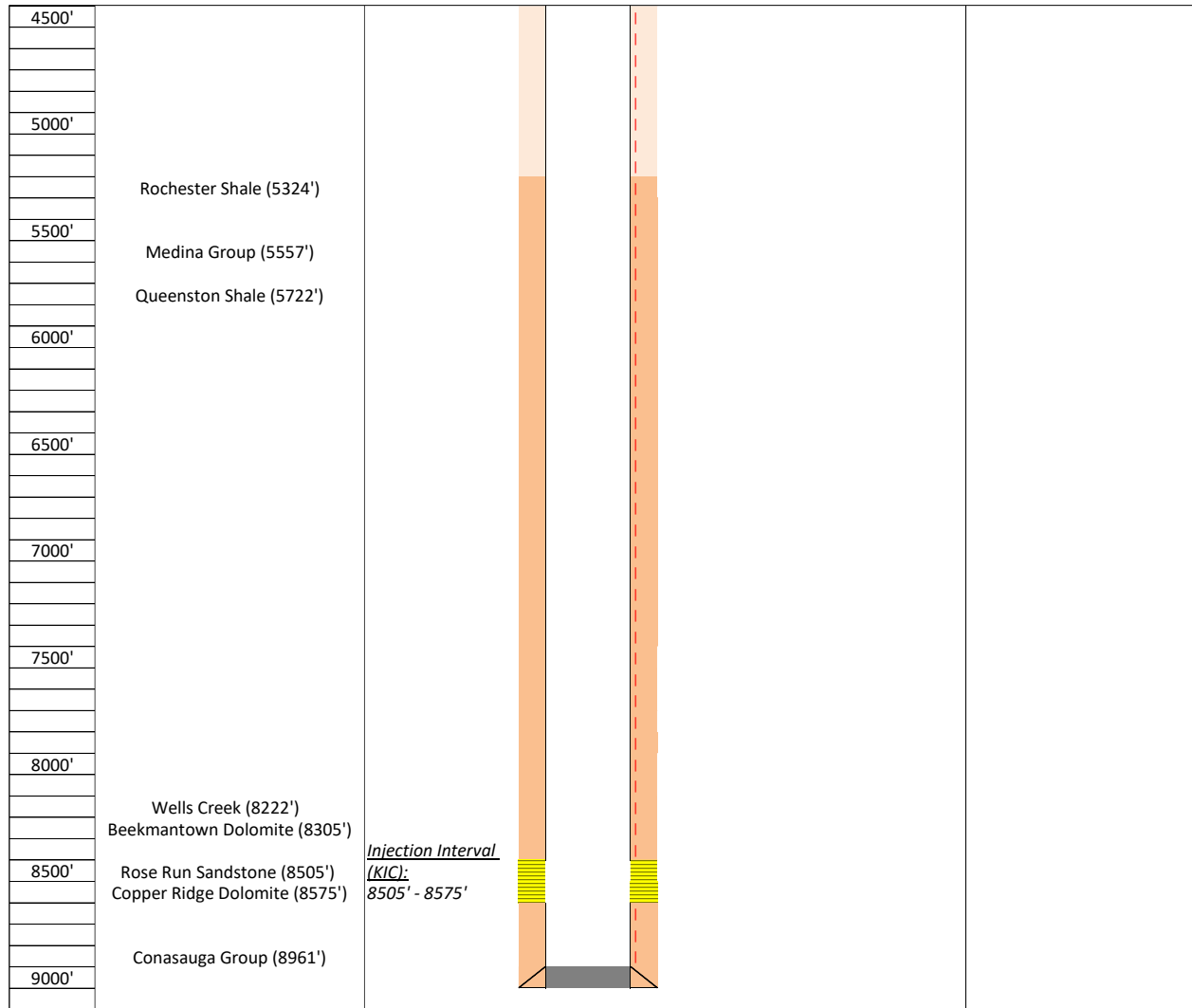
Figure 2: Proposed well schematic for TB1-1 after pulling the completion and before plugging the KIC. Well schematic split in two for illustration purposes, 2/2: 4,500 ft to 9,100 ft.
