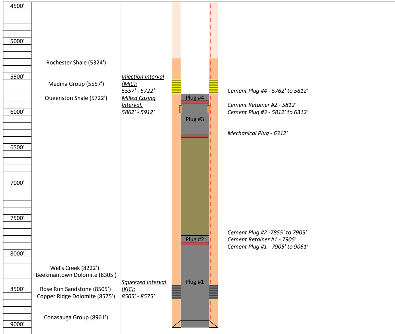
Figure 6: Proposed well schematic for TB1-1 after pulling the completion and before plugging the MIC. Well schematic split in two for illustration purposes, 2/2: 4,500 ft to 9,100 ft.
