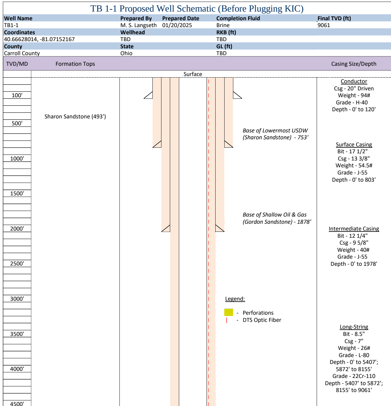
Figure 1: Proposed well schematic for TB1-1 after pulling the completion and before plugging the KIC. Well schematic split in two for illustration purposes, 1/2: Surface to 4,500 ft.
