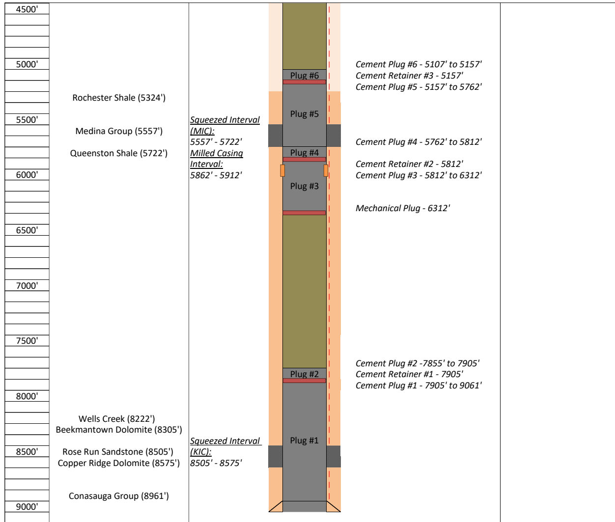
Figure 8: Proposed well schematic for TB1-1 after plugging the MIC to surface. Well schematic split in two for illustration purposes, 2/2: 4,500 ft to 9,100 ft.
