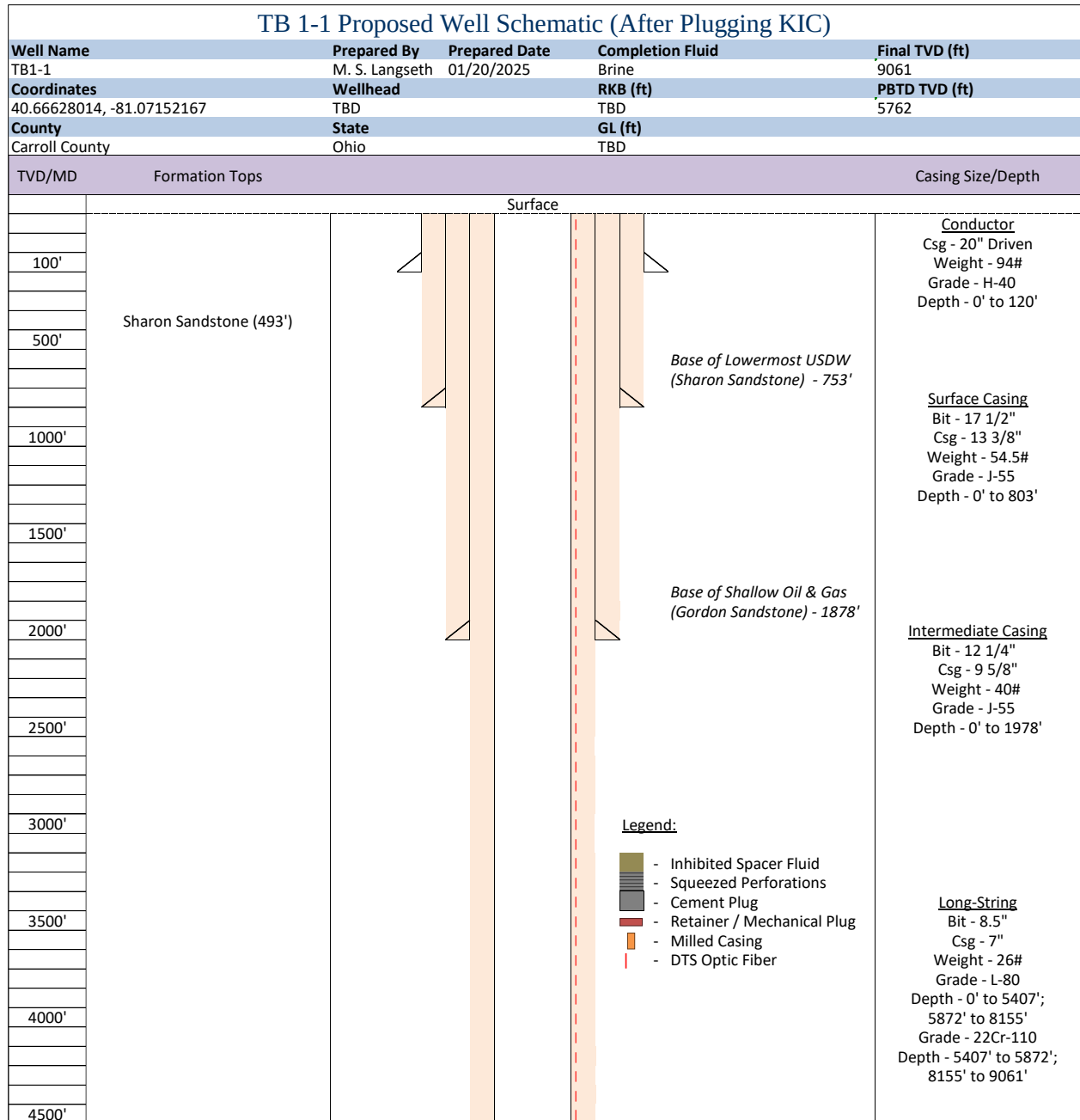
Figure 3: Proposed well schematic for TB1-1 after plugging from the KIC to the Queenston Shale (lower confining zone of MIC). Well schematic split in two for illustration purposes, 1/2: Surface to 4,500 ft.
