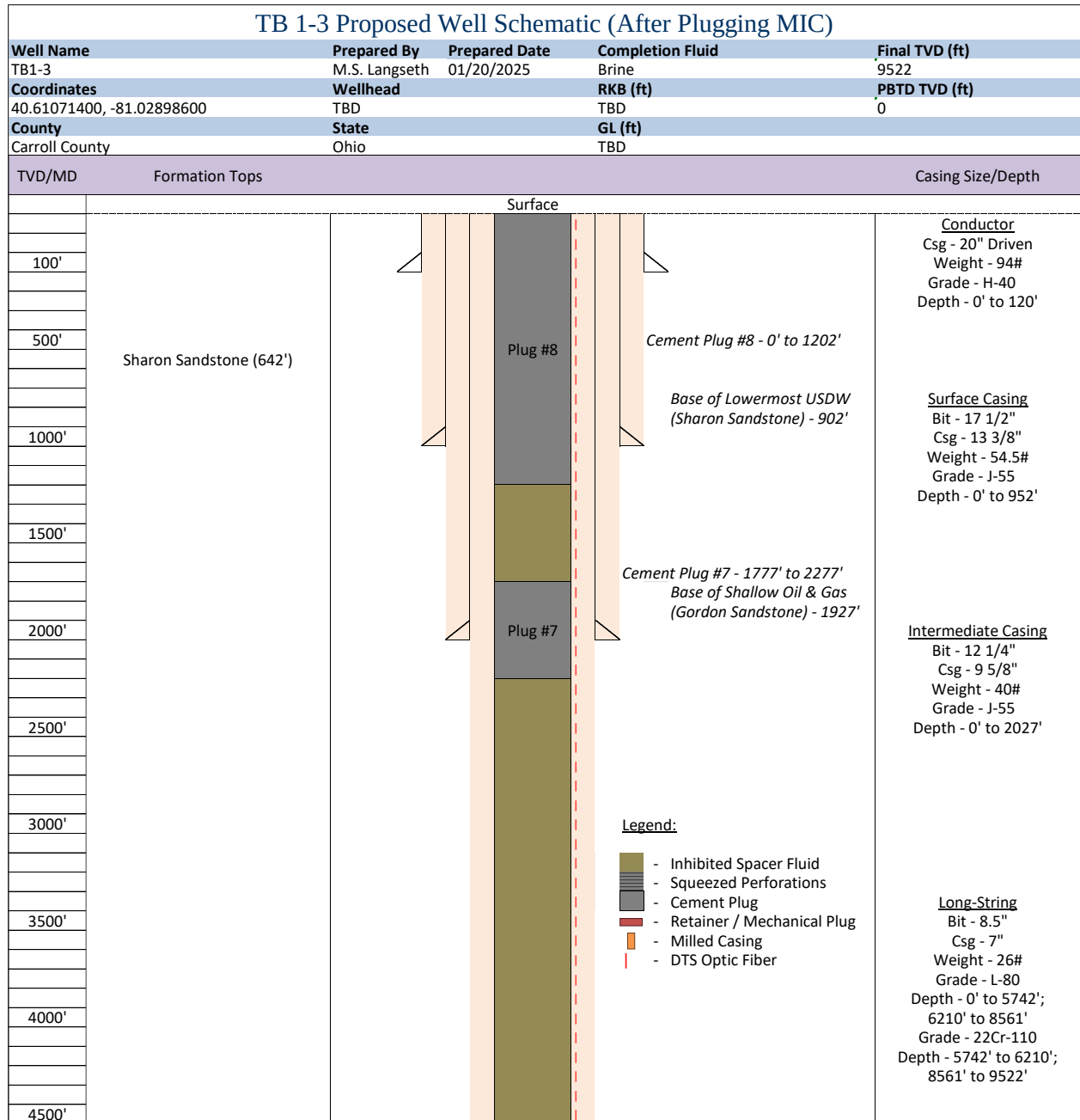
Figure 7: Proposed well schematic for TB1-3 after plugging the MIC to surface. Well schematic split in two for illustration purposes, 1/2: Surface to 4,500 ft.
