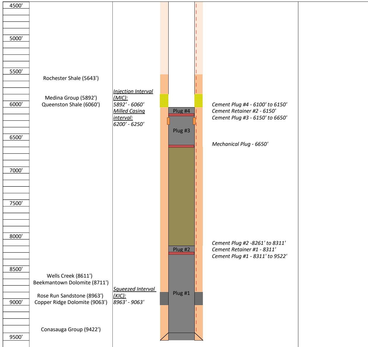
Figure 6: Proposed well schematic for TB1-3 after pulling the completion and before plugging the MIC. Well schematic split in two for illustration purposes, 2/2: 4,500 ft to 9,600 ft.
