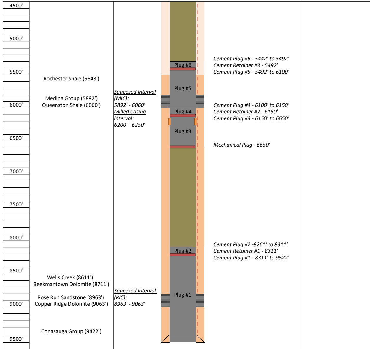
Figure 8: Proposed well schematic for TB1-3 after plugging the MIC to surface. Well schematic split in two for illustration purposes, 2/2: 4,500 ft to 9,600 ft.
