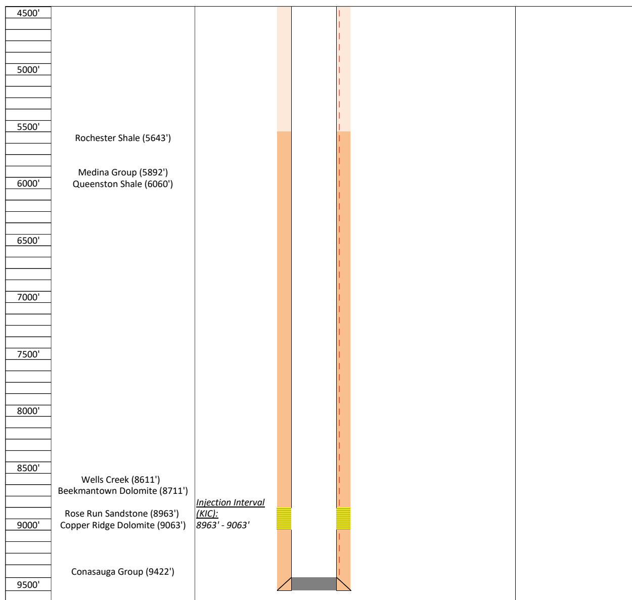
Figure 2: Proposed well schematic for TB1-3 after pulling the completion and before plugging the KIC. Well schematic split in two for illustration purposes, 2/2: 4,500 ft to 9,600 ft.
