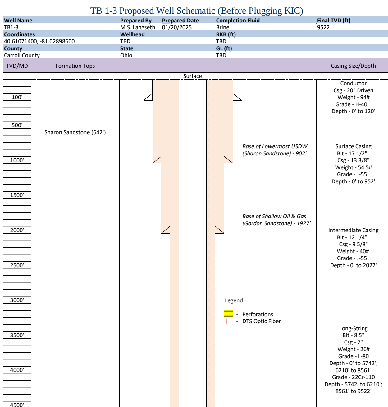
Figure 1: Proposed well schematic for TB1-3 after pulling the completion and before plugging the KIC. Well schematic split in two for illustration purposes, 1/2: Surface to 4,500 ft.
