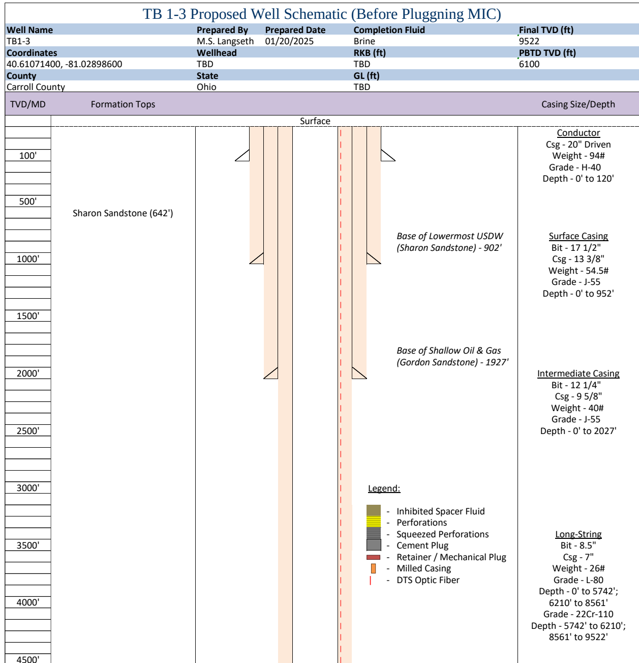
Figure 5: Proposed well schematic for TB1-3 after pulling the completion and before plugging the MIC. Well schematic split in two for illustration purposes, 1/2: Surface to 4,500 ft.
