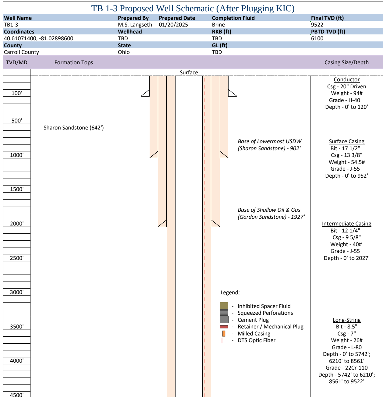
Figure 3: Proposed well schematic for TB1-3 after plugging from the KIC to the Queenston Shale (lower confining zone of MIC). Well schematic split in two for illustration purposes, 1/2: Surface to 4,500 ft.
