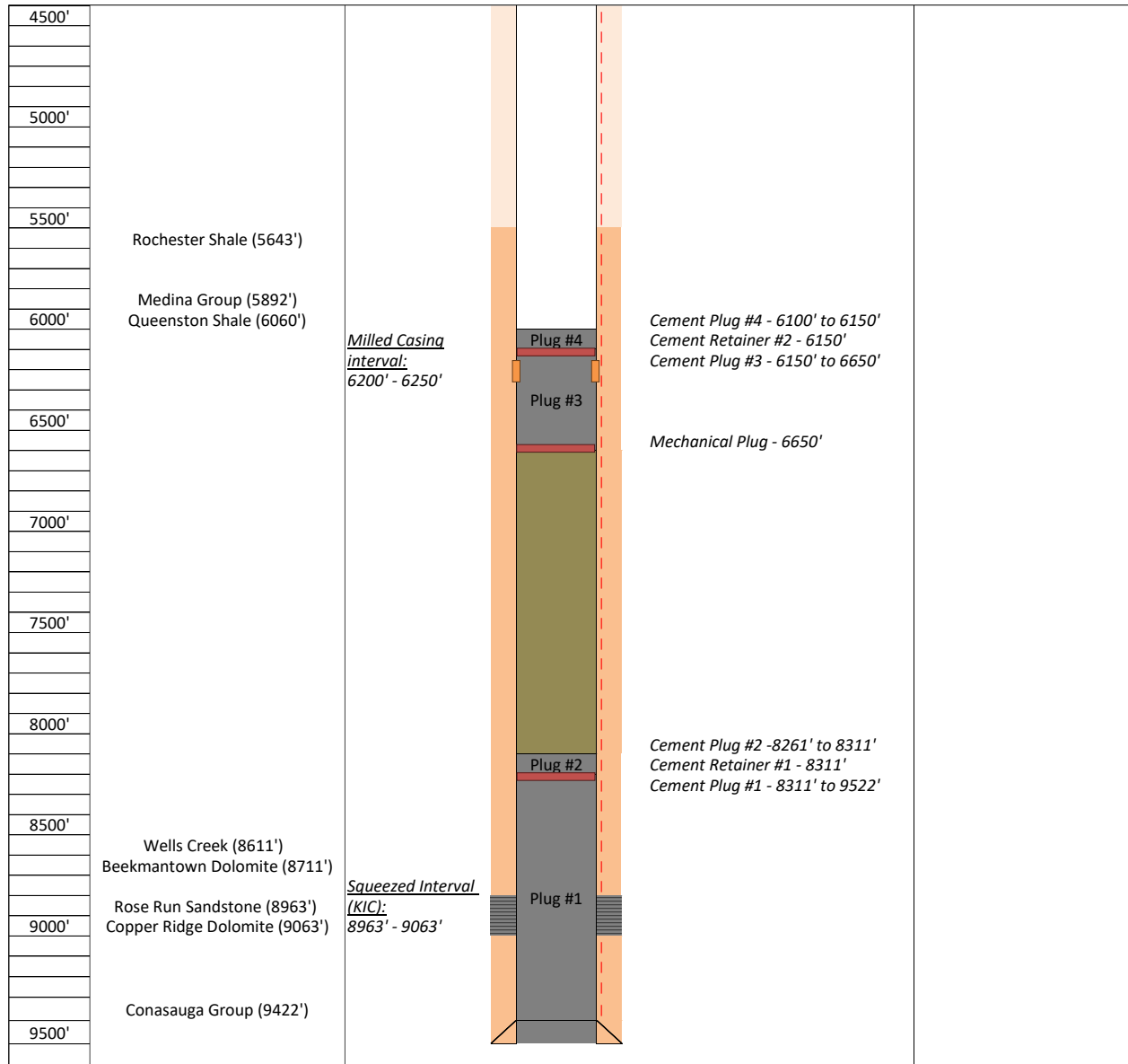
Figure 4: Proposed well schematic for TB1-3 after plugging from the KIC to the Queenston Shale (lower confining zone of MIC). Well schematic split in two for illustration purposes, 2/2: 4,500 ft to 9,600 ft.
