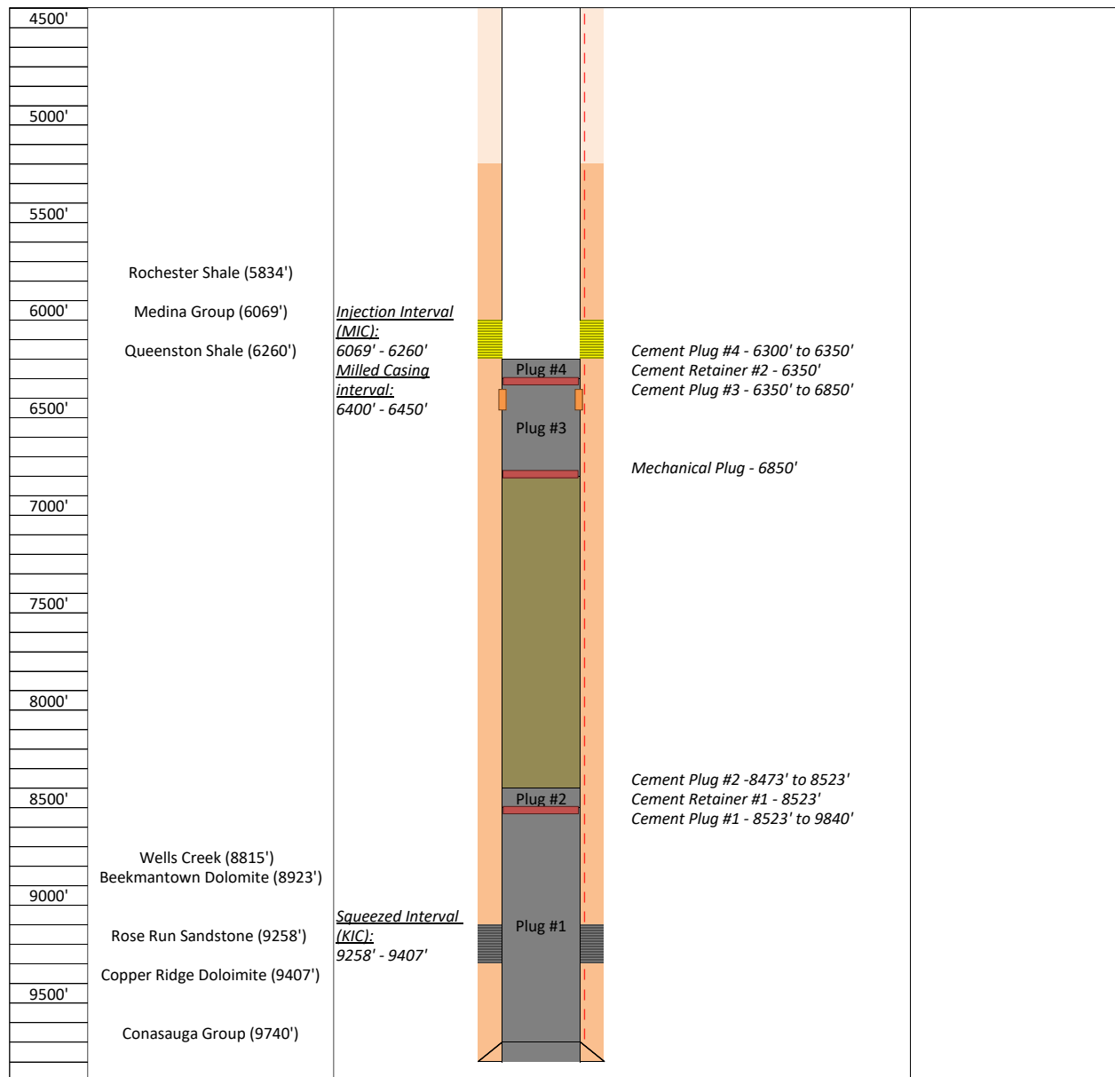
Figure 6: Proposed well schematic for TB1-4 after pulling the completion and before plugging the MIC. Well schematic split in two for illustration purposes, 2/2: 4,500 ft to 9,900 ft.
