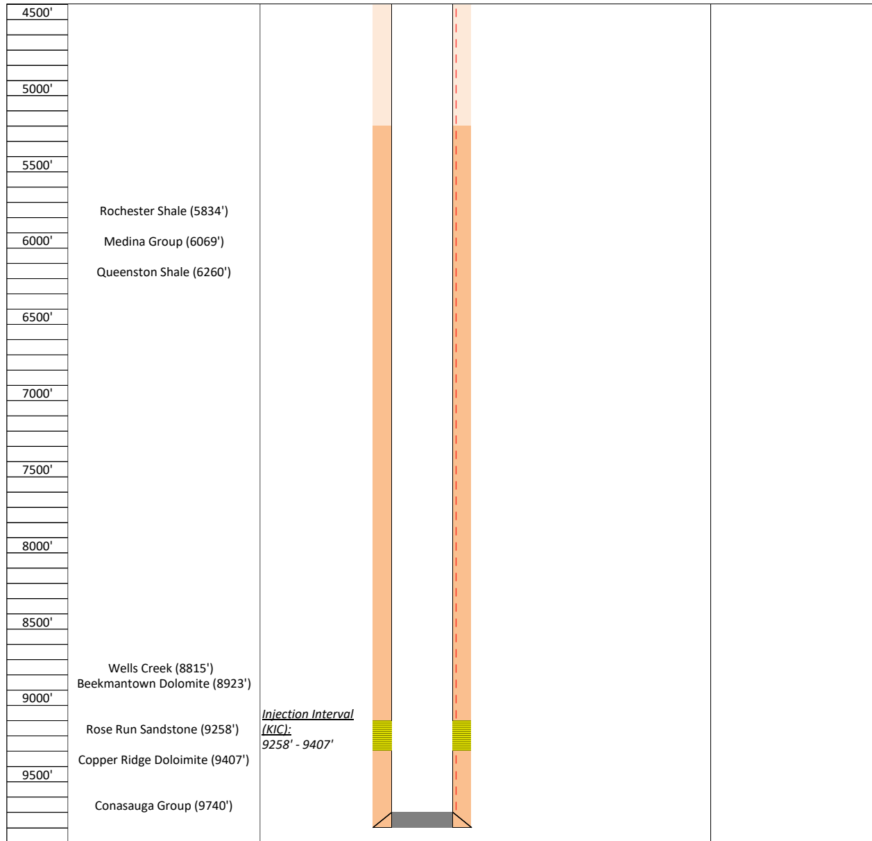
Figure 2: Proposed well schematic for TB1-4 after pulling the completion and before plugging the KIC. Well schematic split in two for illustration purposes, 2/2: 4,500 ft to 9,900 ft.
