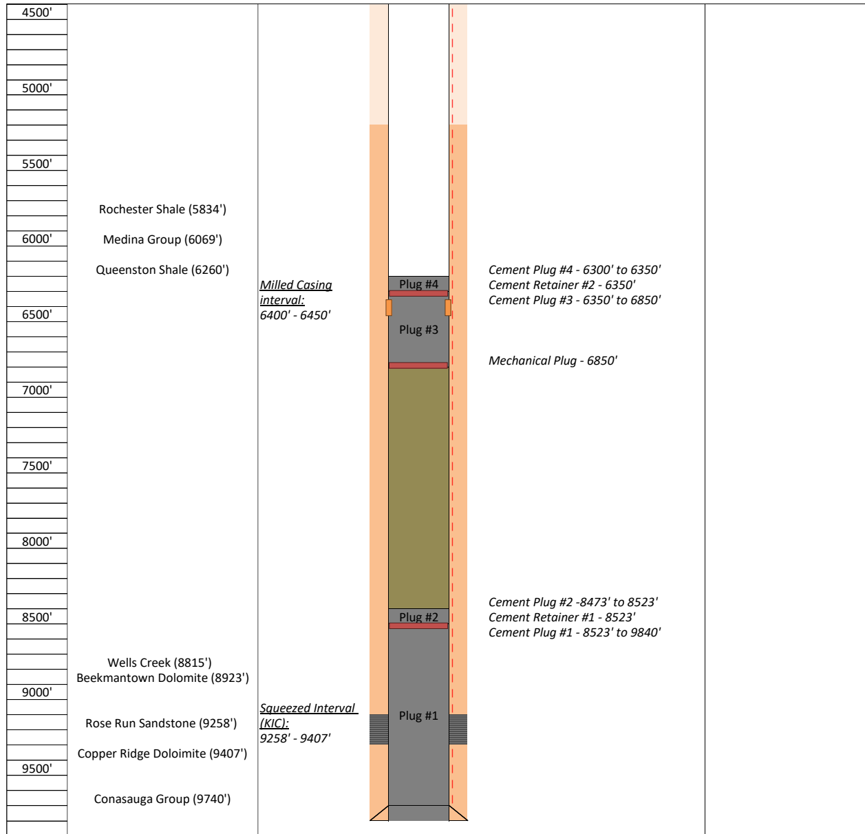
Figure 4: Proposed well schematic for TB1-4 after plugging from the KIC to the Queenston Shale (lower confining zone of the MIC). Well schematic split in two for illustration purposes, 2/2: 4,500 ft to 9,900 ft.
