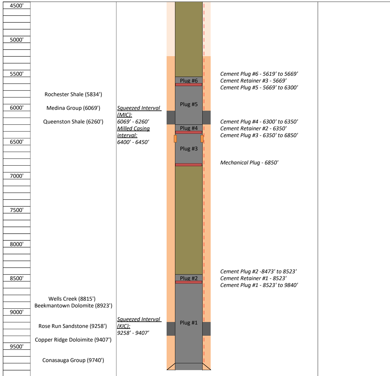
Figure 8: Proposed well schematic for TB1-4 after plugging the MIC to surface. Well schematic split in two for illustration purposes, 2/2: 4,500 ft to 9,900 ft.
