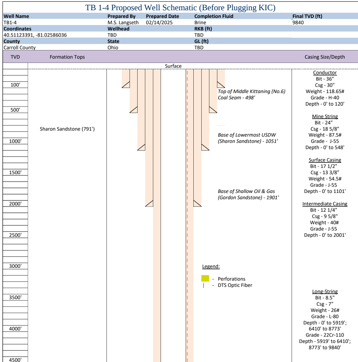
Figure 1: Proposed well schematic for TB1-4 after pulling the completion and before plugging the KIC. Well schematic split in two for illustration purposes, 1/2: Surface to 4,500 ft.
