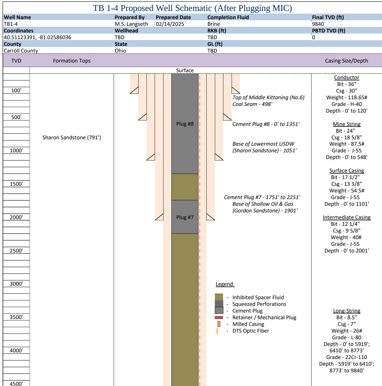
Figure 7: Proposed well schematic for TB1-4 after plugging the MIC to surface. Well schematic split in two for illustration purposes, 1/2: Surface to 4,500 ft.
