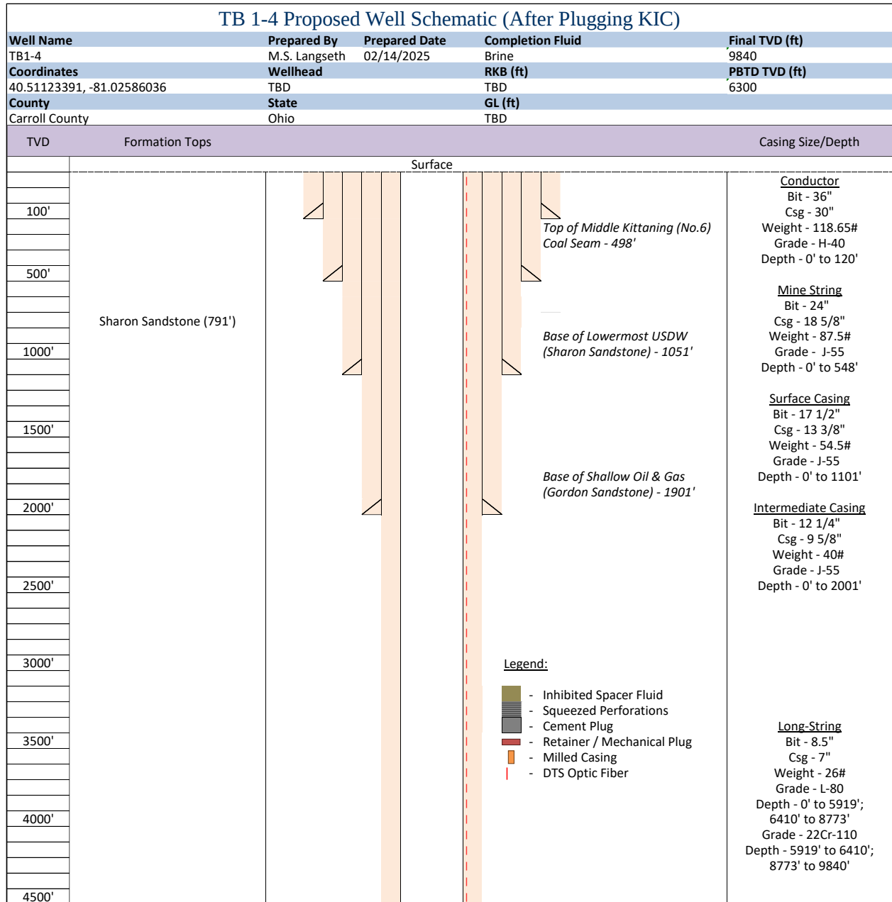
Figure 3: Proposed well schematic for TB1-4 after plugging from the KIC to the Queenston Shale (lower confining zone of MIC). Well schematic split in two for illustration purposes, 1/2: Surface to 4,500 ft.
