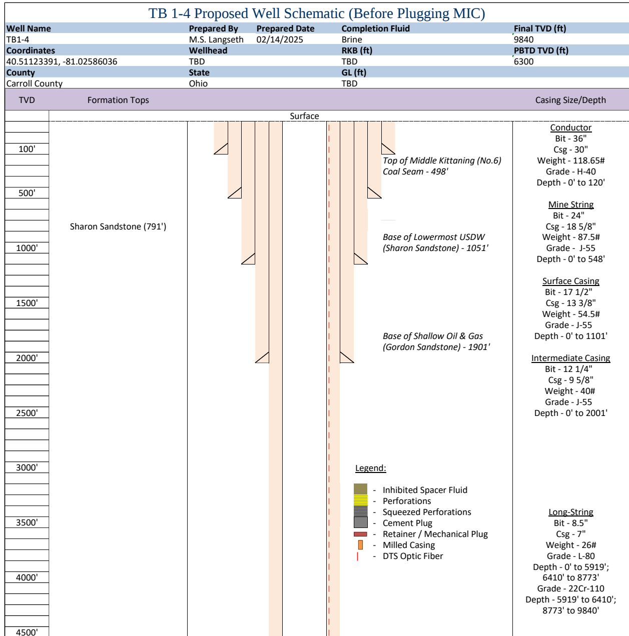
Figure 5: Proposed well schematic for TB1-4 after pulling the completion and before plugging the MIC. Well schematic split in two for illustration purposes, 1/2: Surface to 4,500 ft.
