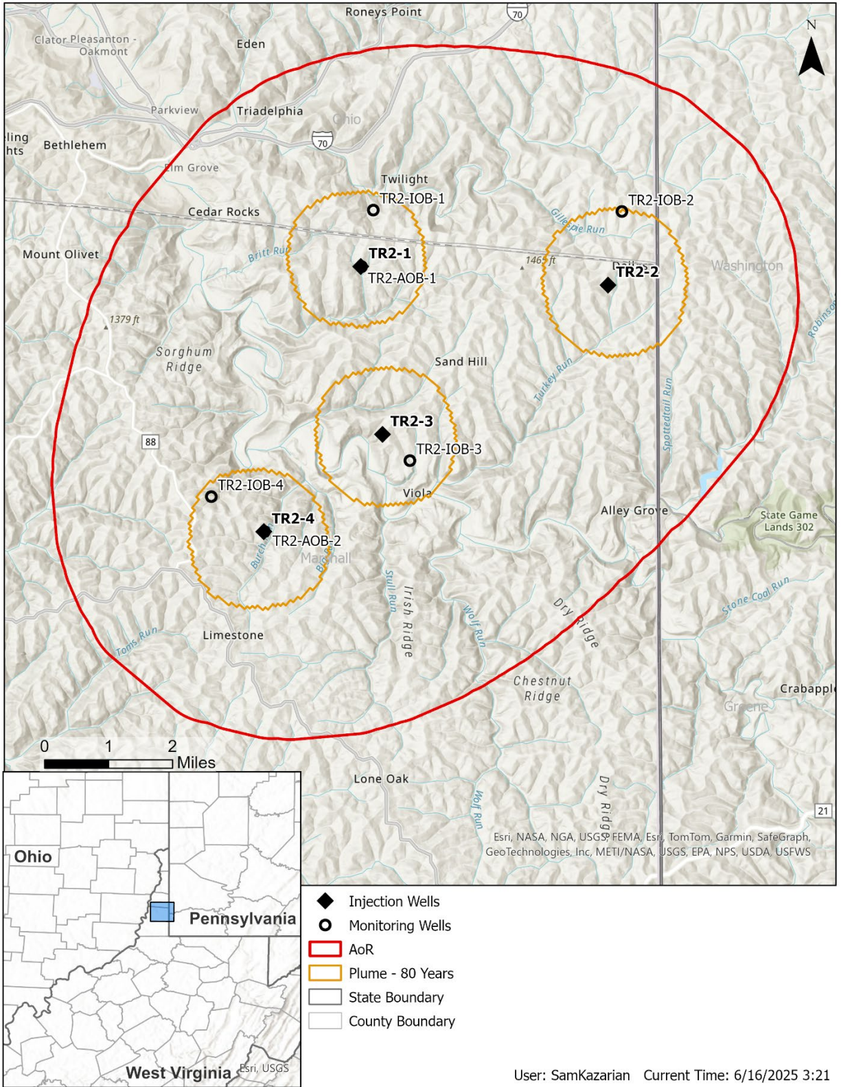
Figure 1: Locations of proposed injection and observation wells at Tri-State CCS Redbud 2.
