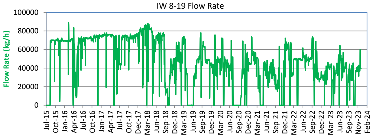
Figure 3-2: Injection Rate History for IW 8-19
