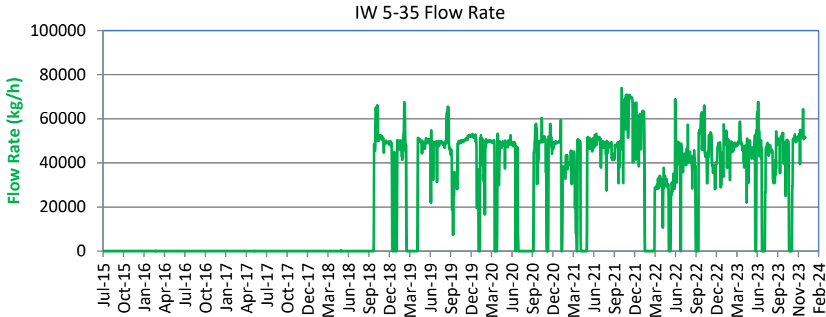
Figure 3-3: Injection Rate History for IW 5-35
