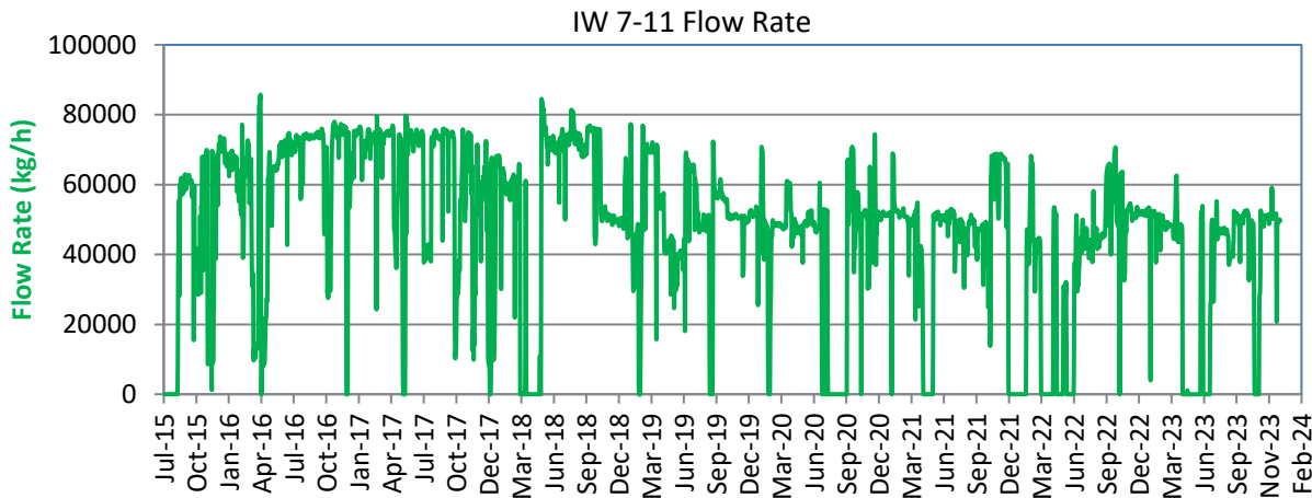
Figure 3-1: Injection Rate History for IW 7-11
