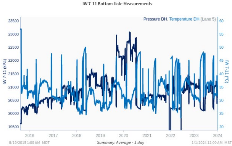
Figure 4-1: IW 7-11 Bottom Hole Measurements
