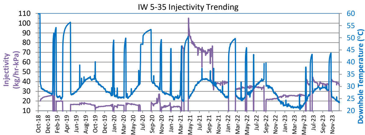
Figure 3-6: Injectivity Index and BHT for 5-35 over time
