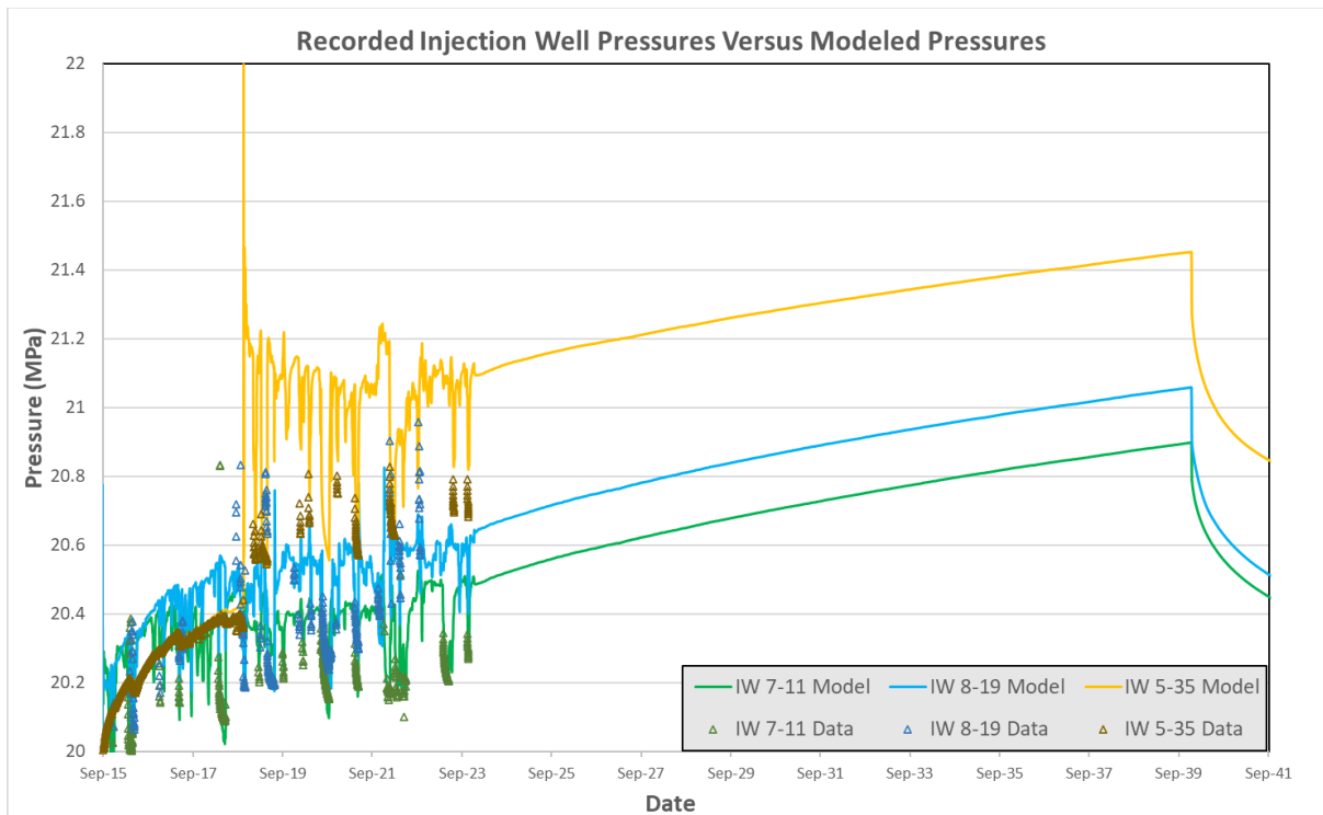
Figure 3-8: Well by well Modelled Pressure Forecast
