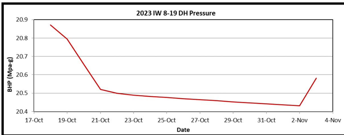
Figure 3-10: IW 8-19 pressure fall-off and stabilization in Q4 2023
