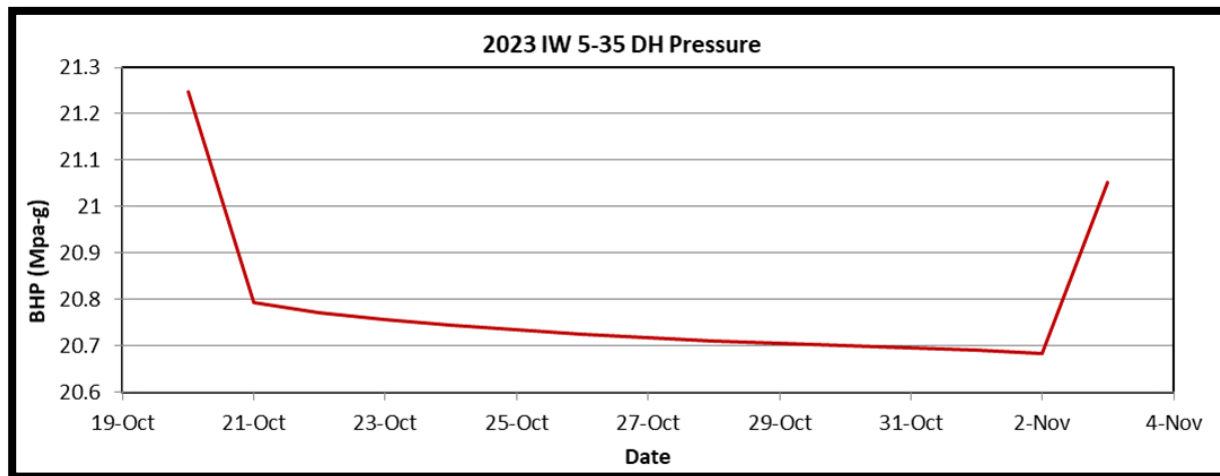
Figure 3-11: IW 5-35 pressure fall-off and stabilization in Q4 2023
