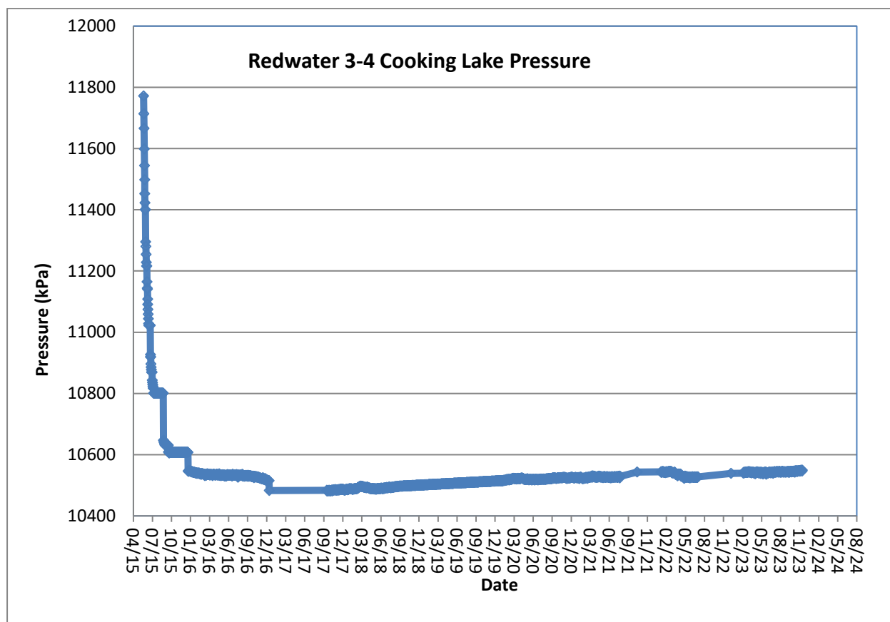
Figure 4-5: Quest Observation well 3-4 pressure history
