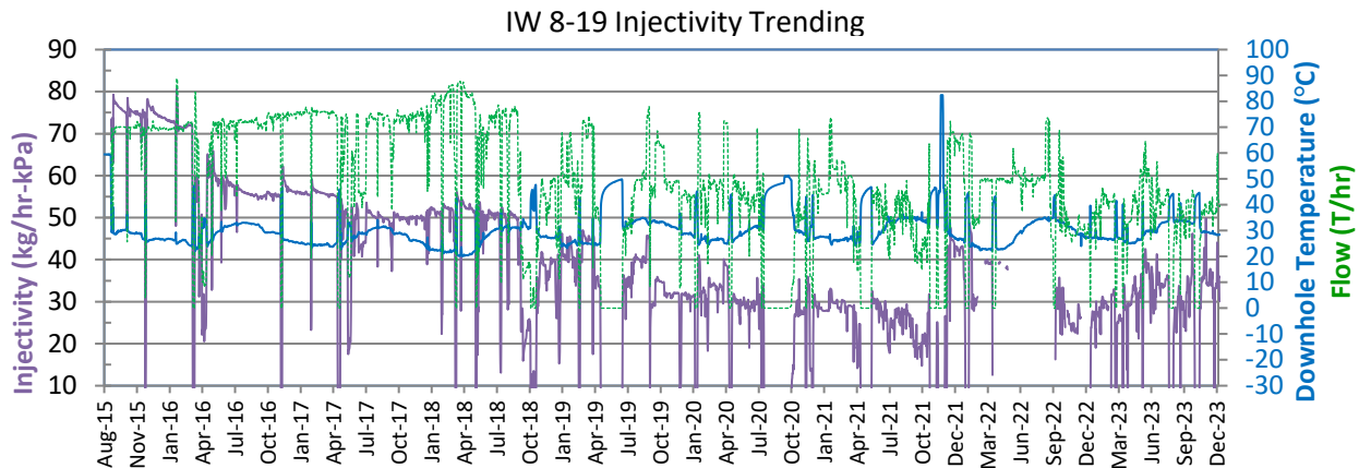
Figure 3-5: Injectivity Index and BHT for 8-19 over time. Flow rate also plotted to show rate dependency of Injectivity throughout injection history
