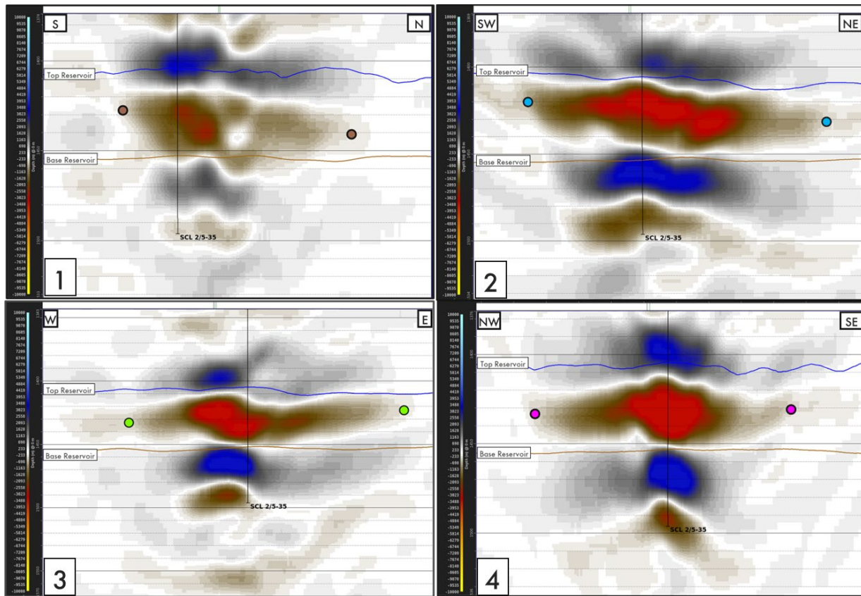
Figure 4-20: 2DVSP quadrature difference volumes, interpreted edge of plume indicated. See Figure 4-21 for map view
