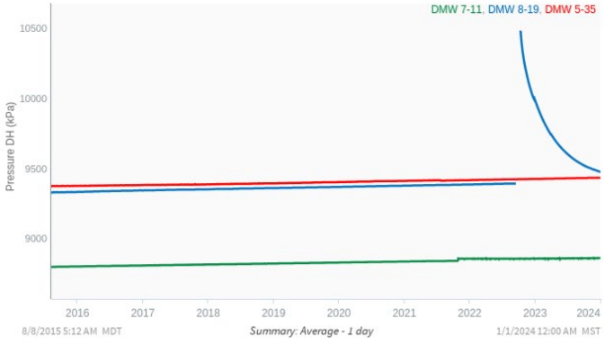
Figure 4-4: Quest deep monitoring well pressure history; (Note: 'steps' in trends mark new gauge installations)
