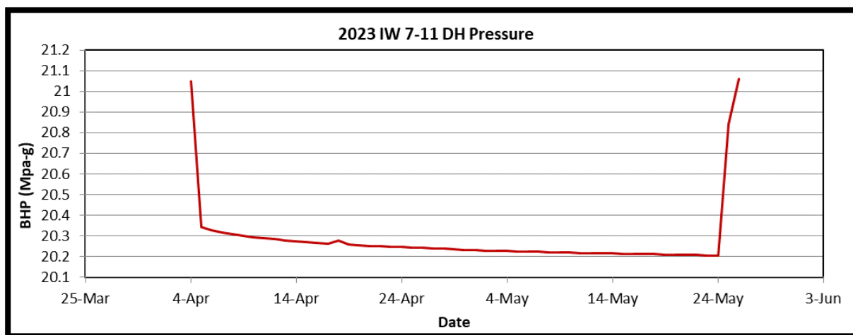
Figure 3-9: IW 7-11 pressure fall-off and stabilization in Q2 2023
