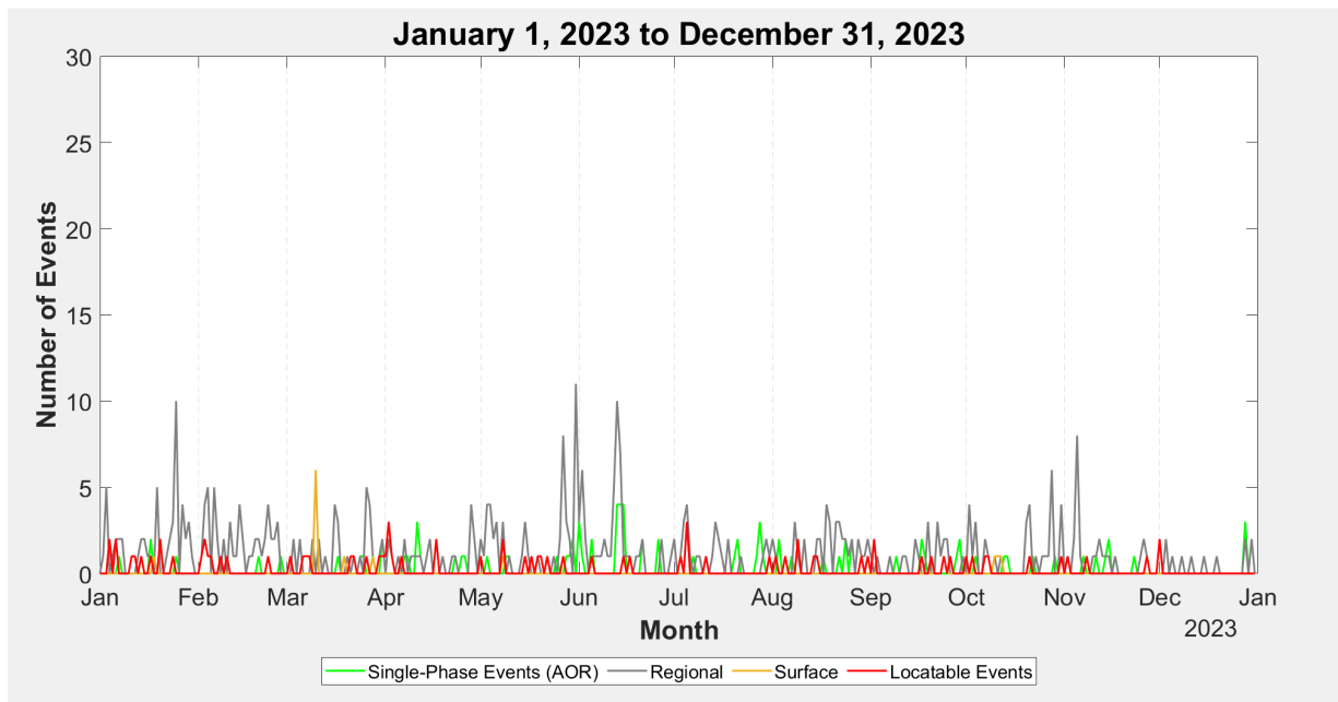
Figure 4-9: Daily event counts of seismicity categorized events in 2023. “Regional” events include locatable regional, single phase regional and potential regional events as defined in Table 4-3
