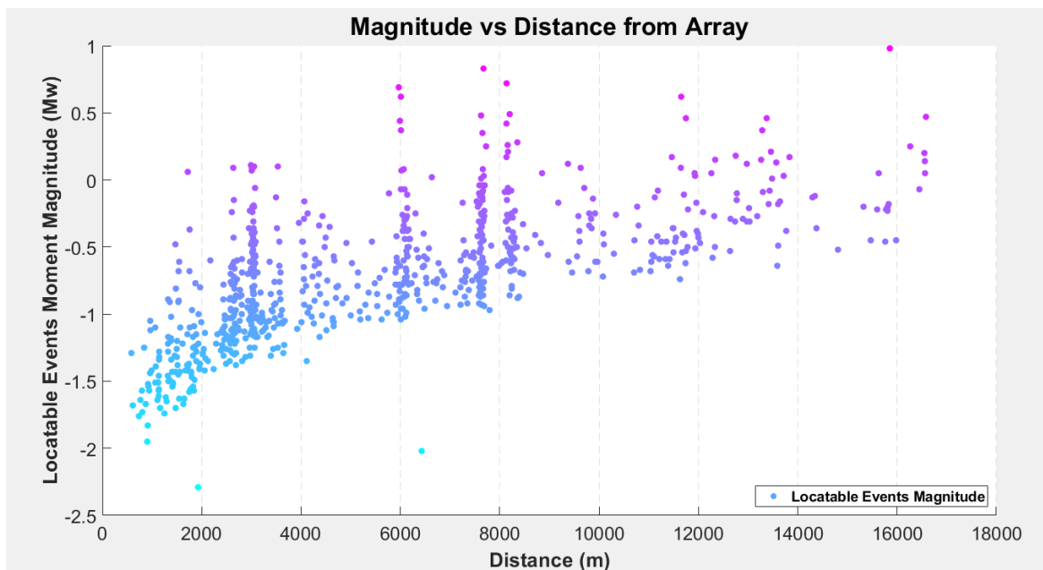
Figure 4-15: Locatable Event moment magnitude ( M_w ) vs Distance from array [m], recorded from November 2014 to December 31 st , 2023. All Locatable Events are coloured by moment magnitude. Increased monitoring distance impacts the ability to identify smaller magnitude events
