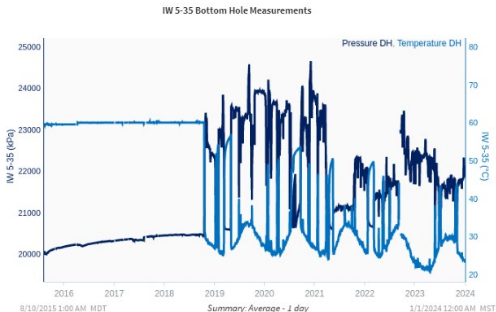
Figure 4-3: IW 5-35 Bottom Hole Measurements
