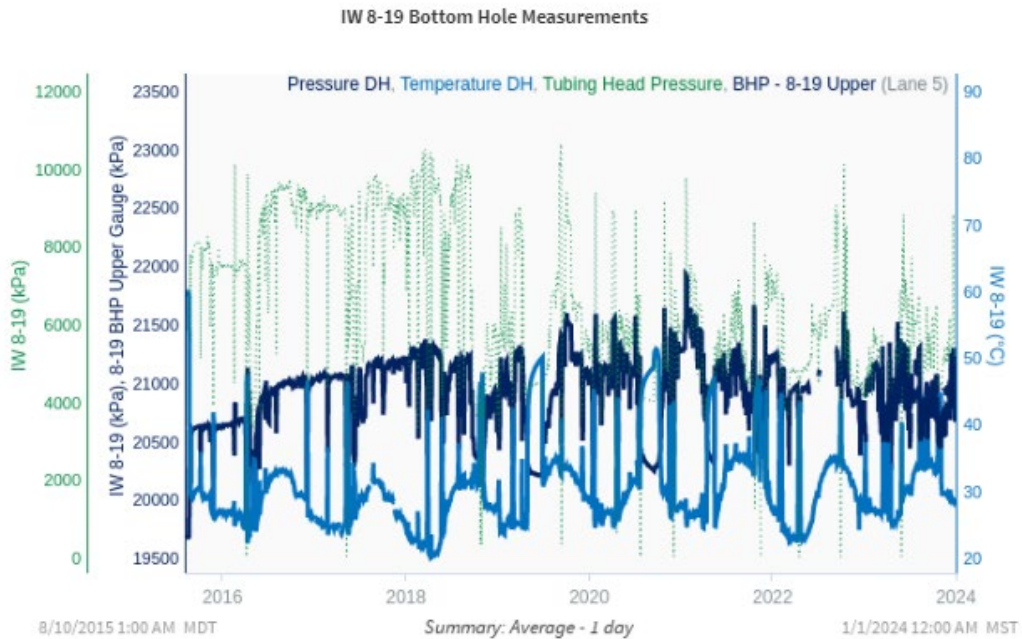
Figure 4-2: IW 8-19 Bottom Hole Measurements – Tubing Head Pressure added to demonstrate containment where there are gaps in DH Pressure measurement
