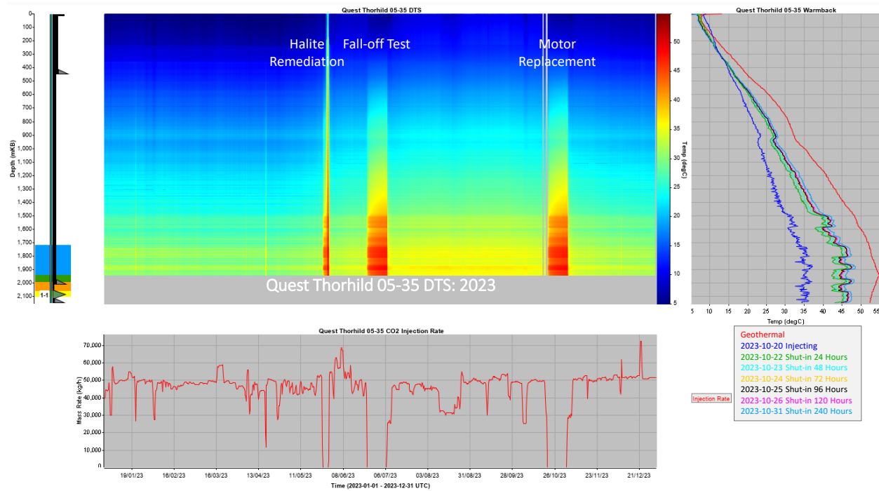
Figure 4-19: Injection well 5-35 DTS data. The heatmap shows DTS data collected during 2023 with a temperature scale from 5° to 55°C. The graph on the right shows individual traces for the warmback analysis from the motor replacement period. The graph at the bottom shows the CO 2 injection rate in [kg/h].
