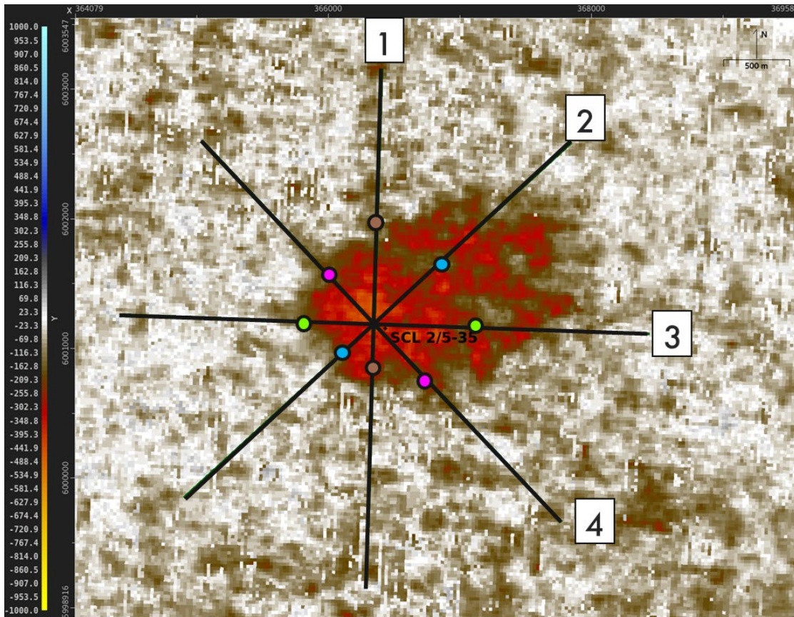
Figure 4-21: Map view of plume edge interpretation on 2DVSP underlain by surface seismic time-lapse response
