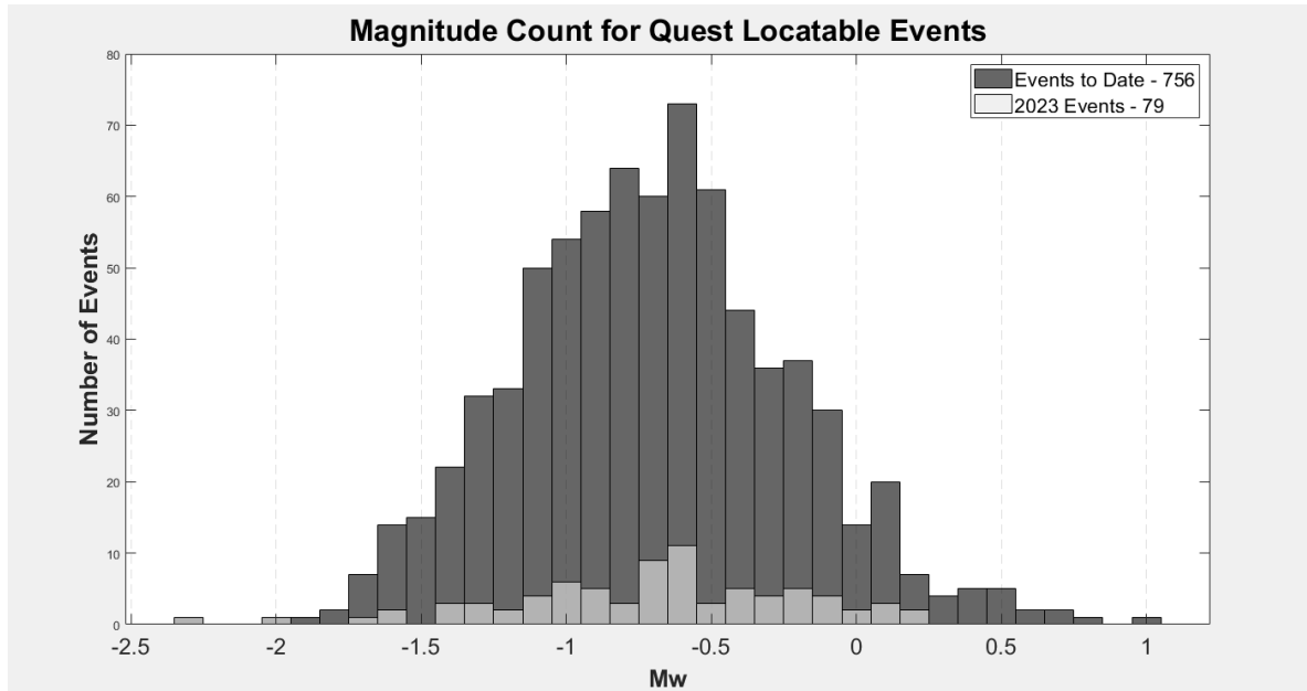
Figure 4-12: Histogram of moment magnitude ( M_w ) of Locatable Events 2015 - 2023; 756 Locatable Events. Overlay of 2023 Locatable Events; 79 Locatable Events
