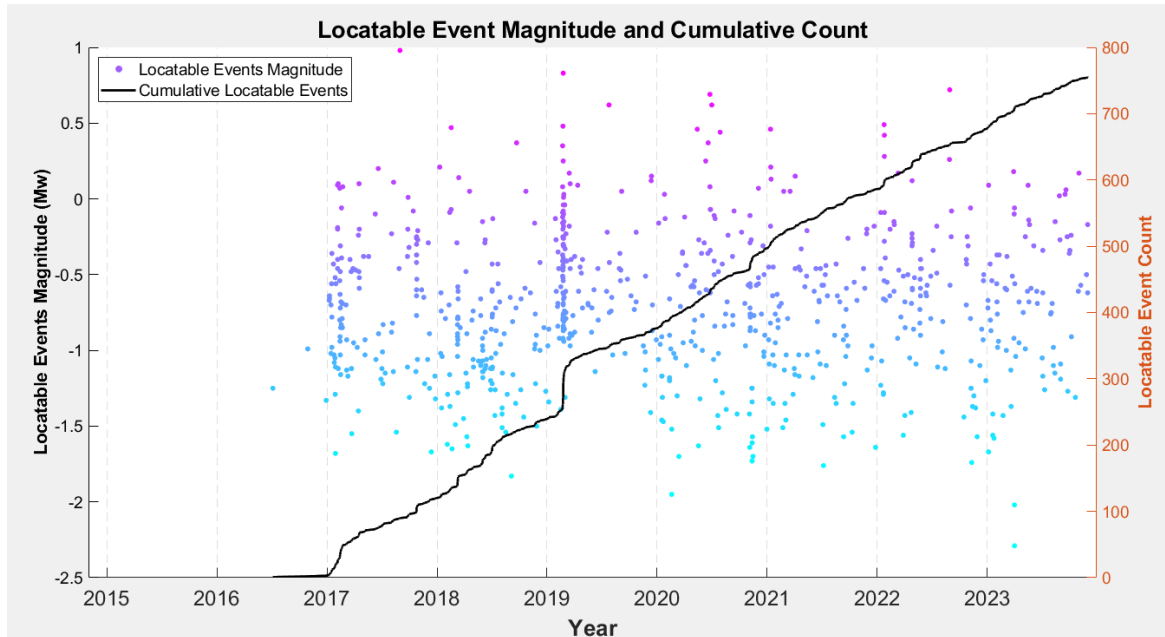
Figure 4-14: All Locatable Events recorded from November 2014 to December 31 st , 2023 are plotted and coloured by moment magnitude ( M_w ). The black curve is the cumulative count of Locatable Events
