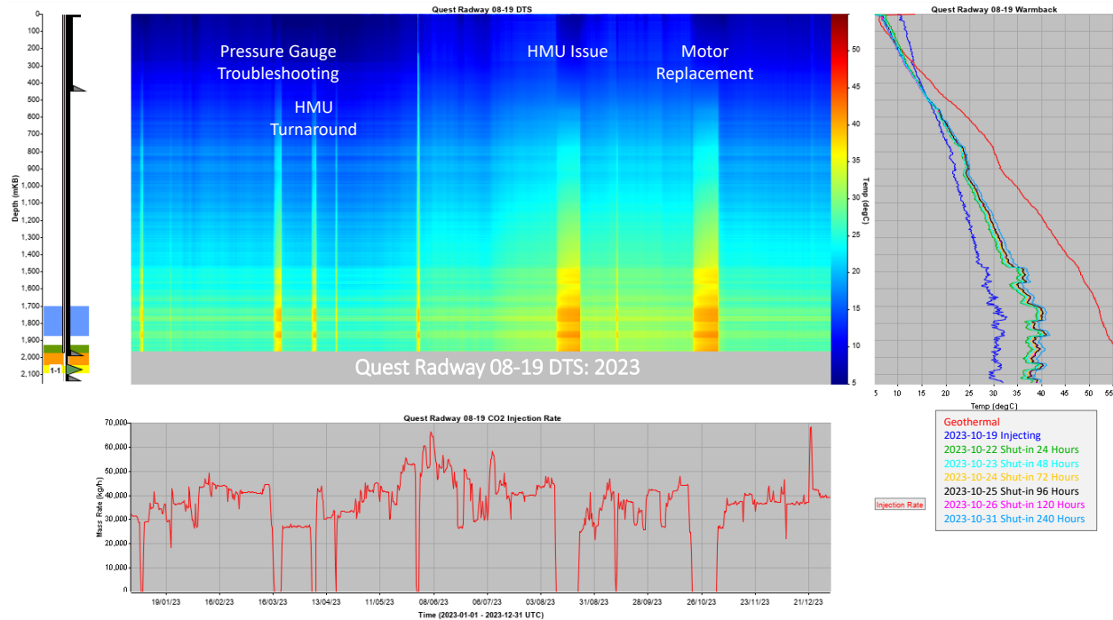
Figure 4-17: Injection well 8-19 DTS data. The heatmap shows DTS data collected during 2023 with a temperature scale from 5° to 55°C. The graph on the right shows individual traces for the warmback analysis from the motor replacement period. The graph at the bottom shows the CO 2 injection rate in [kg/h].
