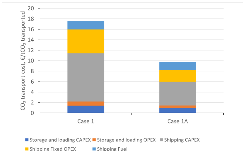
Figure 13 Effect of pressure on CO 2 transport cost. Case 1: CO 2 transport at 15 barg; Case 1A: CO 2 transport at 7 barg.
