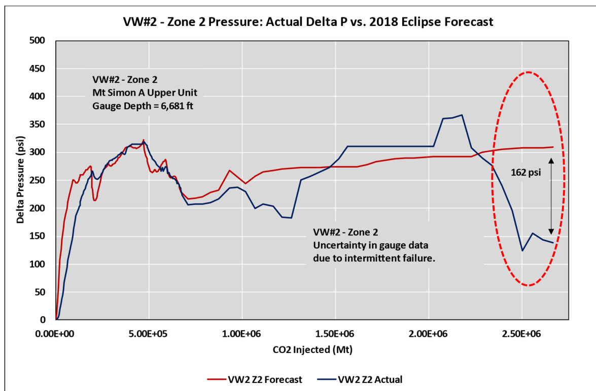
Figure 14: VW#2 Zone 2 actual reservoir differential pressure versus 2018 Eclipse forecast.
