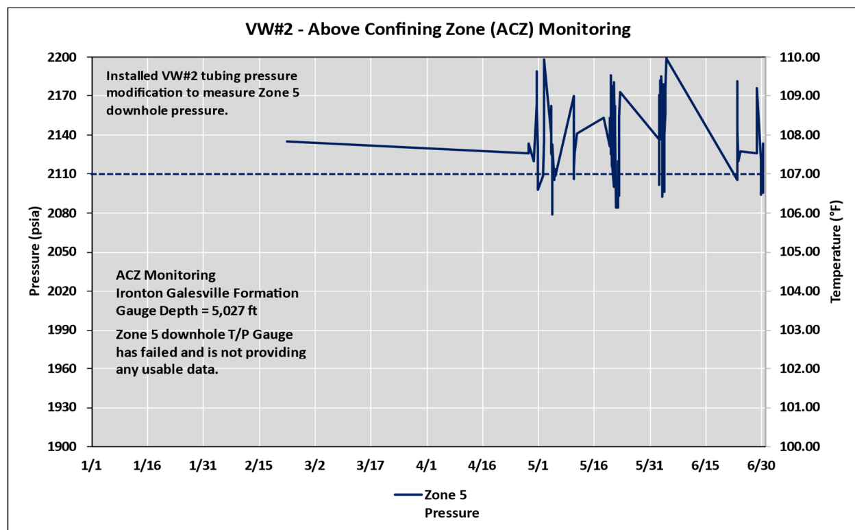
Figure 6: VW#2 ACZ monitoring of the Ironton Galesville Formation for Jan-Jun 2022.
