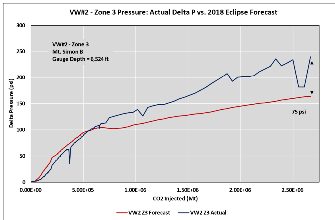
Figure 15: VW#2 Zone 3 actual reservoir differential pressure versus 2018 Eclipse forecast.
