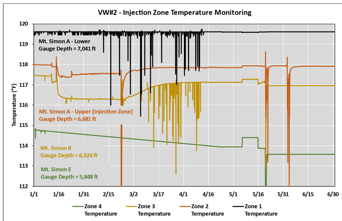
Figure 18: VW#2 injection zone temperature monitoring data for Jan-Jun 2022.
