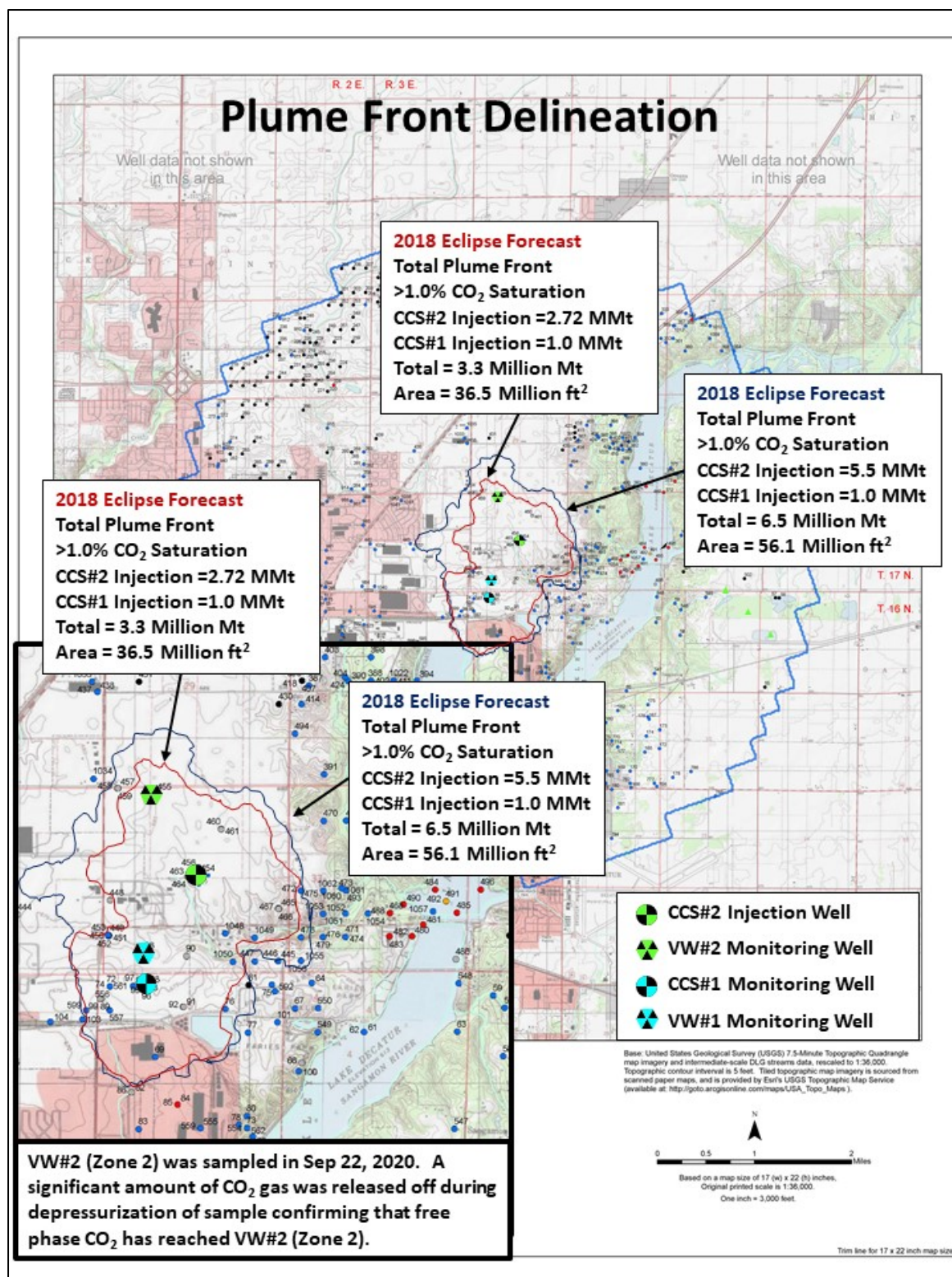
Figure 25: 2018 Eclipse model's plume front delineation for June 30, 2022 and after the total injection of 6.5 million Mt (CCS#1=1.0 million Mt and CCS#2=5.5 million Mt).
