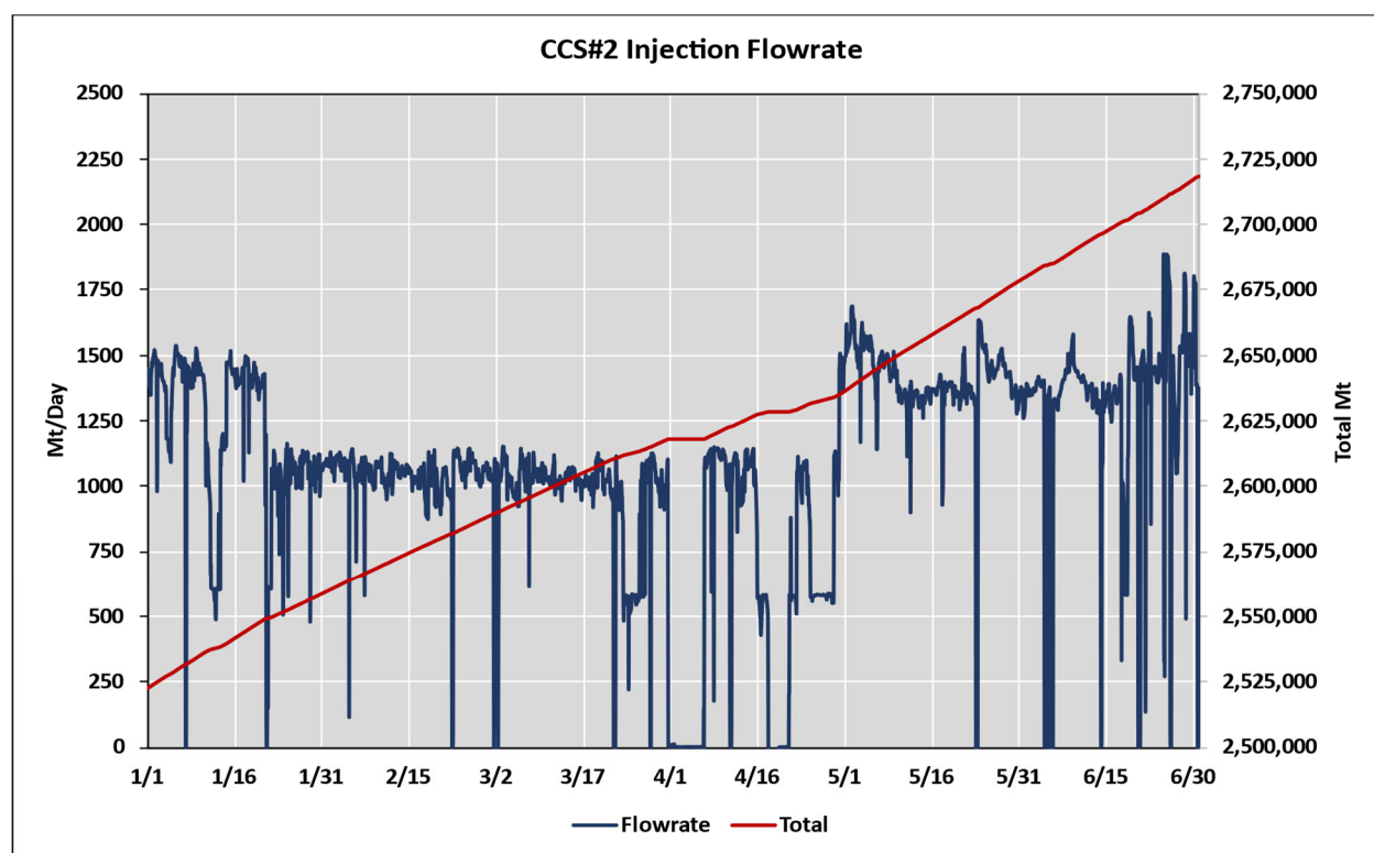
Figure 1: CCS#2 - Injection rate monitoring data for Jan-Jun 2022.
