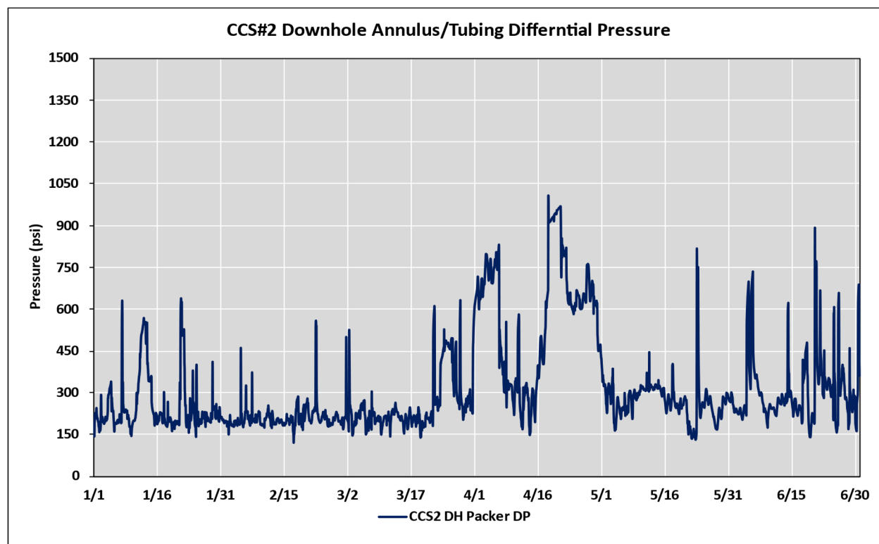
Figure 5: CCS#2 downhole annulus and tubing differential pressure monitoring data for Jan-Jun 2022.
