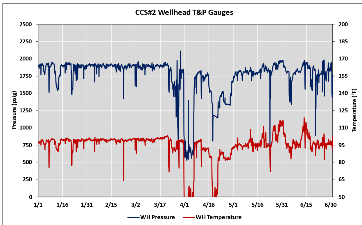
Figure 2: CCS#2 wellhead temperature and pressure monitoring data for Jan-Jun 2022.
