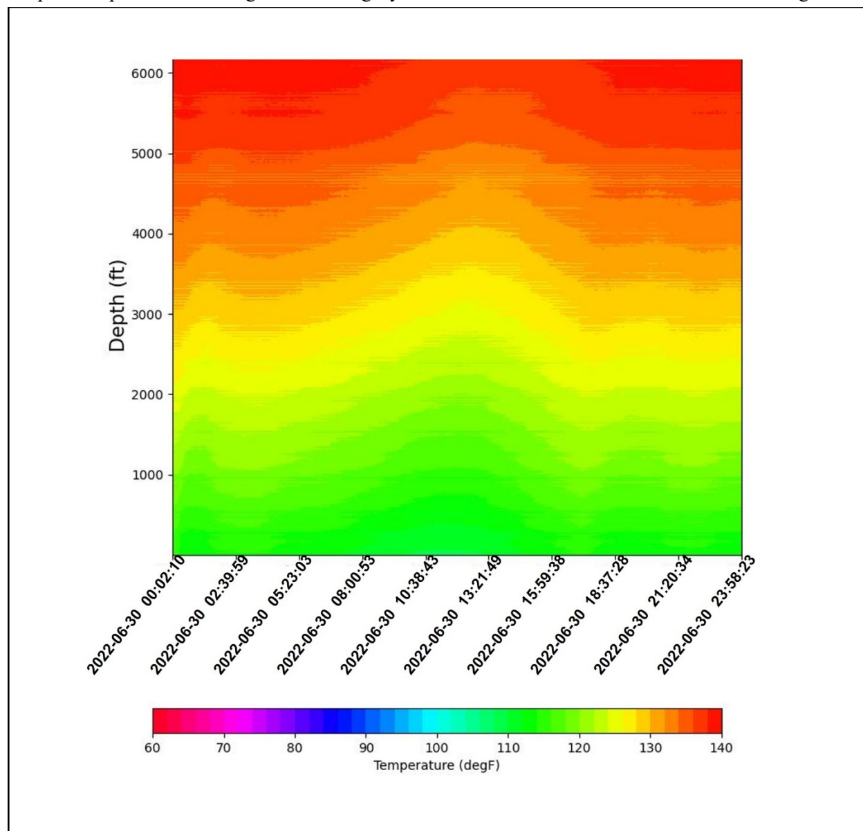
Figure 9: CCS#2 DTS data in 3-dimensional view for last day of reporting period 06/30/2022.
