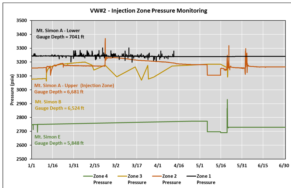
Figure 17: VW#2 injection zone pressure monitoring data for Jan-Jun 2022.
