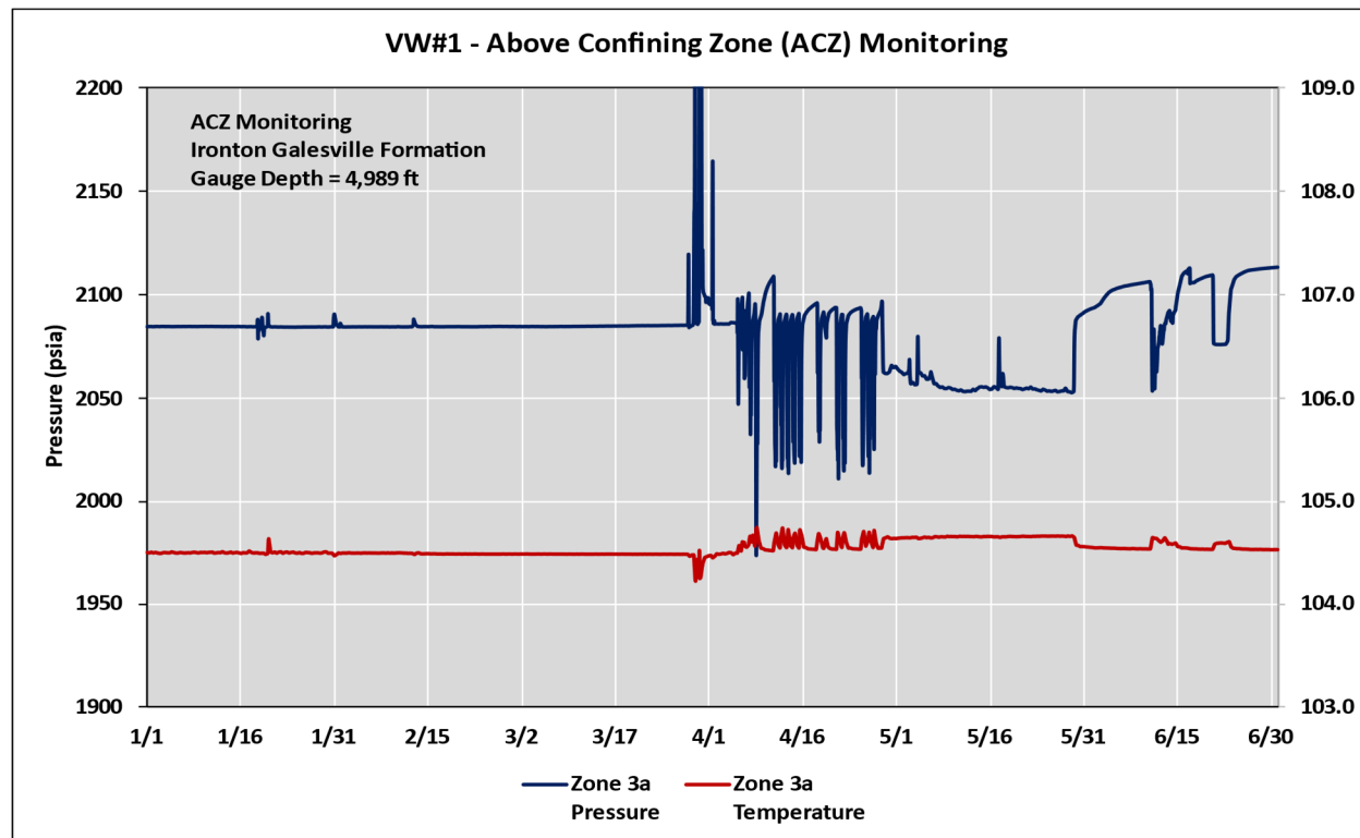
Figure 7: VW#1 ACZ monitoring of the Ironton Galesville Formation for Jan-Jun 2022.
