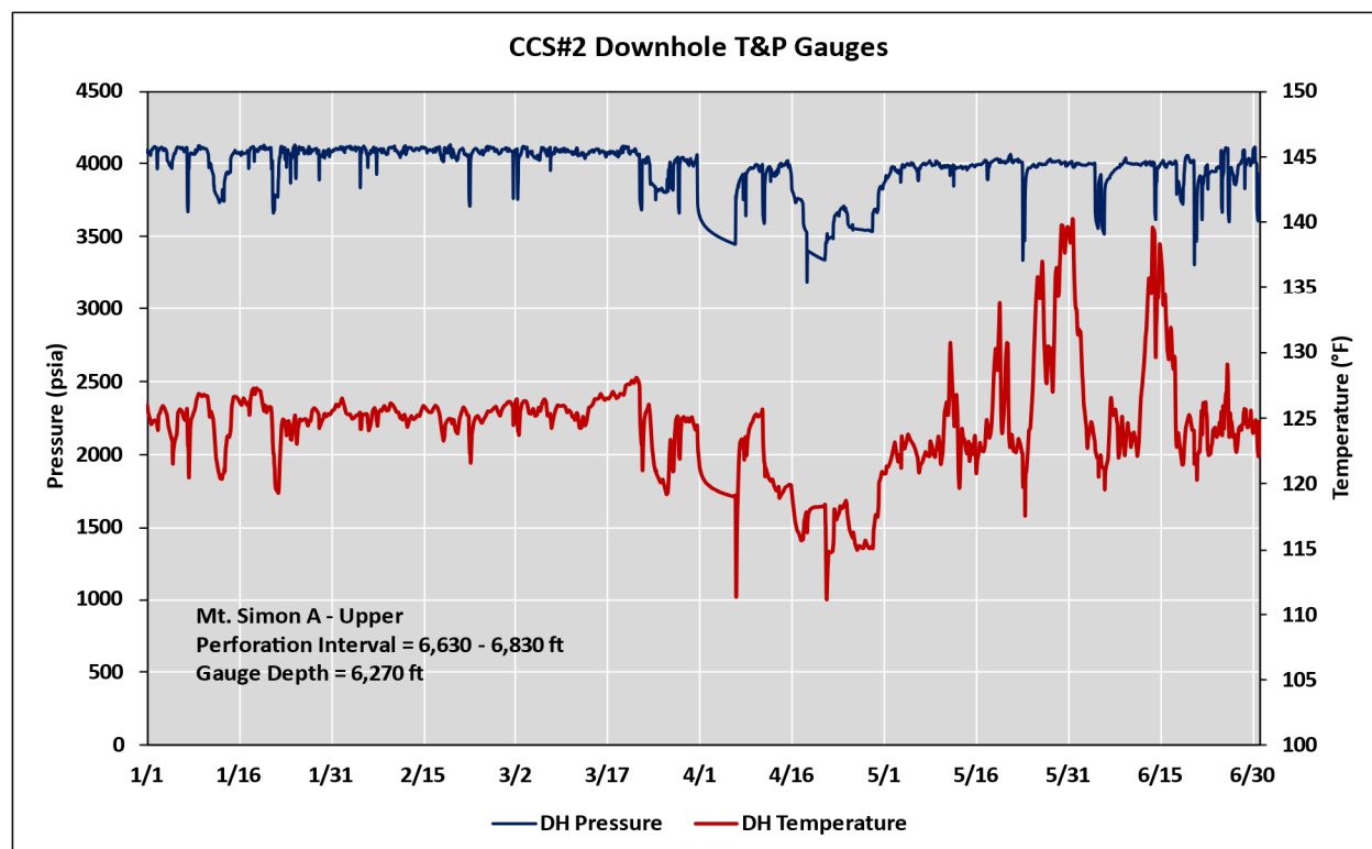
Figure 4: CCS#2 downhole temperature and pressure monitoring data for Jan-Jun 2022.
