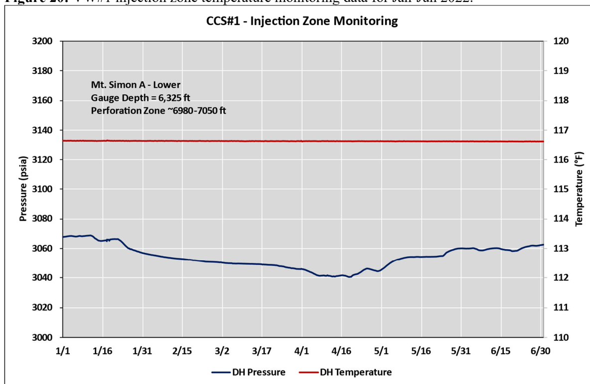
Figure 21: CCS#1 injection zone temperature & pressure monitoring data for Jan-Jun 2022.
