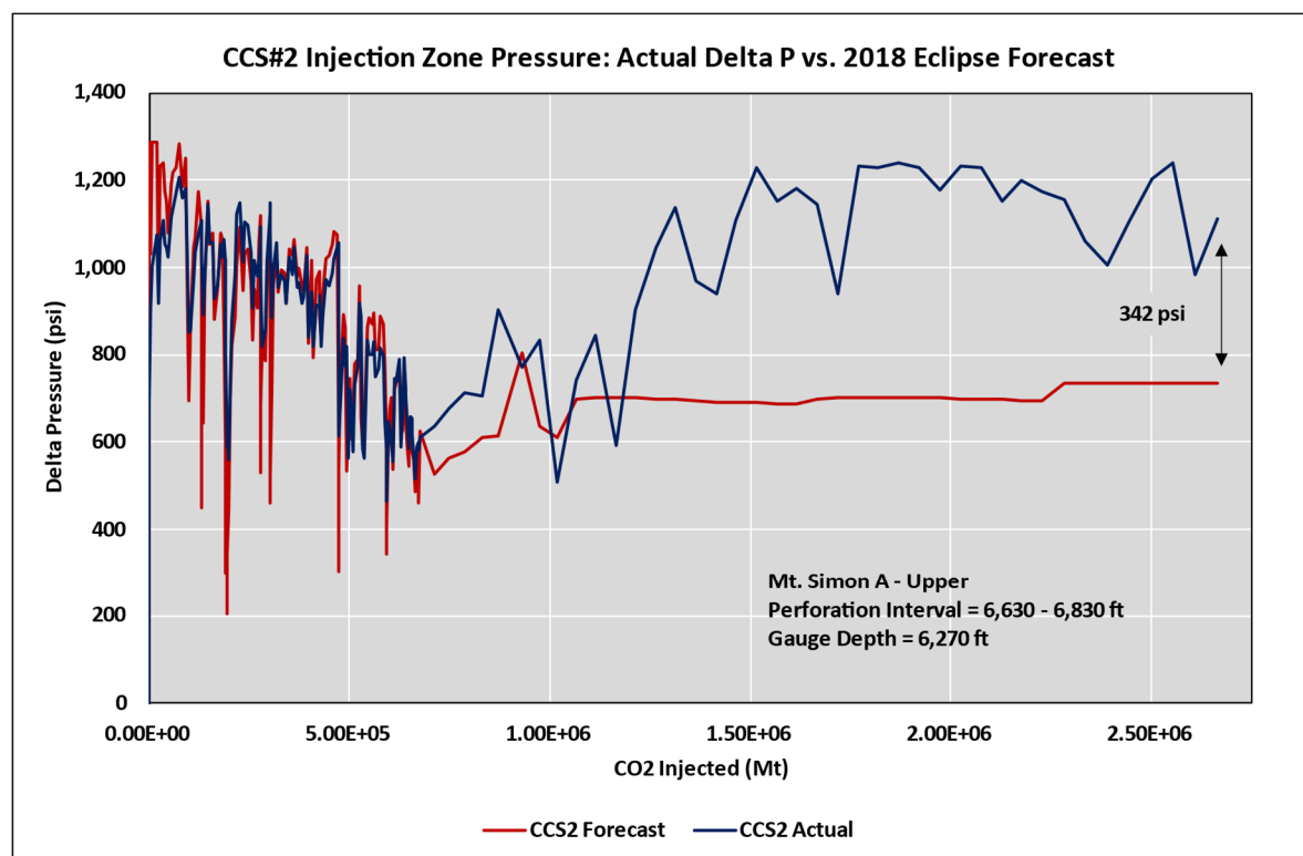
Figure 10: CCS#2 comparison of the downhole injection pressure versus the forecast pressure generated by the 2018 Eclipse reservoir model.
