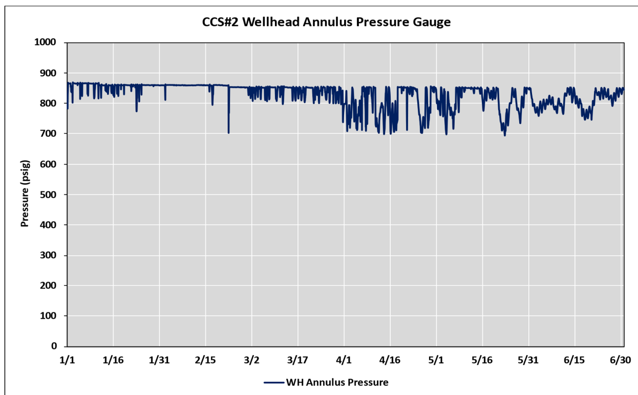
Figure 3: CCS#2 wellhead annulus pressure monitoring data for Jan-Jun 2022.
