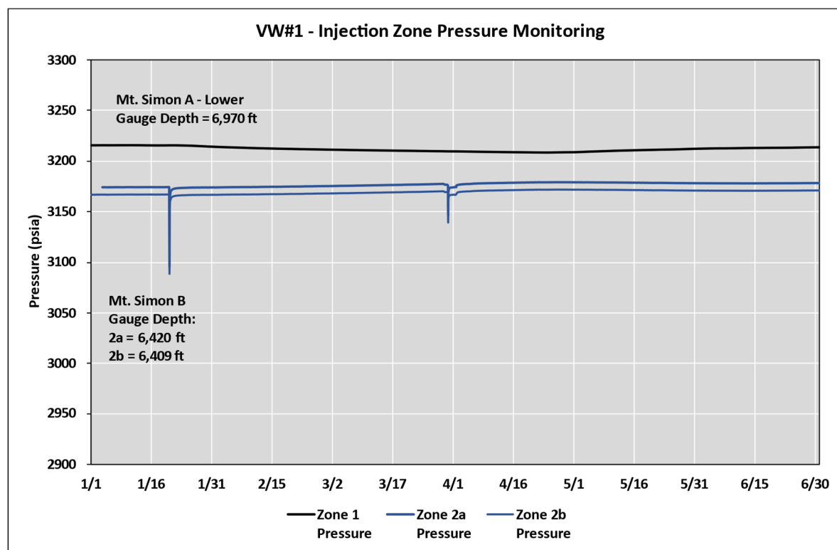
Figure 19: VW#1 injection zone pressure monitoring data for Jan-Jun 2022.
