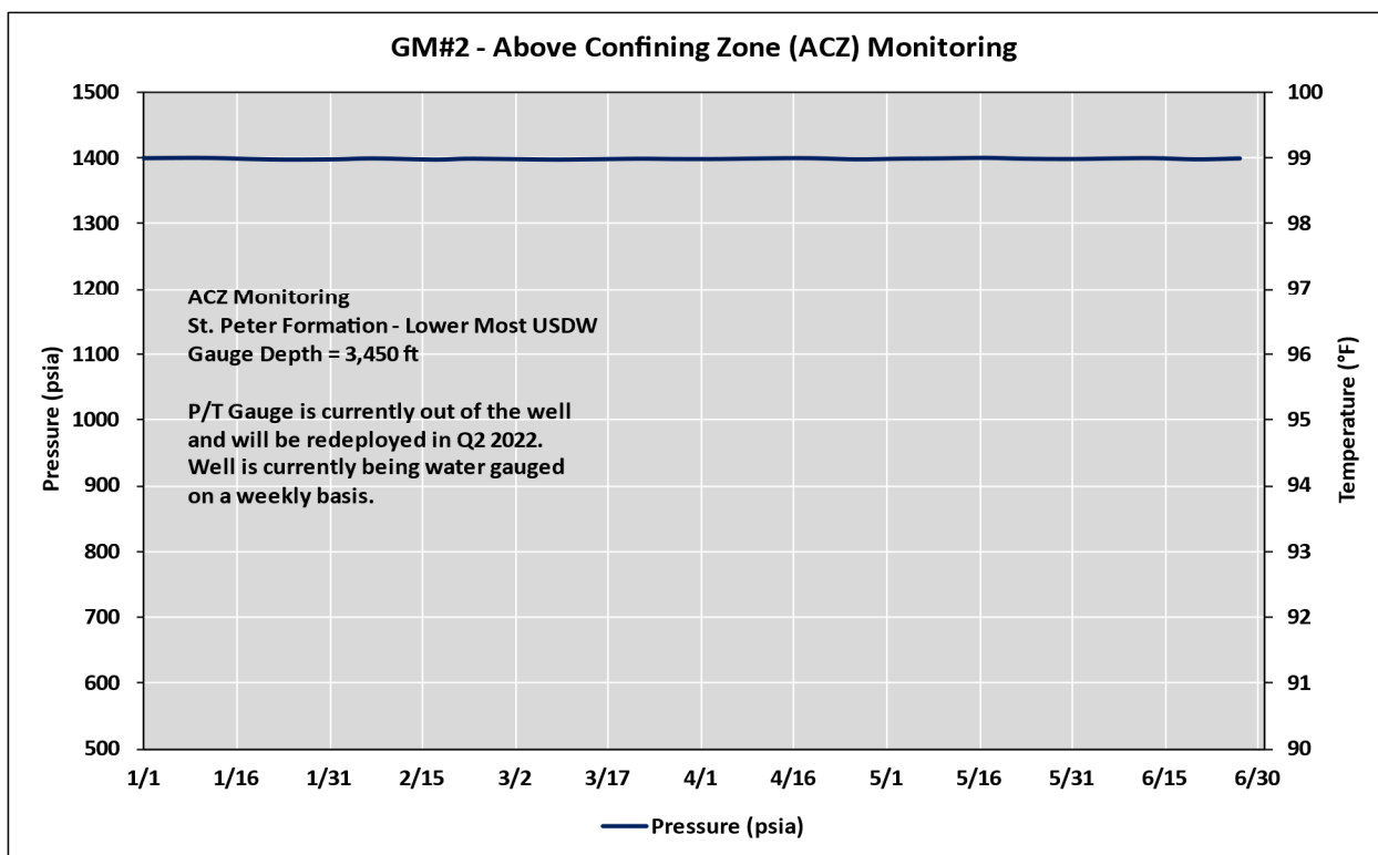
Figure 8: GM#2 ACZ monitoring of the St. Peter Formation for Jan-Jun 2022.
