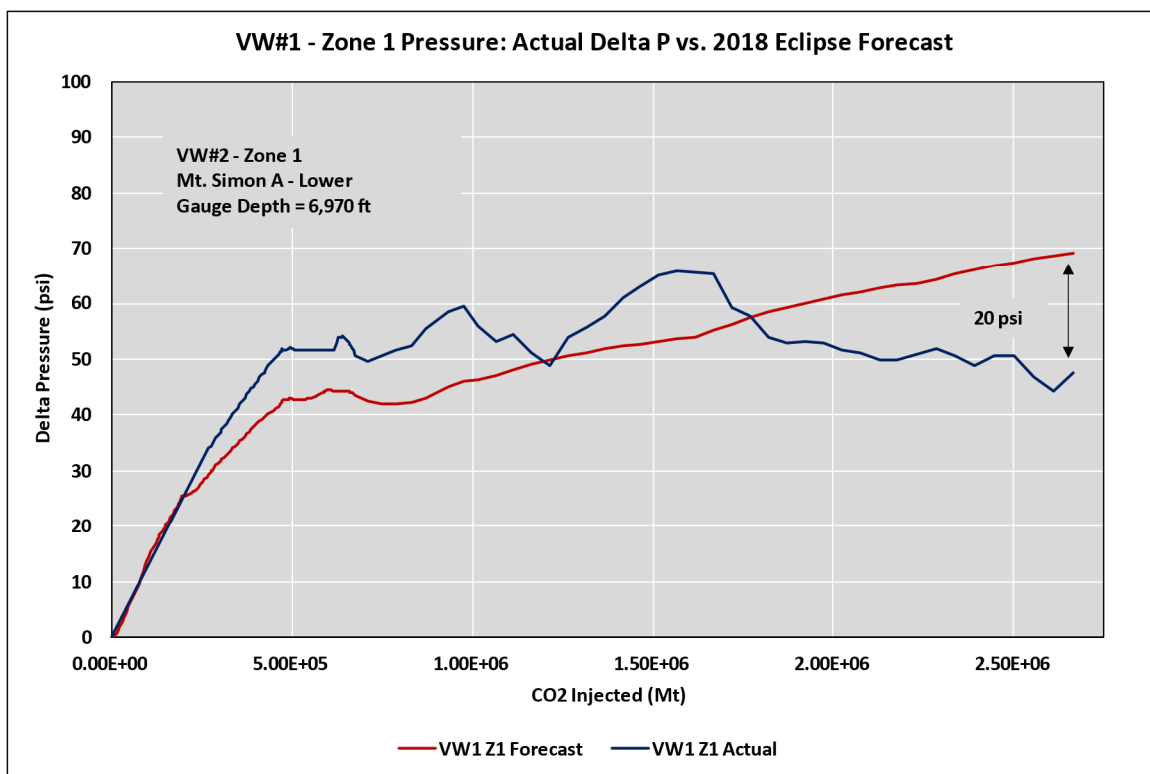
Figure 11: VW#2 Zone 1 differential pressure comparison of actual versus 2018 Eclipse forecast.
