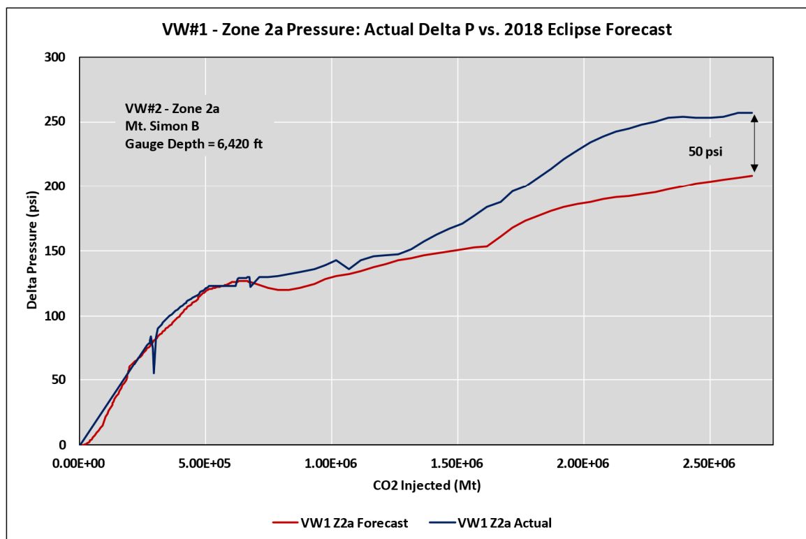
Figure 13: VW#1 Zone 2a actual reservoir differential pressure versus 2018 Eclipse forecast.
